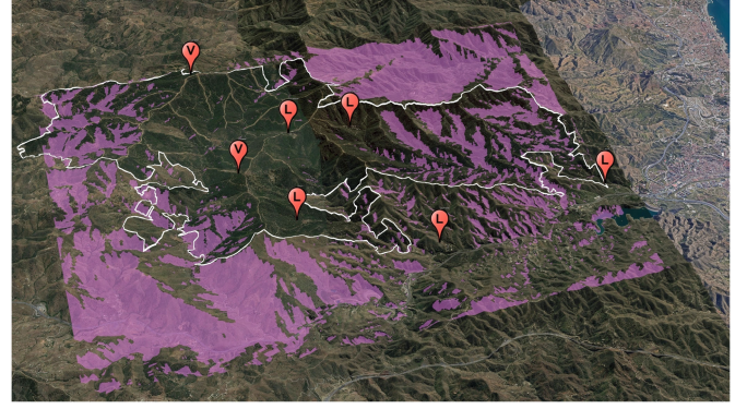
Fig. 4. CHAR map generated at the end of Stage-2. It shows the remaining uncovered area (purple layer) after having analyzed the viewshed from the initial five logistic points (L) and two points of maximum viewshed (V) in W_p . The white line represents the boundaries of the Montes de Malaga Natural Park.
