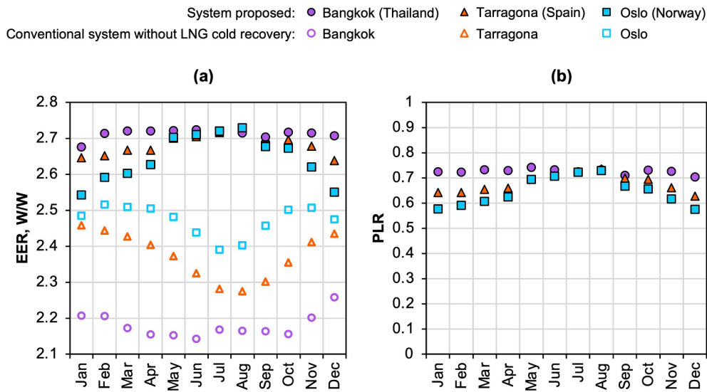
Fig. 5. Monthly average results in each location considered for a refrigeration capacity index equal to unity. (a) Energy Efficiency Ratio ( EER ) of the refrigeration machine for the system proposed in this paper and the conventional system without LNG cold utilization. (b) Part load ratio, PLR (same for both the proposed and the conventional system).
