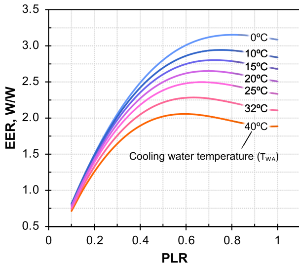
Fig. 3. Performance curves of the modelled indirect \text{NH}_3/\text{CO}_2 cascaded vapor-compression refrigeration machine for different PLRs and cooling water temperatures.
