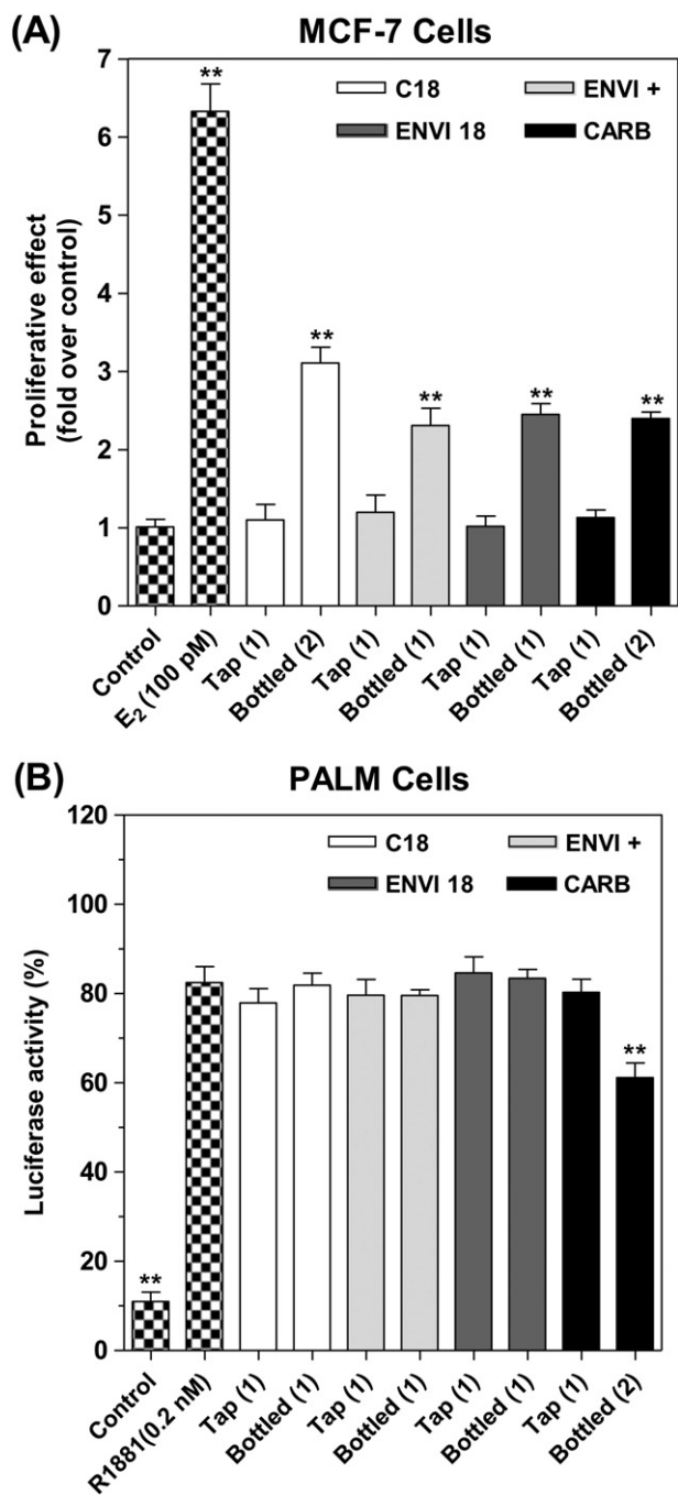
Fig. 1. Comparison of the extraction efficacy of different SPE methods to study the estrogenic and anti-androgenic activities of tap and bottled water. Panel (A): Estrogenic activity in MCF-7 cells. Results are expressed as proliferative effect (mean \pm SD of three separate experiments). ** p < 0.01 (versus hormone-free control). Panel (B): Anti-androgenic activity in PALM cells. Results are expressed as percentage of luciferase activity (mean \pm SD of three separate experiments). ** p < 0.01 (versus R1881 0.3 nM). The sample extract concentration producing the maximum effect/inhibition is reported in brackets: (1) 0.5% and (2) 0.25%.
