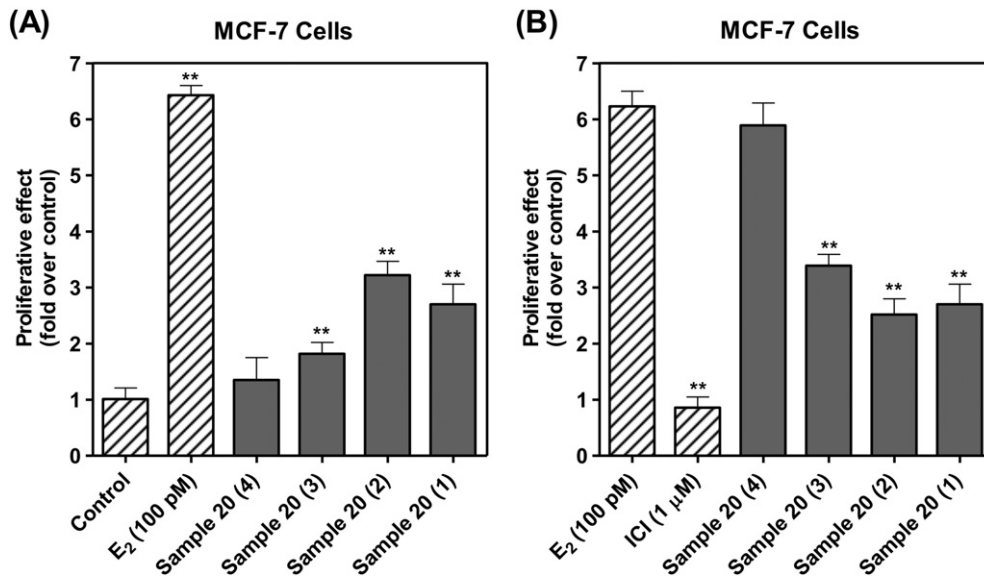
Fig. 3. Dose–response curves of bottled water sample number 20 in the E-Screen bioassay. Panel (A): Proliferative response of MCF-7 cells. Cells were incubated for 144 h at 37 °C with increasing concentrations (0.0625–0.5%) of this water sample extract. Results are expressed as proliferative effect (mean ± SD of three separate experiments). **p < 0.01 (versus hormone-free control). Panel (B): Anti-proliferative response of MCF-7 cells. Cells were treated with 100 pM E 2 in the presence of this water sample extract for 144 h at 37 °C. Results are expressed as proliferative effect (mean ± SD of three separate experiments). **p < 0.01 (versus E 2 100 pM). The sample concentration producing the (anti-)proliferative effect is reported in brackets: (1) 0.5%, (2) 0.25%, (3) 0.125% and (4) 0.0625%.
