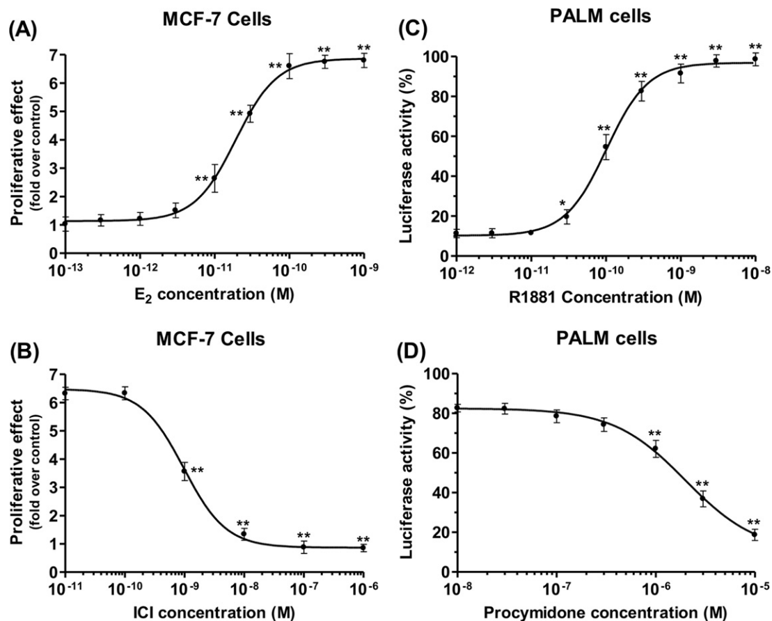
Fig. 4. Dose–response curves of E 2 and ICI on MCF-7 cells and R1881 and procymidone on PALM cells. MCF-7 cells were incubated for 144 h at 37 °C with E 2 (Panel A) or ICI in the presence of 100 pM E 2 (Panel B) at the indicated concentrations. Results are expressed as proliferative effect (mean ± SD of three separate experiments). *p < 0.05 and **p < 0.01 (versus hormone-free control or E 2 100 pM). PALM cells treated with R1881 (Panel C) or procymidone in the presence of 0.3 nM R1881 (Panel D) at the indicated concentrations for 40 h at 37 °C. Results are expressed as percentage of maximal R1881 induction (mean ± SD of three separate experiments). *p < 0.05 and **p < 0.01 (versus R1881 10 or 0.3 nM).
