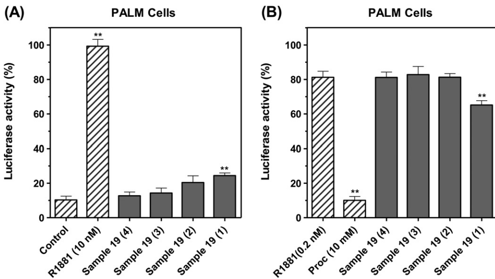
Fig. 6. Dose–response curves of bottled water sample number 19 in the PALM assay. Panel (A): Induction of luciferase activity in PALM cells, which were incubated for 40 h at 37 °C with increasing concentrations (0.0625–0.5%) of this water sample extract. Results are expressed as percentage of maximal R1881 induction (mean ± SD of three separate experiments). ** p < 0.01 (versus R1881 10 nM). Panel (B): Inhibition of luciferase activity in PALM cells, which were treated with 0.3 nM R1881 in the presence of increasing concentrations of this water sample extract for 40 h. Results are expressed as percentage of 0.3 nM R1881 induction. Values are mean ± SD of three separate experiments. ** p < 0.01 (versus R1881 0.3 nM). The sample concentration producing the induction/inhibition of luciferase activity is reported in brackets: (1) 0.5%, (2) 0.25%, (3) 0.125% and (4) 0.0625%.
