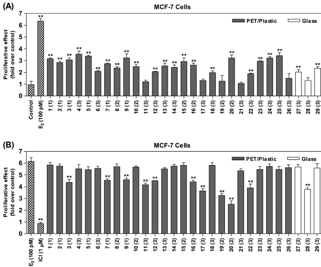
Fig. 2. Effect of bottled water samples in the E-Screen bioassay. Panel (A): Proliferative response of MCF-7 cells. Cells were incubated for 144 h at 37 °C with increasing concentrations (0.0625–0.5%) of water sample extracts of the studied products. Results are expressed as proliferative effect (mean ± SD of three separate experiments). **p < 0.01 (versus hormone-free control). Panel (B): Anti-proliferative response of MCF-7 cells. Cells were treated with 100 pM E 2 in the presence of the water sample extracts for 144 h at 37 °C. Results are expressed as proliferative effect (mean ± SD of three separate experiments). **p < 0.01 (versus E 2 100 pM). The sample concentration producing the maximum (anti-)proliferative effect is reported in brackets: (1) 0.5%, (2) 0.25% and (3) 0.125%.
