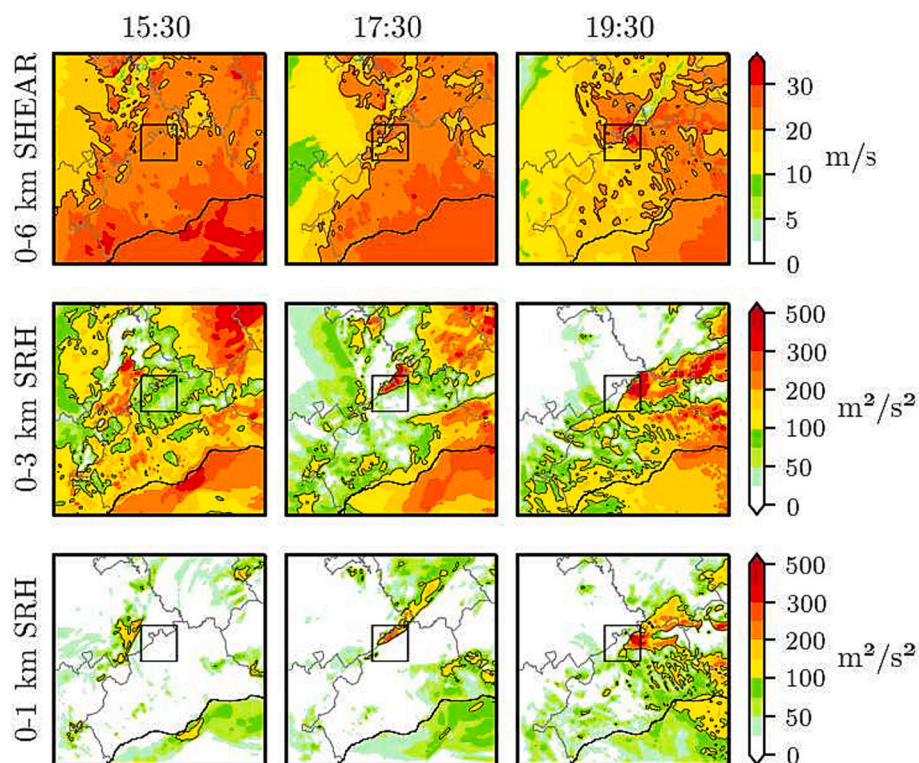
Fig. 25. Kinetic parameters for EG simulation. Deep layer (0–6 km) shear (first row), 0–3 km storm relative helicity (second row) and 0–1 km storm relative helicity (third row). Each column of maps represents one temporal instant within the most convective period of the episode in UTC. Black rectangles highlight the interest area (see Fig. 1). Thin black contour lines emphasize reference levels ( \text{SHEAR}_{06} = 20 \text{ m/s} , \text{SRH}_{03} = 100 \text{ m}^2/\text{s}^2 , \text{SRH}_{01} = 100 \text{ m}^2/\text{s}^2 ).
