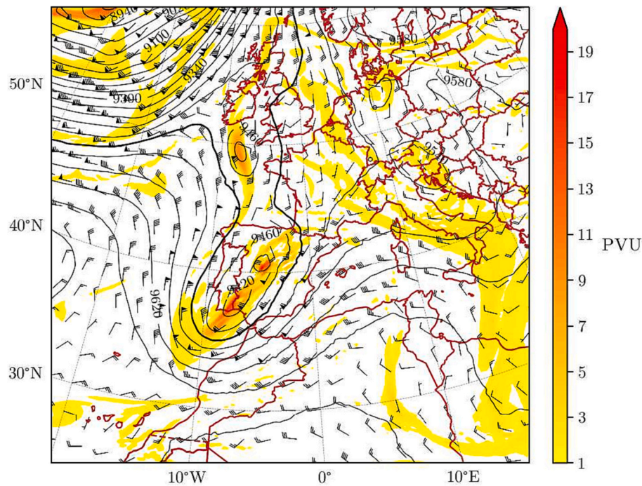
Fig. 2. Potential vorticity in PVU (shaded), geopotential height in gpm (black contours) and wind barbs at 300 hPa for HRES-IFS operational analysis. Base time: 26 August 2019 at 12:00 UTC (14:00 LT).
