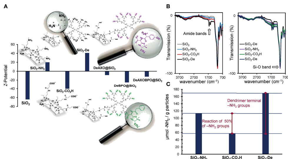
FIGURE 3 | (A) Z-potential measurements and (B) IR spectra of the functionalized particles; (C) quantification of free amino groups of SiO 2 -NH 2 , SiO 2 -CO 2 H and SiO 2 -De.
