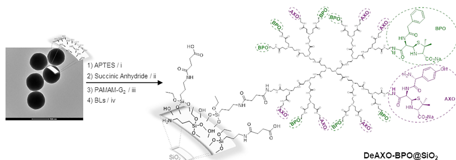
SCHEME 1 | Preparation of DeAn@SiO 2 . (i) Toluene, reflux, 12h; (ii) TEA, DMF, r.t., 12h; (iii) EDCI, NHS, DMF, r.t., 12h; (iv) Na 2 CO 3 /NaHCO 3 aqueous buffer, 4°C, 7 days. BLs correspond to amoxicillin to obtain DeAXO@SiO 2 , Benzylpenicillin to obtain DeBPO@SiO 2 or a 1:1 mixture of amoxicillin/benzylpenicillin to obtain DeAXO-BPO@SiO 2 .
