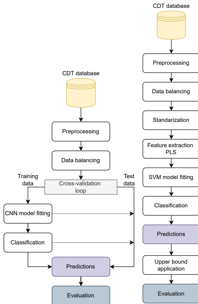
Figure 4. Flowchart of the analysed models. On the left, the flowchart associated with the deep learning-based model, which is based on cross-validation (K-fold). On the right, the flowchart associated with the machine learning-based model, based on resubstitution with upper bound correction as validation procedure.
