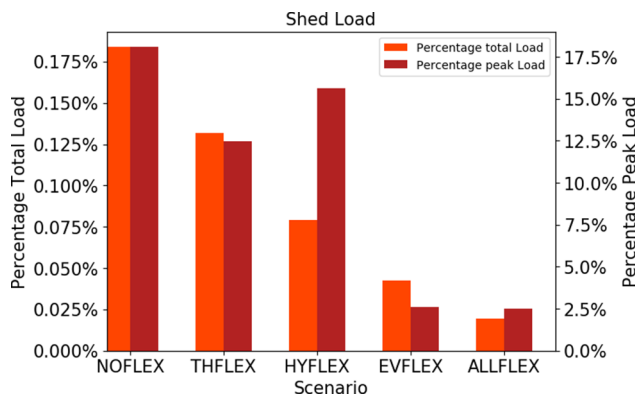
Fig. 12. Total annual and maximum hourly shed load in all scenarios as a percentage of total and peak load.
