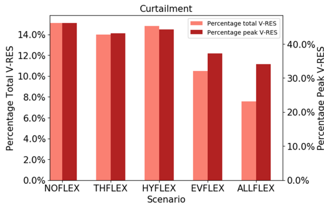
Fig. 11. Total annual and maximum aggregated hourly curtailment as percentage of total and peak generation from VRES in all scenarios.
