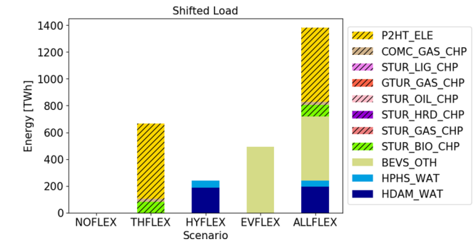
Fig. 13. Shifted load per fuel and technology type in all five scenarios. Contoured labels indicate TES storage of CHP and P2HT units.
