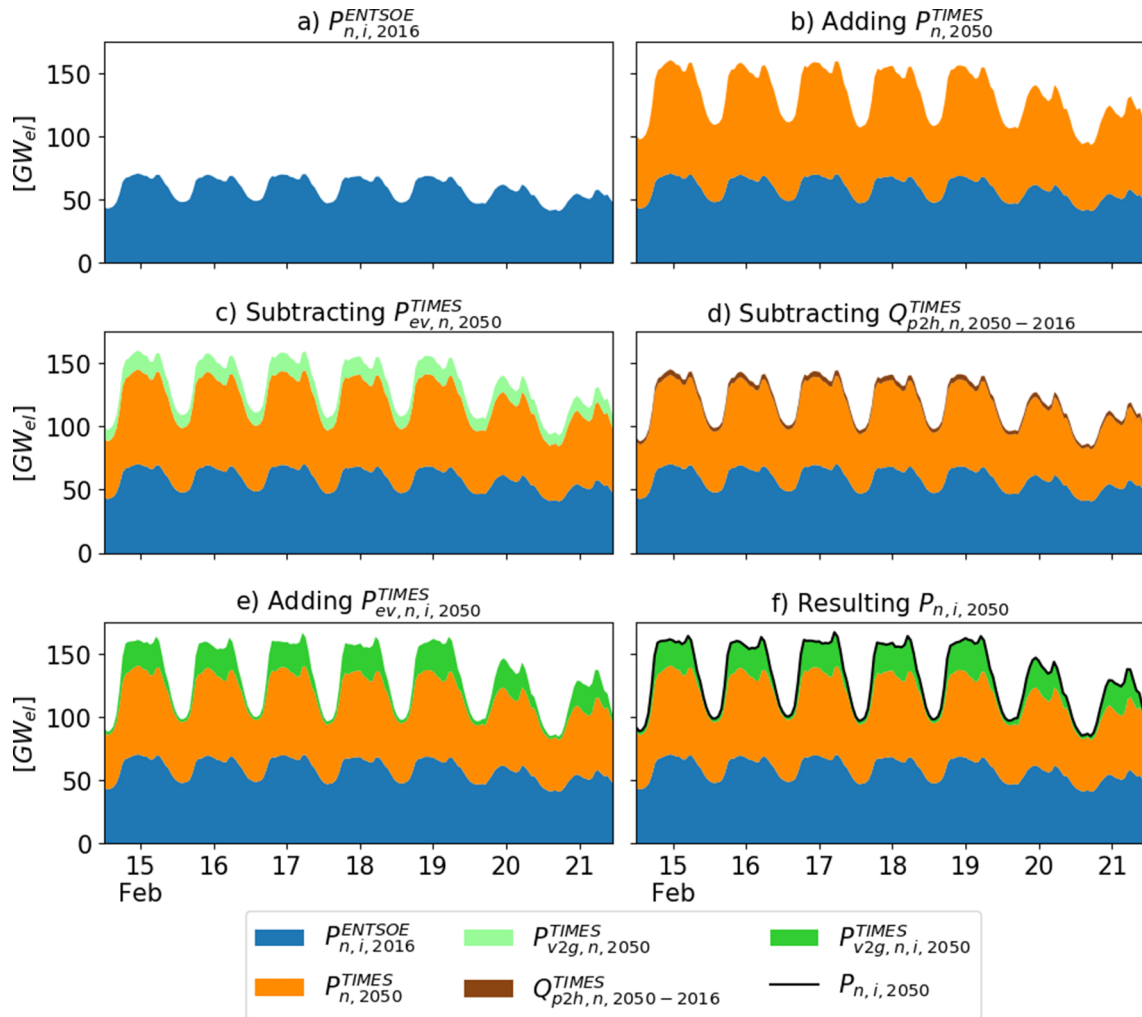
Fig. 5. Electricity demand modelling steps for one week in February. Resulting hourly demand curve is composed of ENTSO-E 2016 dataset increased to match annual demand from JRC-EU-TIMES model, adjusted electric vehicle charging demand and decreased by the P2H demand in 2016.
