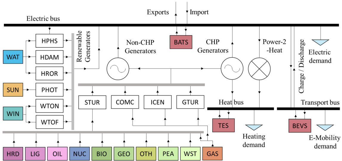
Fig. 2. System structure for a single node. Each node represents a whole country. Each object represents fuels, storage and generation technologies (boxes), buses (tick black lines) or demands (triangles). Fuels are coloured according to the Dispa-SET colour scheme.
