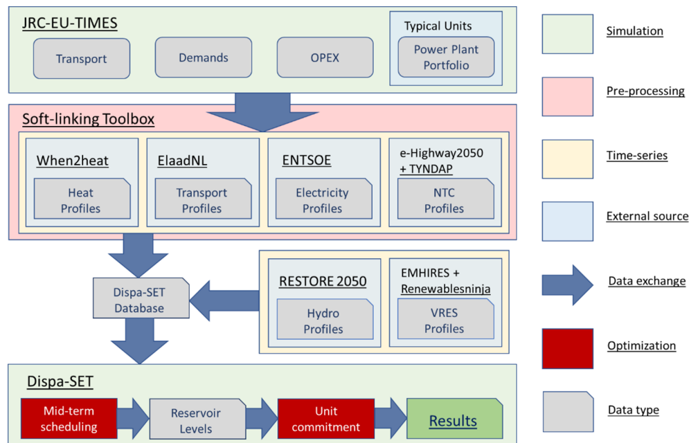
Fig. 1. Relational block-diagram between models and various data sources used with this study. JRC-EU-TIMES outputs (top) are complemented with different hourly timeseries and profiles through soft-linking toolbox (middle) and then solved with a two stage Dispa-SET model (bottom).
