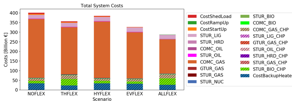
Fig. 7. Costs breakdown in all five scenarios. Variable fuel costs are presented per fuel and per technology type and other costs represent backup heaters and shed load.
