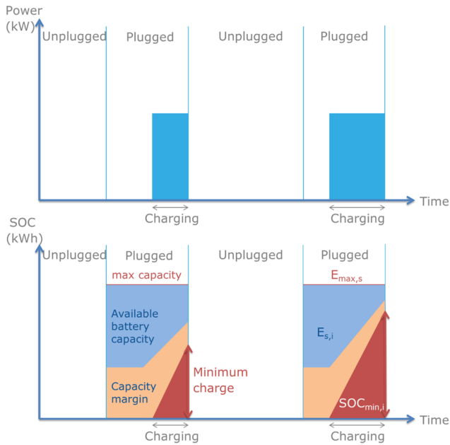
Fig. 3. Optimal charging strategy, and computation of the battery capacity of a single BEVS unit made available for the system. Battery capacity available for V2G is constrained by the minimum state of charge and corresponding capacity margin.
