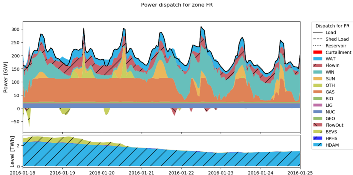
Fig. 16. Dispatch plots for France in all scenarios. Same week in January is analysed to showcase how activation of different flexibility resources has a positive impact on shed load reduction.
