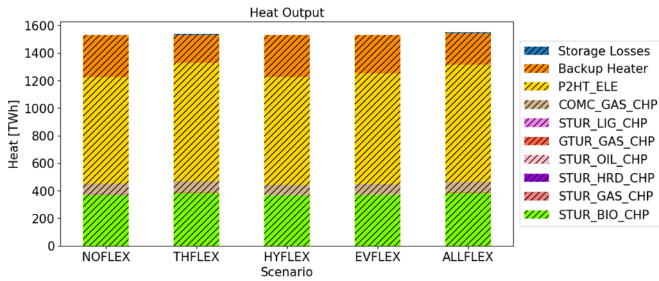
Fig. 10. Heat output per fuel and per technology type as computed in all five scenarios. Generation from backup heaters indicates either lack of heat generation capacity or expensive electricity.
