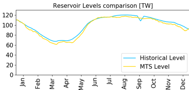
Fig. 6. Comparison of historical and computed aggregated reservoir levels. Short-term variations are optimised, and long-term seasonal variation is preserved.
