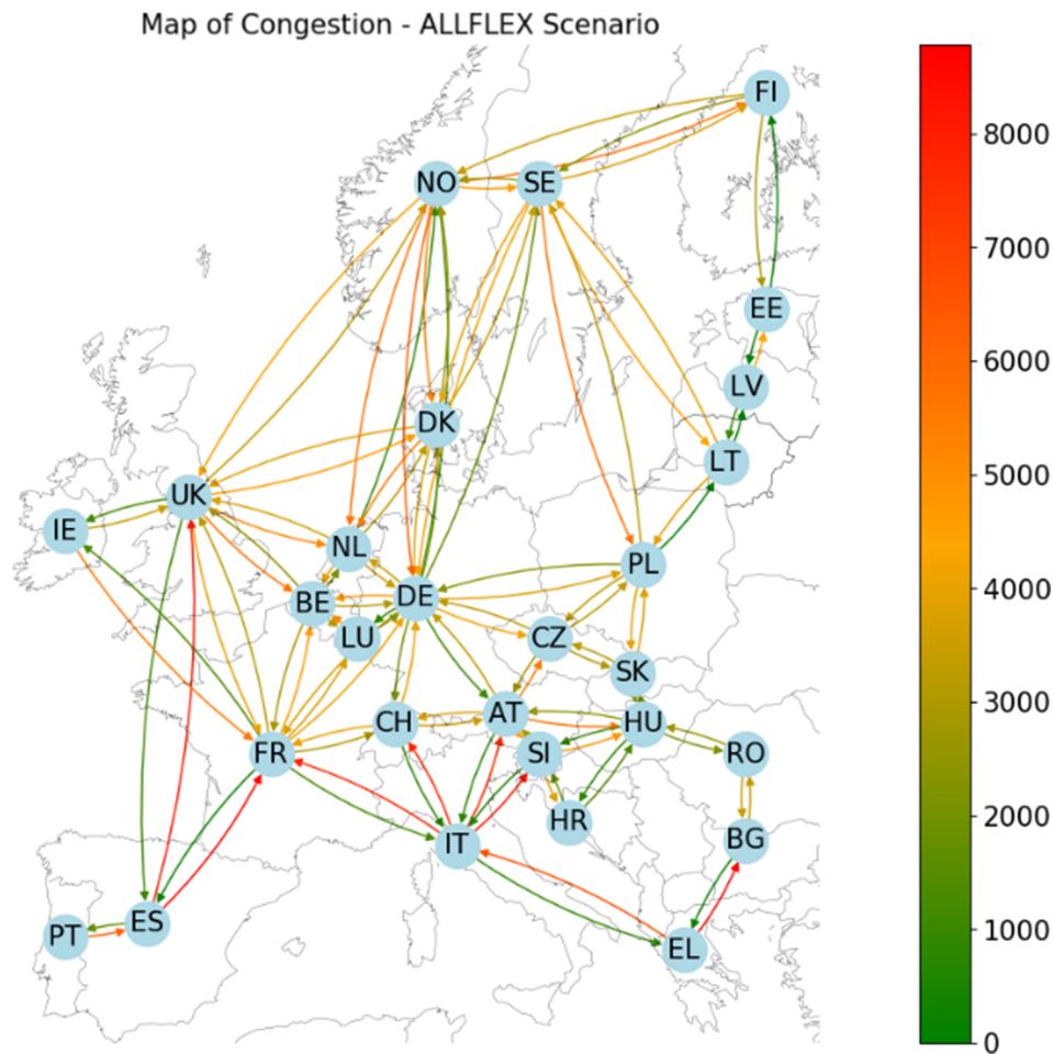
Fig. 14. Number of hours of congestion in the cross-border lines. Red lines indicate high (lack of NTC capacity) and green values low congestion (adequate NTC capacity).
