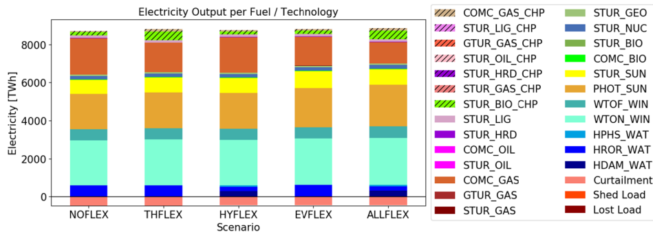
Fig. 9. Electricity output per fuel and per technology type as computed in all five scenarios. Positive values on the y-axis indicate generation, while negative values indicate demand suppression in form of shed load and lost load and RES curtailment.
