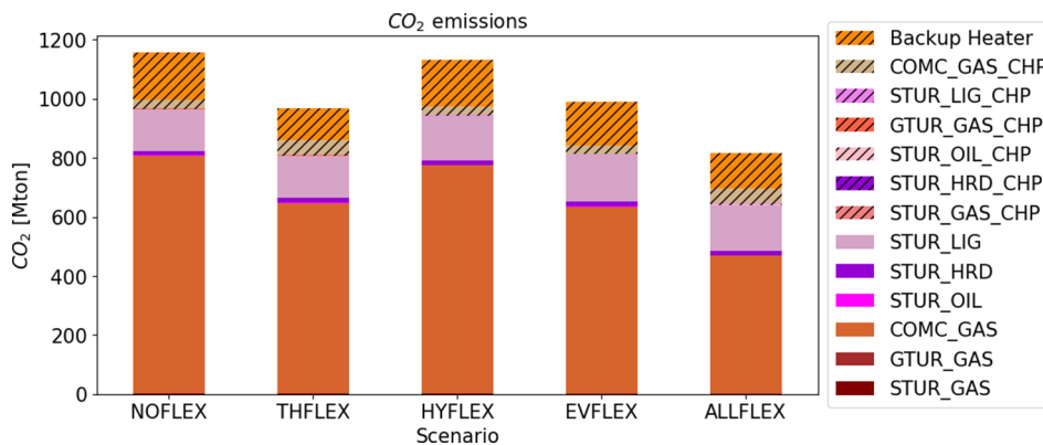
Fig. 15. Summary of CO 2 emissions grouped per fuel and per technology type in all scenarios.
