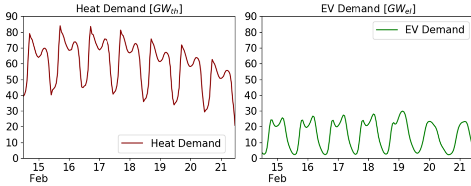
Fig. 4. Aggregated EU-wide demand breakdown of heating and transport sectors for one week in February
