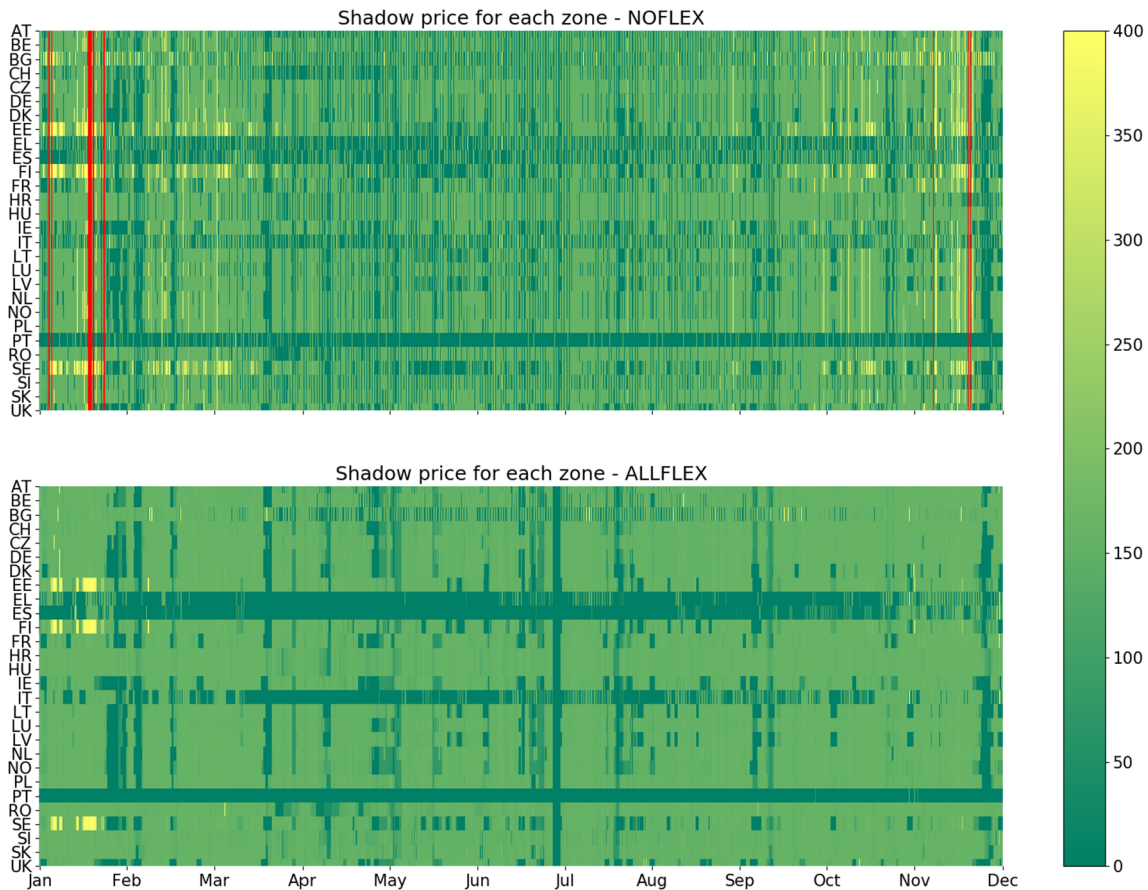
Fig. 8. Heat map of computed shadow prices on hourly scale in each of the 28 countries. Values on the legend indicate shadow prices in EUR/MWh, green colours represent variable dispatch costs, yellow stands for shed load and red indicates disregarded time periods where lost load, resulting in infeasible solutions, is being computed.
