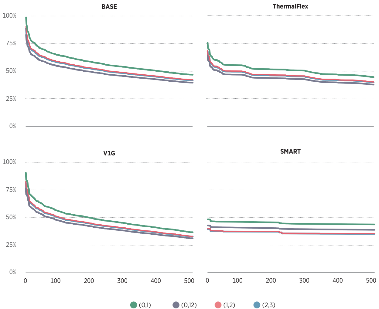
⚡ FIGURE 20 | Load duration curves of the use of lines (ratio of actual capacity to nominal capacity) for the most demanded lines in the grid
