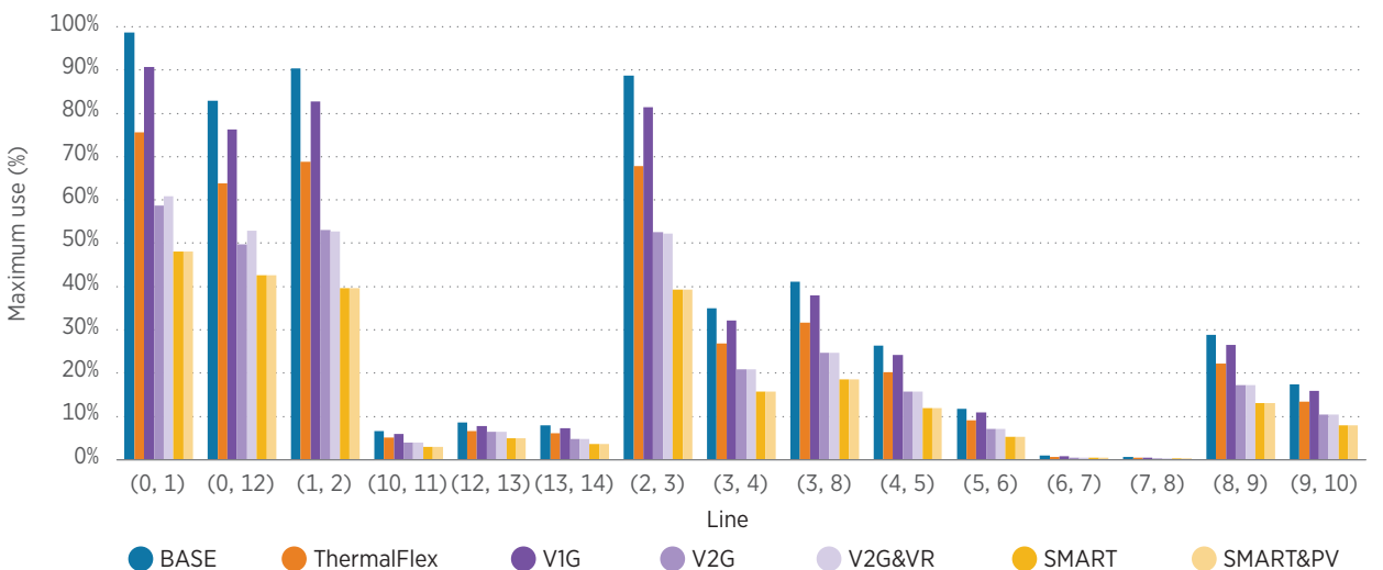
FIGURE 18 | Maximum use of lines capacity
