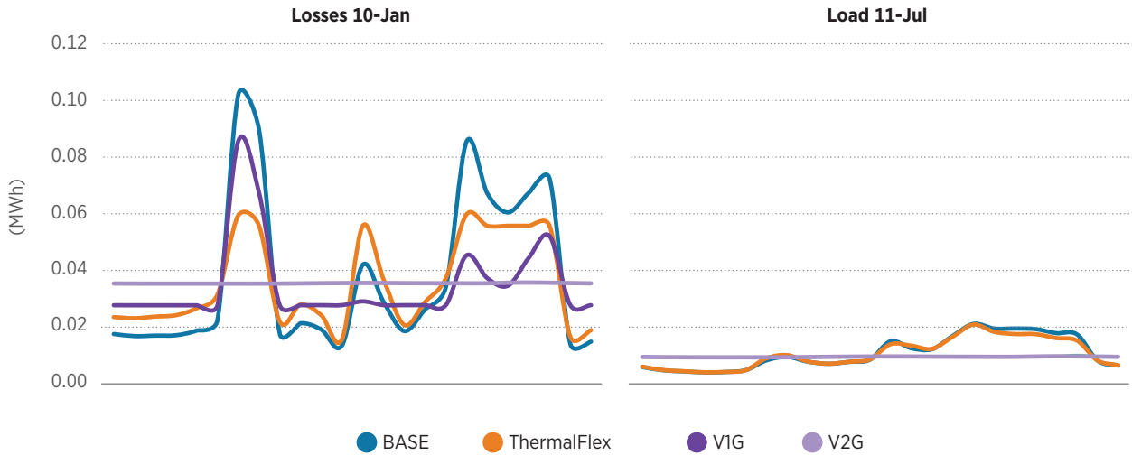
FIGURE 12 | Total energy losses in the representative winter day (left) and summer day (right)
