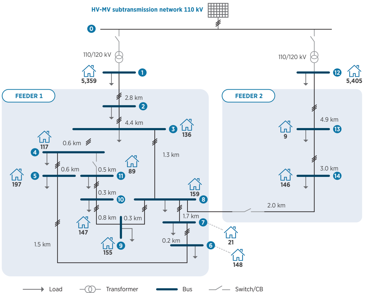
FIGURE 2 | CIGRE medium-voltage network
