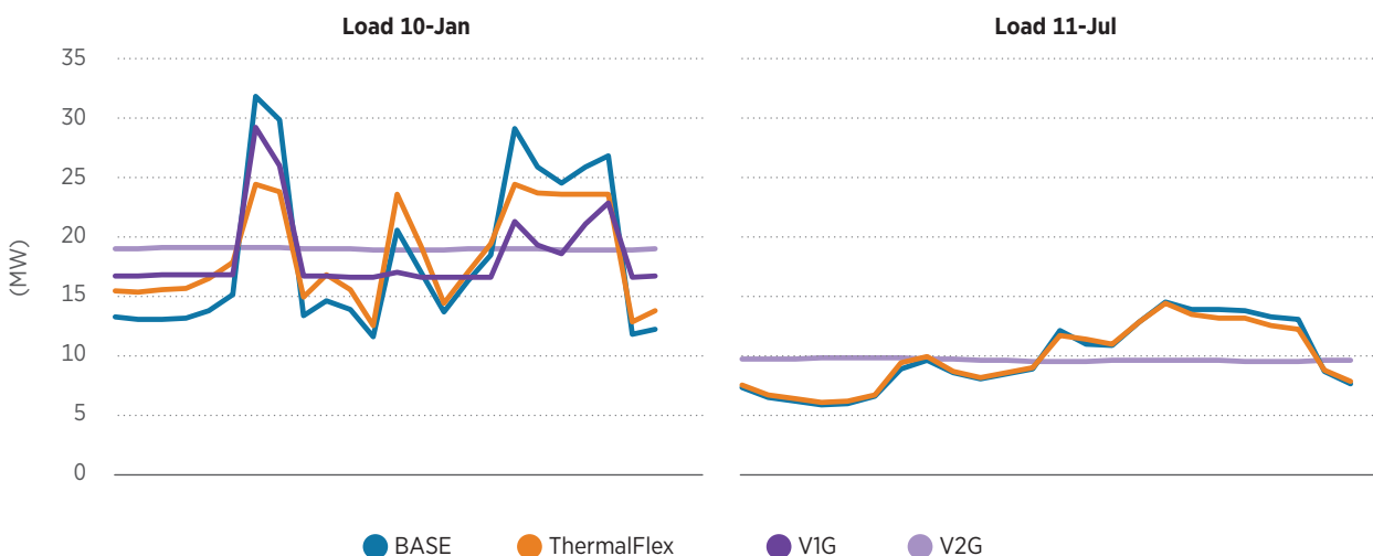
⚡ FIGURE 8 | Total energy demand in the representative winter day (left) and summer day (right)
