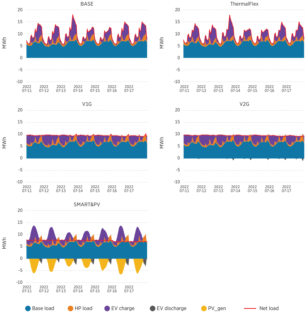
FIGURE 10 | Weekly demand dispatch – non-winter
