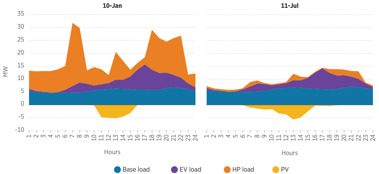
FIGURE 5 | Daily energy demand profile for a winter day (left) and summer day (right)
