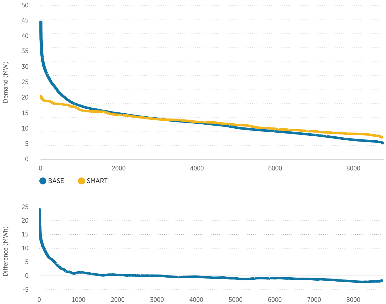
FIGURE 22 | Load duration curve of the demand in the BASE and SMART scenarios (upper) and difference in demand between the two scenarios
