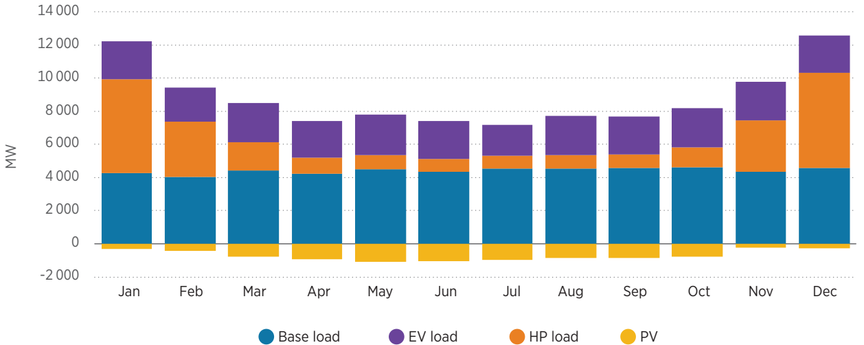
FIGURE 6 | Aggregated monthly energy demand profiles
