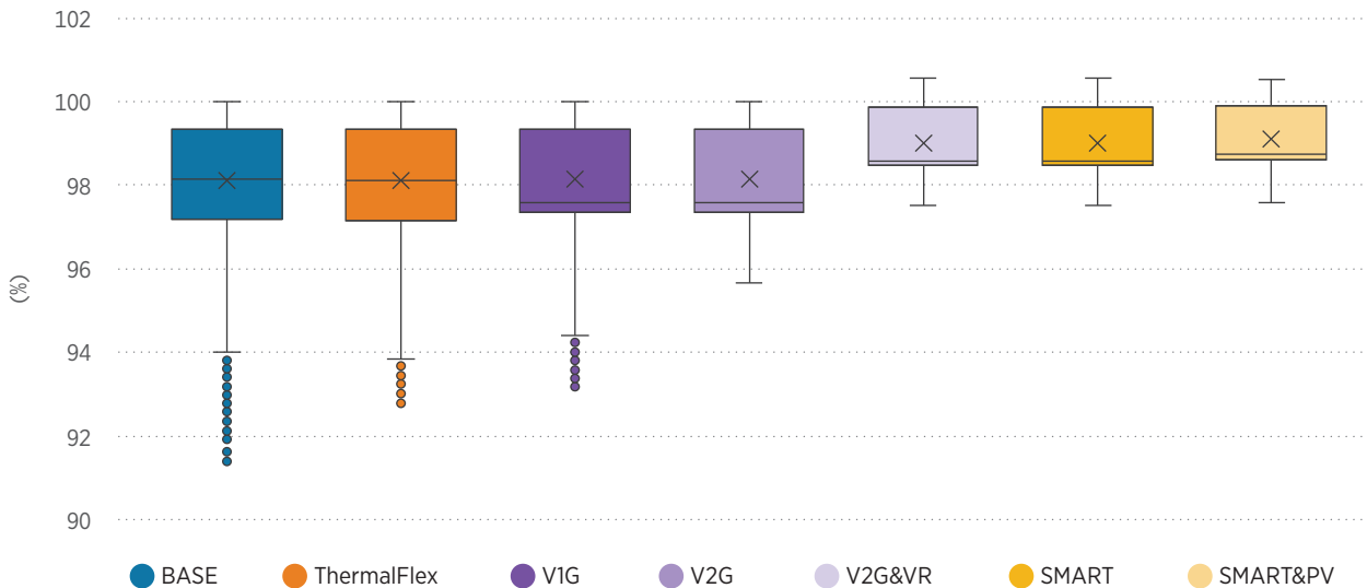
FIGURE 14 | Voltage magnitude - non-winter
