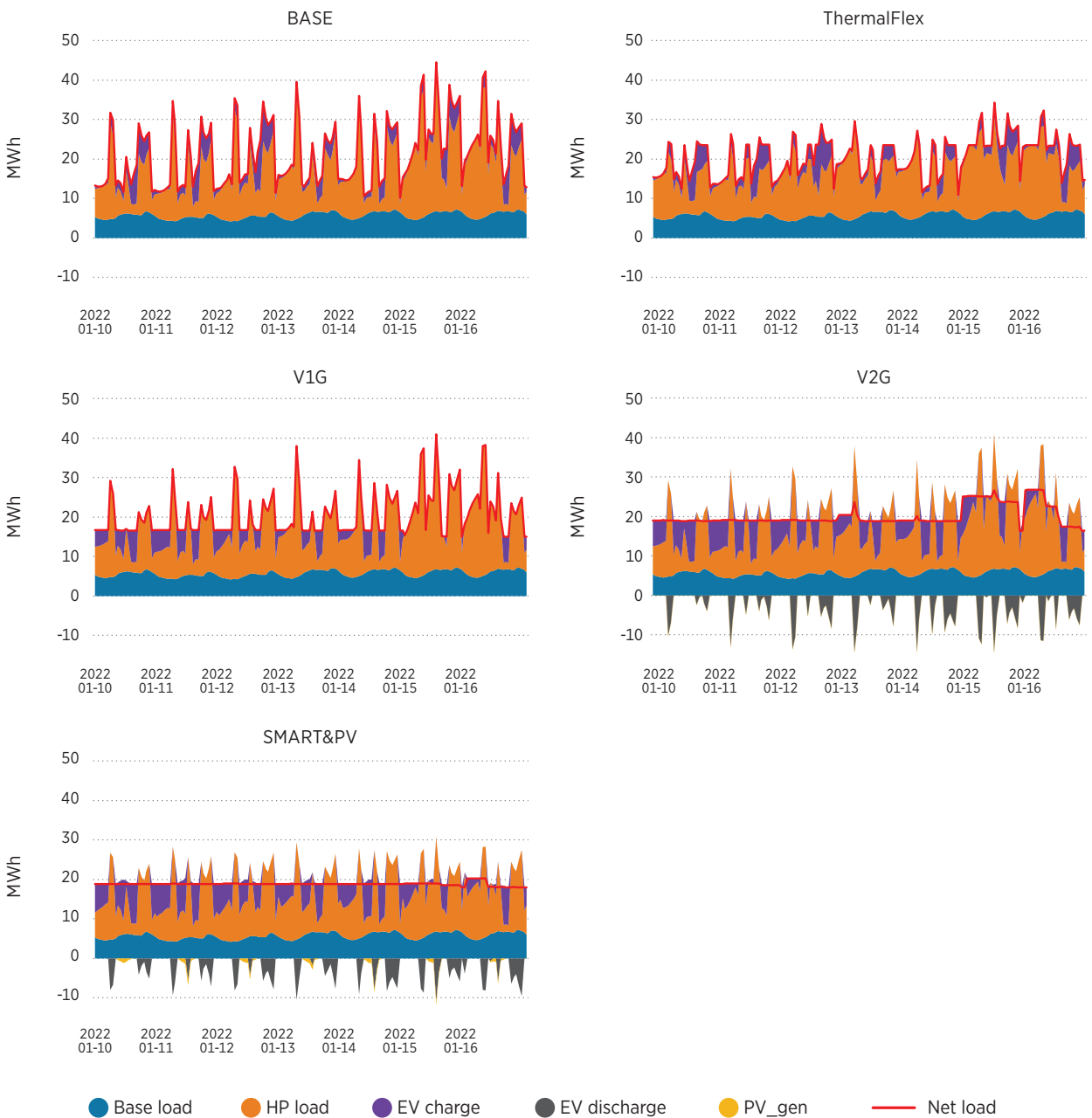
FIGURE 9 | Weekly demand dispatch – winter
