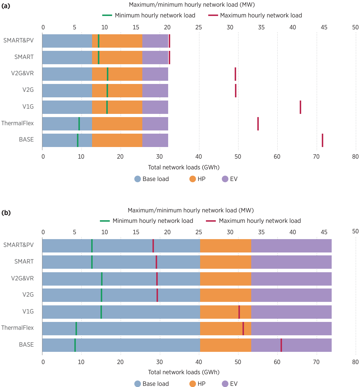
FIGURE 7 | Total, maximum and minimum energy demand – winter (a) and non-winter (b)
