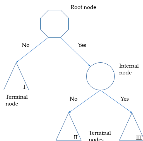
Figure 1. Decision Tree Classifier (for learning purpose).
