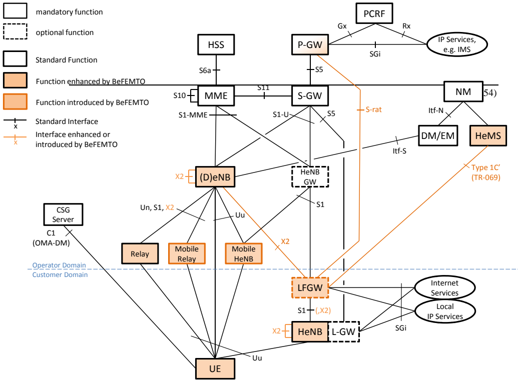
(b) BeFEMTO EPS Architecture [103].
