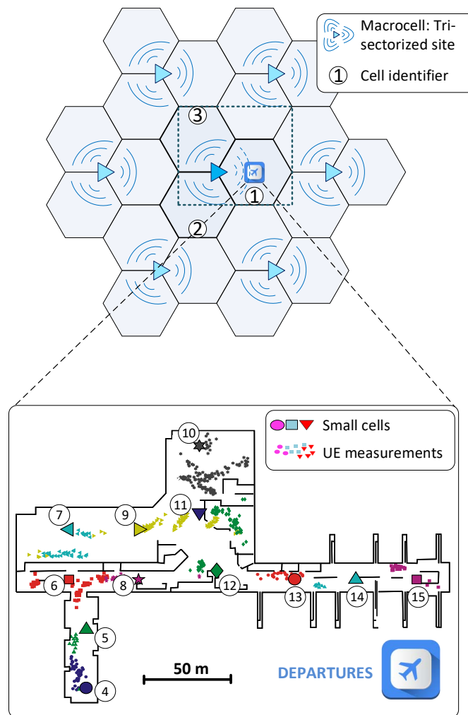
Figure A.2: Simulated airport scenario.
