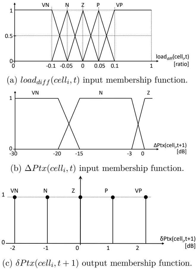
Figure 4.6: FLC membership functions.
