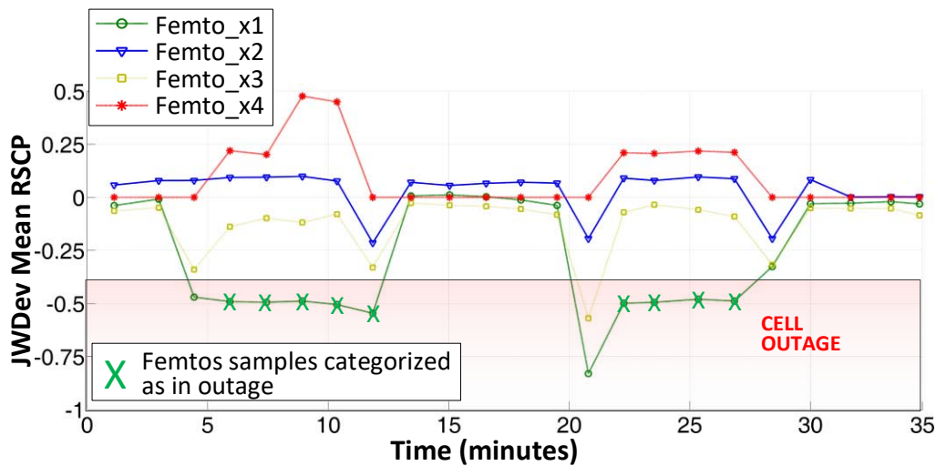
Figure 5.6: Joint Weighted Deviation Mean RSCP.
