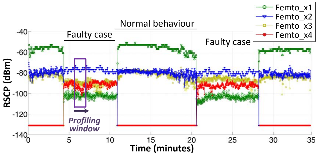
Figure 5.3: Evolution of indicator RSCP gathered by one terminal.
