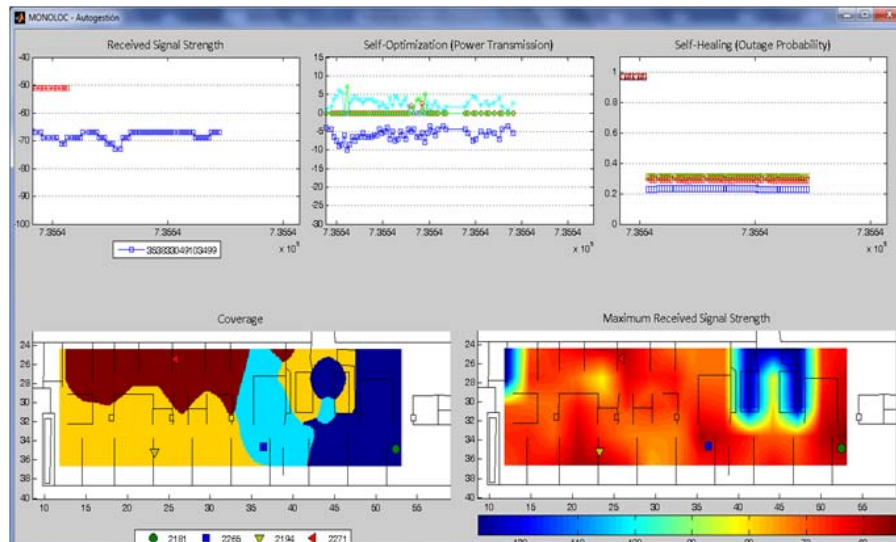
Figure A.5: Testbed SON monitoring GUI.
