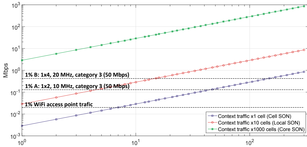
Figure 4.9: Signaling costs and baseline user plane cell throughput for LTE small cells.
