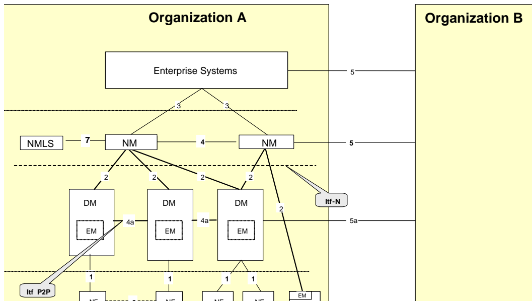
Figure 2.7: Management reference model [52].
