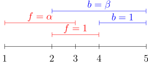
Figure 3: Example of fuzzy interval model and algebra. In non-shown intervals all propositional letters are evaluated to 0.
