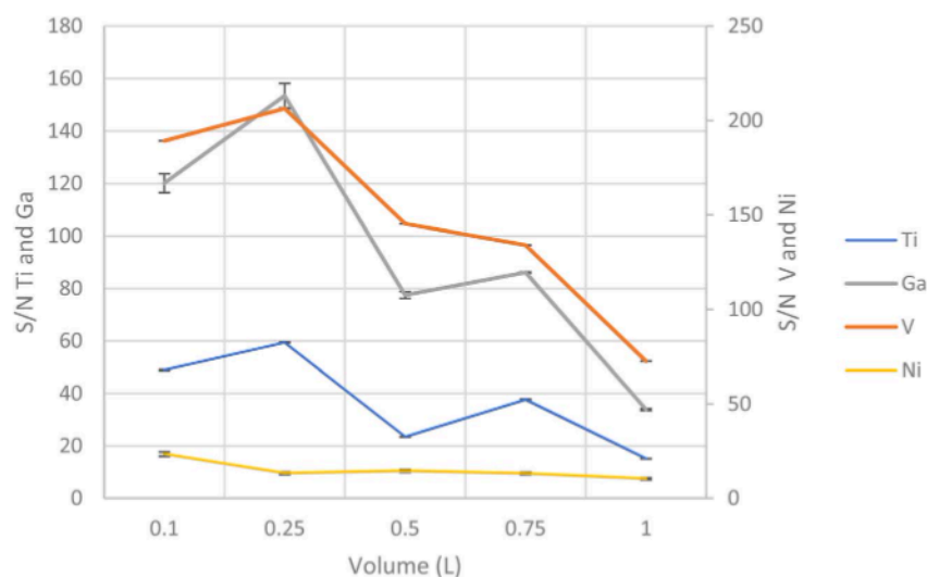
Fig. 5 Study of maximum sample volume to a quantitative analysis.
