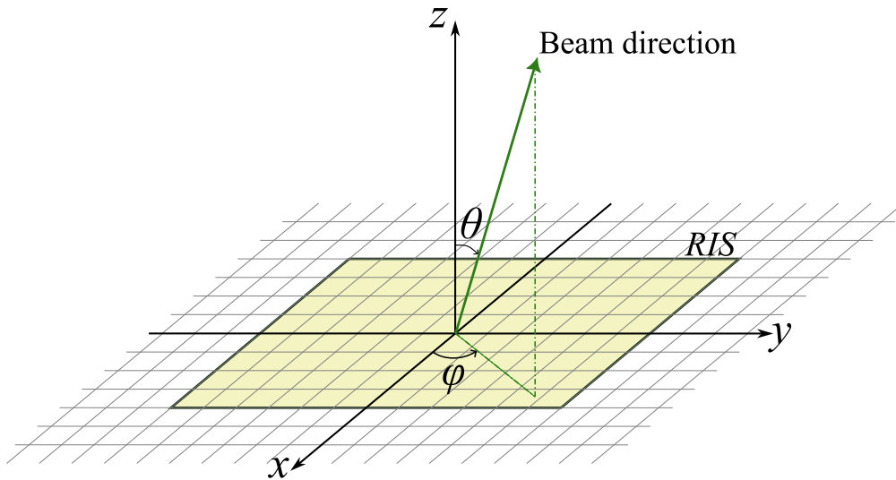
Fig. 1. Representation of the angles \phi and \theta characterizing each beam shaped by the reconfigurable intelligent surface (RIS).
