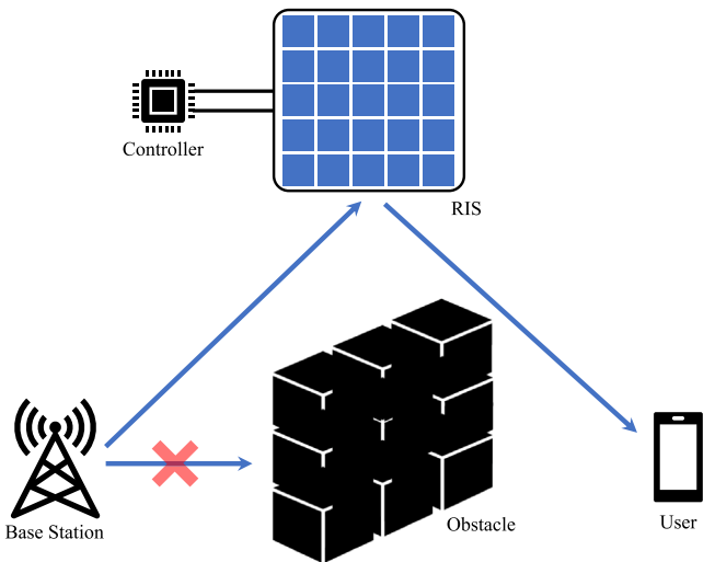
Fig. 2. A RIS being used to redirect a beam from a base station to a user, i.e., creating a virtual Line Of Sight (LOS).
