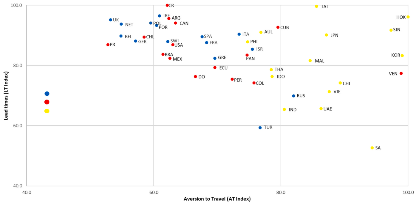
Fig. 3. Joint positioning matrix according to the indices: Aversion to Travel (AT Index) and Lead Times (LT Index).
