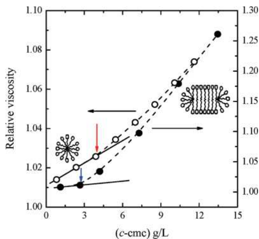
Figure 6. Relative viscosity of OTG micellar solutions in (b) water and (O) 3 M urea.
