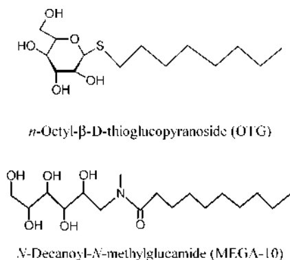
Figure 1. Molecular structures of the surfactants studied in the present investigation.
