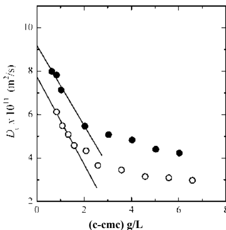
Figure 5. Apparent diffusion coefficients D_e vs surfactant concentration for OTG in urea solutions: (O) 1 M and (b) 2 M. Solid lines are the best fit of data to eq 5.
