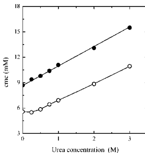
Figure 3. Effect of the urea concentration on the cmc of the surfactants: (b) OTG and (O) MEGA-10.
