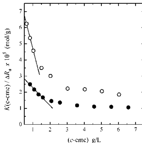
Figure 7. Debye plots for OTG micellar solutions in urea solutions: (b) 1 M and (O) 2 M.
