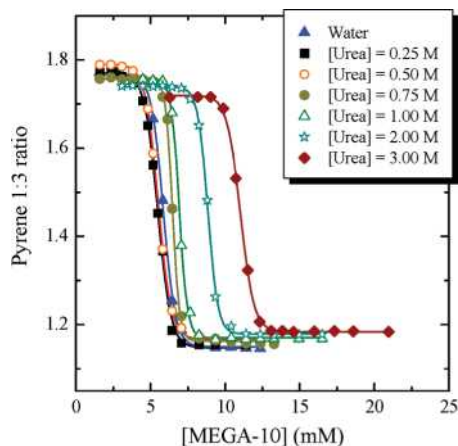
Figure 2. Plots of pyrene 1:3 ratio vs the total concentration of MEGA-10 in water and at different urea concentrations.
