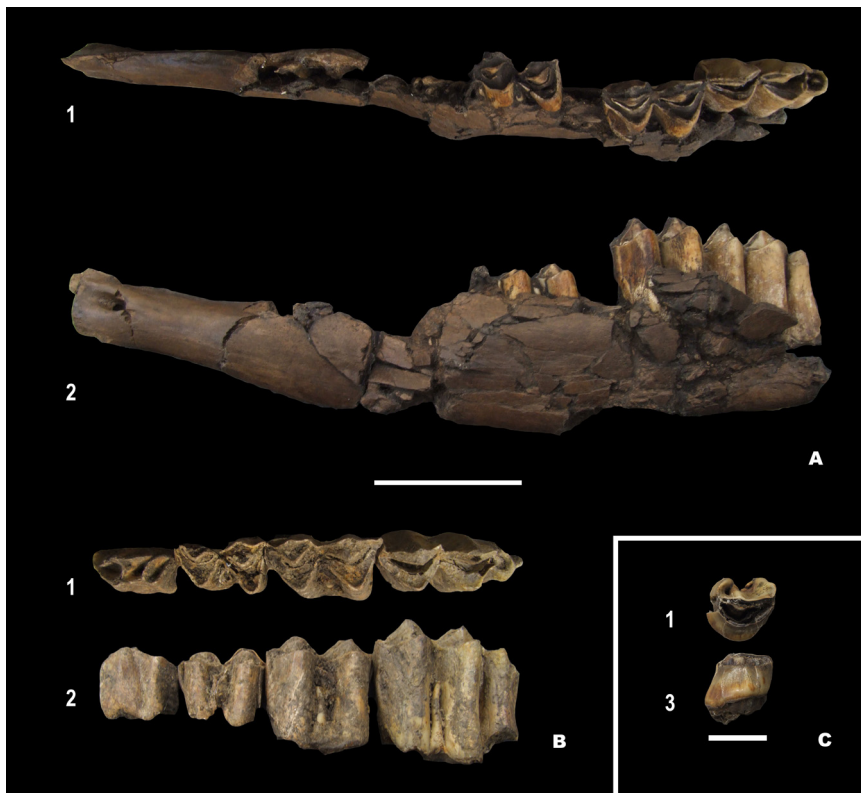
Fig. 8. Alephis sp. remains. A. Left mandible BA-1 2015 N9 No. 13. B. Left mandible BA-1 2001 O10 No. 7. C. Left P3/BA-1 2015 O11 No. 22. 1: occlusal view, 2: labial view; 3: lingual view. Scale bars represent 5 cm (A and B) and 2 cm (C).
