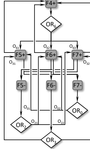
Fig. 7: Example or-overlap.
