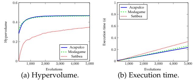
Fig. 8: Results for Mobile Media feature model.
