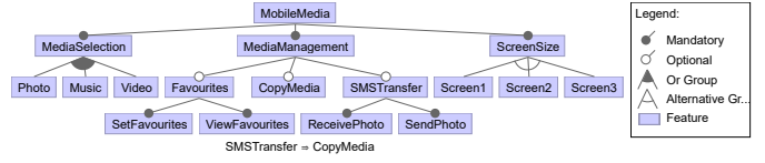
Fig. 1: Example feature diagram of Mobile Media.
