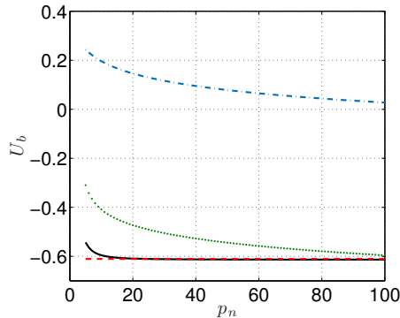
Figure 2: Comparison of the cut-off formula (dashed red line) with the approximate formula (2.5) (solid black line). Binormal component of the induced velocity versus the number p_n of segments by turn for an helix of circulation \Gamma = 1 , pitch h = 1 , radius R = 1 , and core size a = 0.05 . The two contributions \mathbf{U}^{loc} and \mathbf{U}^{seg} are also indicated in dash-dot and dotted lines, respectively.
