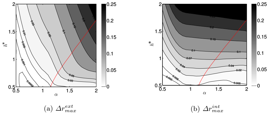
Figure 10: Maximum deformation contours in the (\alpha, h^*) plane for R^* = 0.5 , \varepsilon = 0.03 , \kappa = 1 , N = 1 . The thick solid line corresponds to the line \Delta r_{max}^{int} = \Delta r_{max}^{ext} .
