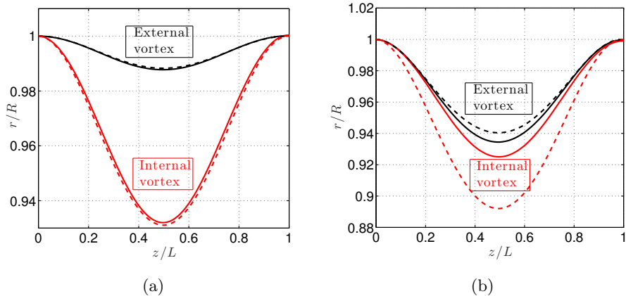
Figure 6: Radial position of the internal and external vortices for a single counter-rotating helical pair for (a) R^* = 0.5 , \kappa = 1 , h^* = 1 , \alpha = 0.9 and \varepsilon = 0.03 (b) R^* = 0.5 , \kappa = 1 , h^* = 1 , \alpha = 1.4 and \varepsilon = 0.03 . Solid line: numerical solution. Dashed line: first order approximation.
