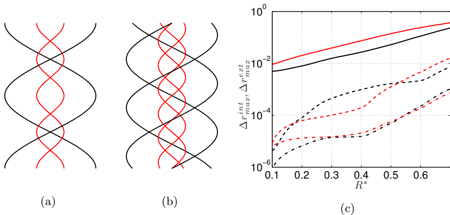
Figure 9: Representation of 2 vortex pairs (a) and 3 vortex pairs (b) for h^* = 1 , R^* = 0.4 , \varepsilon = 0.05 , \alpha = 2 , \kappa = 1 . (c): Maximum deformation \Delta r_{max}^{int} (red) and \Delta r_{max}^{ext} (black) versus R^* for 1 vortex pair (solid lines), 2 vortex pairs (dashed lines), 3 vortex pairs (dash-dot lines). h^* = 1 , \alpha = 1.5 , \kappa = 1 and \varepsilon = 0.05 .
