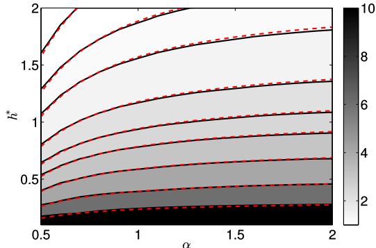
Figure 19: Contours of mass axial flow rate M (normalized by \rho N T R_{ext} ) in the (\alpha, h^*) plane for R^* = 0.5 , \varepsilon = 0.03 , N = 1 and \kappa = 1 . Contours correspond from top to bottom to \{1, 1.25, 1.5, 2, 2.5, 3, 4, 6, 10\} . Solid lines: M ; red dashed lines: M^H .
