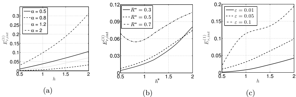
Figure 7: First order approximation error E_{r,int}^{(1)} for a single vortex pair ( N = \kappa = 1 ). (a): R^* = 0.5 and \varepsilon = 0.03 ; (b): \alpha = 1.2 and \varepsilon = 0.03 ; (c): R^* = 0.5 and \alpha = 1.2
