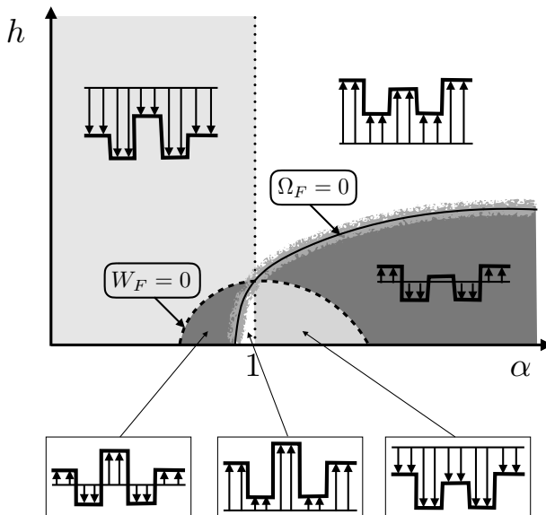
Figure 21: Diagram of the different rotor flow regimes. White regions: windmill brake regime or wind turbine regime (both vortices are going upwards as the external wind). Light gray regions: ascending regime (both vortices are going downwards as the external wind). Dark gray regions: slow descending regime and vortex ring state (both vortices are going downwards while the external wind is going upwards). Close to the line \Omega_F = 0 , there exist a small region where one vortex is going upwards while the other is going downwards: such a solution cannot describe the (far) wake of a rotor.
