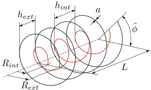
Figure 4: Configuration of two undeformed co-axial helical vortices. Here both helices have the same orientation: \kappa = 1 .
