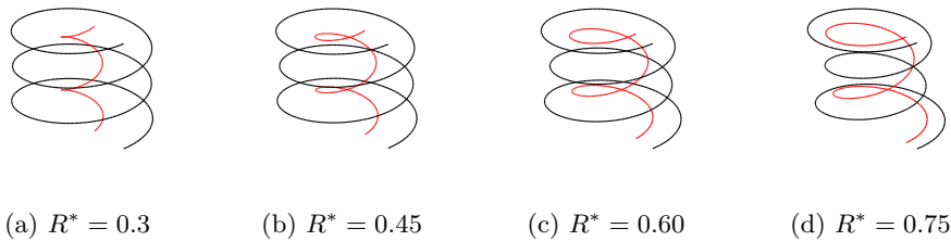
Figure 8: Representation of the deformed vortex structure for N = 1 , \kappa = 1 , h^* = 2 , \alpha = 1.5 , \varepsilon = 0.06 and different values of R^*
