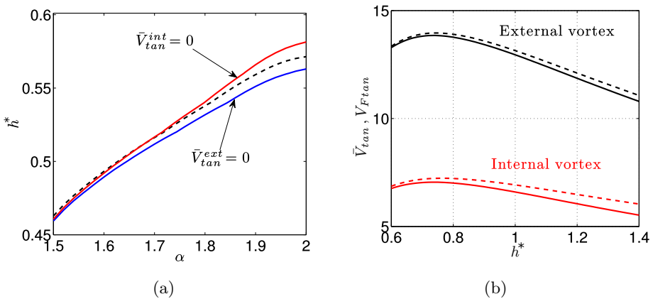
Figure 16: (a) Value of h^* versus \alpha for which \Omega_F = 0 (black dashed line), \bar{V}_{tan}^{ext} = 0 (blue line), \bar{V}_{tan}^{int} = 0 (red line) for R^* = 0.5 , \varepsilon = 0.03 , N = 1 , \kappa = 1 . (b) Comparison of mean tangential velocity \bar{V}_{tan} (solid lines) and tangential frame velocity V_{Ftan} (dashed lines) for external and internal vortices (normalized by \Gamma/R_{ext} ). Parameters are R^* = 0.5 , \alpha = 1.2 , \varepsilon = 0.03 , N = 1 , \kappa = 1 .
