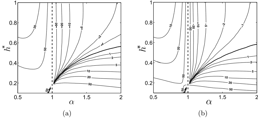
Figure 15: Contour values of the mean tangential velocities in the (\alpha, h) plane for R^* = 0.5 , \varepsilon = 0.03 , N = 1 , \kappa = 1 . (a) External vortex: \bar{V}_{tan}^{ext} R_{ext}/\Gamma . (b) Internal vortex: \bar{V}_{tan}^{int} R_{ext}/\Gamma . The dashed line ( \alpha = 1 ) indicates a line where \bar{V}_{tan}^{ext} and \bar{V}_{tan}^{int} are not defined. The thick solid curve corresponds to the level zero.
