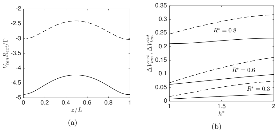
Figure 14: (a) Variation of the tangential velocity on a period in the internal vortex (dashed line) and in the external vortex (solid line) for a typical case ( R^* = 0.6 , h^* = 1.5 , \alpha = 1.4 and \varepsilon = 0.03 , N = 1 , \kappa = 1 ). (b) Maximum tangential velocity fluctuation in the internal vortex (dashed lines) and external vortex (solid lines) as a function of h^* for different values of R^* and \alpha = 1.4 , \varepsilon = 0.03 , N = 1 , \kappa = 1 .
