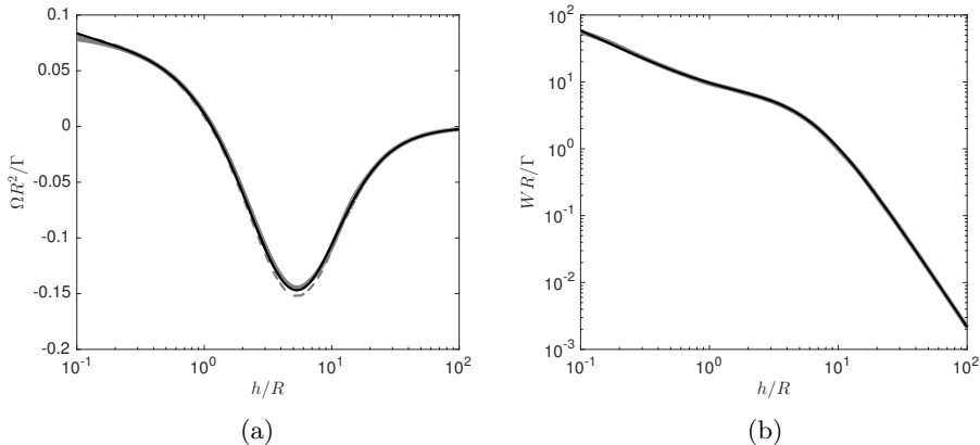
Figure 3: Non-dimensionalized rotation rate \Omega R^2/\Gamma (a) and axial speed WR/\Gamma (b) of a right-handed helix of circulation \Gamma , radius R , pitch h and core size a as a function of h/R for a/R = 0.03 . The solid black curves correspond to the numerical results obtained in this work. The solid grey curves correspond to the theoretical expressions (A 1a,b), the dashed grey curves correspond to the results obtained by Velasco Fuentes (2018), that is the same expressions without the 1/4 terms. Both theoretical results are for an equivalent Rankine vortex of core size a/R = 0.0408 .
