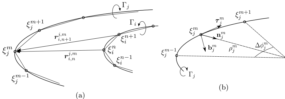
Figure 1: Discretization procedure of the vortex filaments. (a) Discretization in segments of two filaments of circulation \Gamma_i and \Gamma_j . (b) Arc of circle formed by three consecutive points of a discretized filament for the computation of the local contribution.
