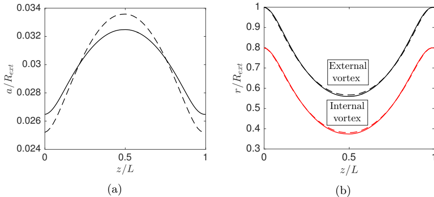
Figure 20: (a) Variation of the core size a/R_{ext} for the external (solid line) and internal (dashed line) vortex. The mean core size value in each vortex is a/R_{ext} = 0.03 . (b) Radial position of the internal and external vortices for a constant core size (dashed line) and for a variable core size obtained using (4.1) (solid line). The parameters in both figures are R^* = 0.8 , h^* = 1.4 , \alpha = 1.4 , N = 1 , \kappa = 1 and a mean core size a/R_{ext} = 0.03 .
