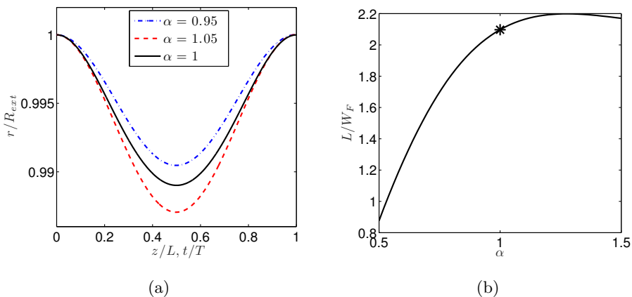
Figure 11: Characteristics close to \alpha = 1 for h^* = 1 , \varepsilon = 0.01 , N = 1 , \kappa = 1 . (a) Comparison of the radial positions of deformed helices versus z/L for \alpha = 1.05 and \alpha = 0.95 with the radial position of perfect helices versus t/T for \alpha = 1 . (b) Variation of the characteristic time scale L/W_F versus \alpha . The symbol represents the period T of the temporal evolution of perfect helices for \alpha = 1 .
