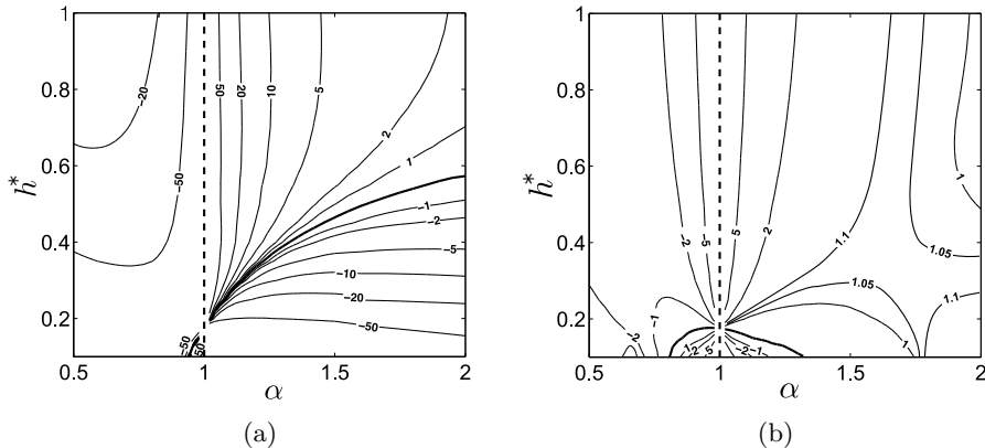
Figure 13: Contour values of the frame velocity in the (\alpha, h) plane for R^* = 0.5 , \varepsilon = 0.03 , N = 1 and \kappa = 1 . (a) Angular velocity \Omega = \Omega_F R_{ext}^2 / \Gamma , (b) Axial velocity W = W_F R_{ext} / \Gamma . The dashed line ( \alpha = 1 ) indicates a line where \Omega and W are not defined. The thick solid curve corresponds to the level zero.
