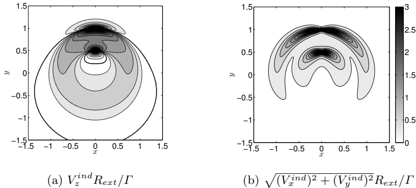
Figure 17: Induced velocity contours in a cross section ( z = 0 plane) for h^* = 1 , R^* = 0.5 , \alpha = 1.5 , \varepsilon = 0.03 , N = 1 and \kappa = 1 . In (a) colors are for |V_z^{ind}| with the same colormap as in (b).
