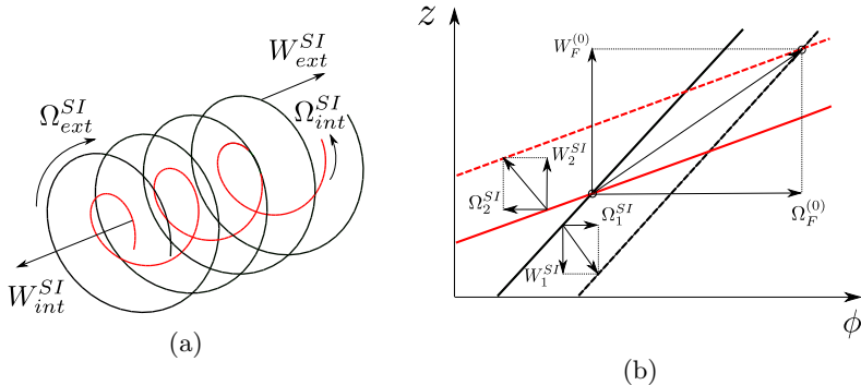
Figure 5: (a) Self-induced velocities of a pair of coaxial vortices when the mutual induction is negligible. (b) Schematic diagram showing how the moving frame velocities \Omega_F^{(0)} and W_F^{(0)} are obtained. Solid and dashed lines represent the two helices at t = 0 and t = 1 respectively. The frame velocity is given by the vector connecting the crossing points of solid lines with dashed lines. The axial and azimuthal components of this vector provides W_F^{(0)} and \Omega_F^{(0)} respectively.
