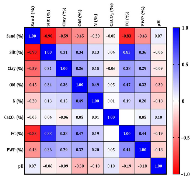
FIGURE 4 Pearson's correlation analysis of selected soil physicochemical parameters for the fluvisols in the Málaga province. Blue color indicates a positive correlation, while red color exhibits a negative correlation at p < .05 . Blank boxes represent no correlation among parameters [Color figure can be viewed at wileyonlinelibrary.com ]
