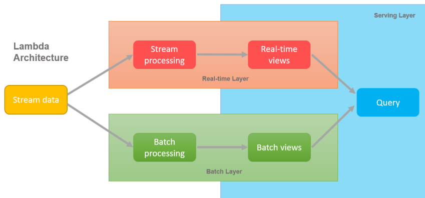
Figure 3: Lambda Architecture
