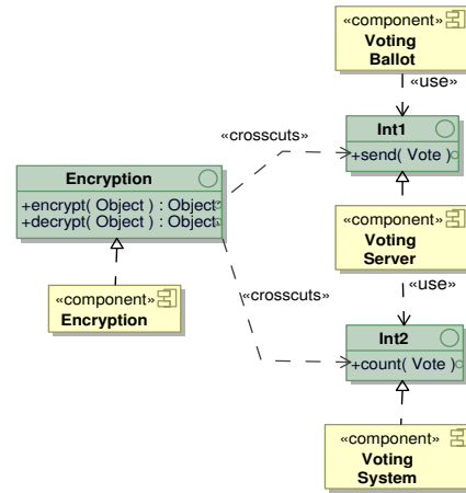
Figure 12: Result of applying Weaving Pattern 5 for Encryption.
