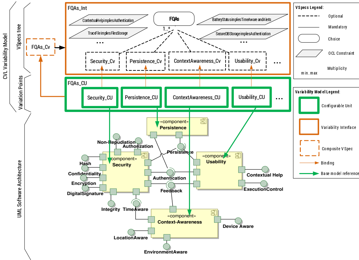
Figure 4: Complete variability model of the FQAs in CVL.
