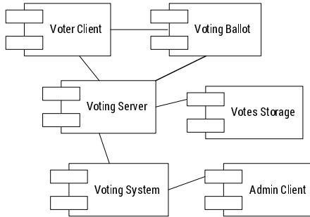
Figure 1: E-voting software architecture.
