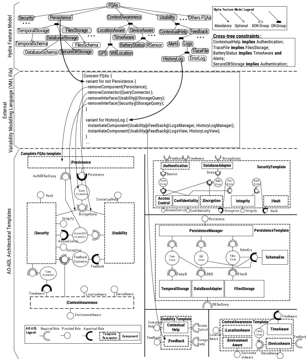
Figure 3: Domain Engineering of the FQA family using FMs, AO-ADL and VML languages.
