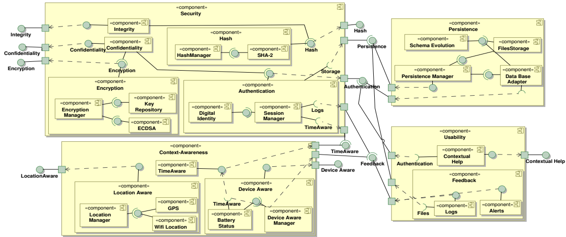
Figure 6: FQAs architecture configuration (resolved model of the FQAs).
