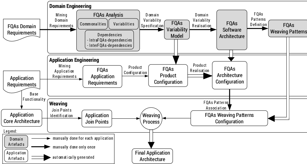
Figure 2: Generic process for weaving FQAs customised for an application.
