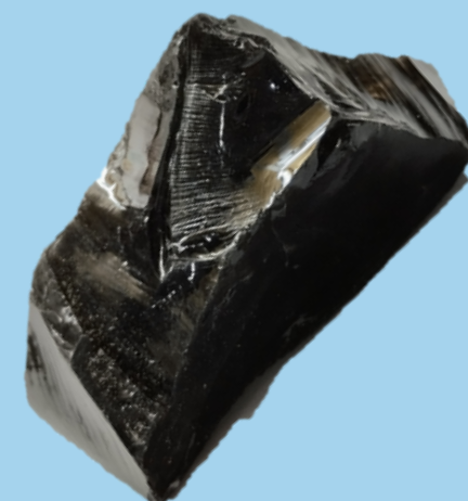
Obsidiana
