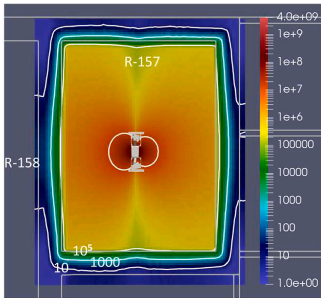
Fig. 17. Shutdown dose rate ( \mu\text{Sv/h} ) in the RWTS room R157 contributed by HFTM after 1-day cooling.
