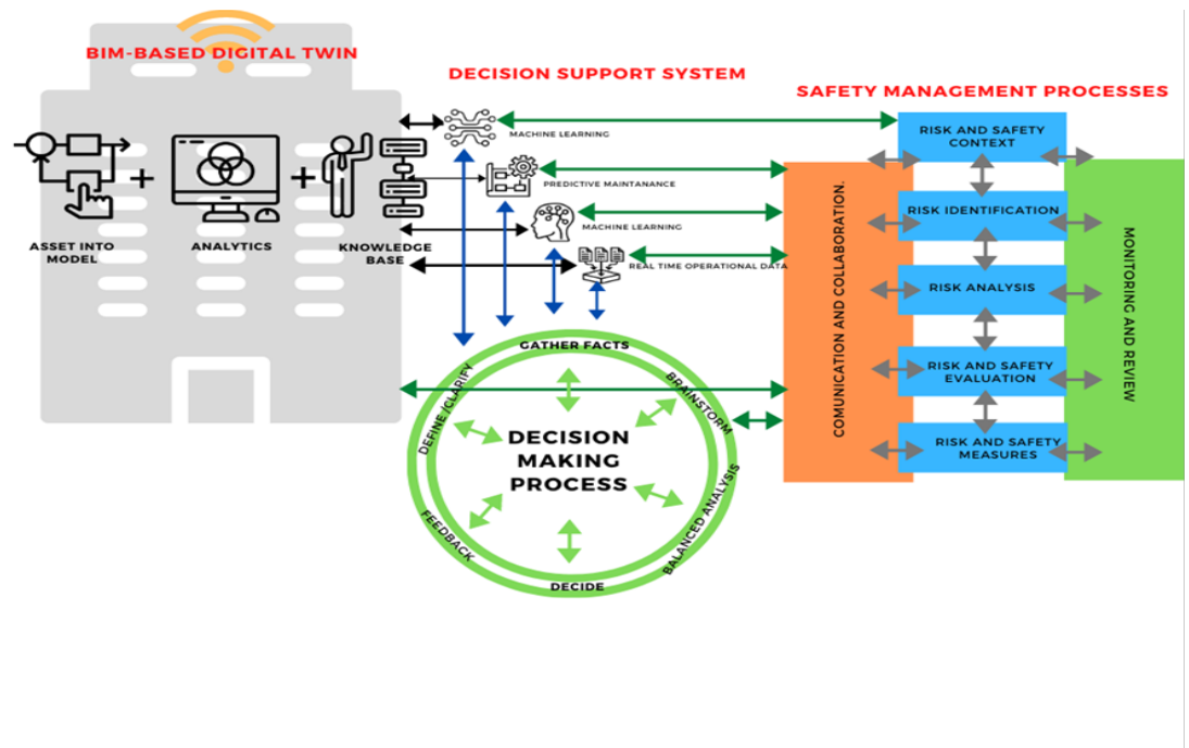
Figura 3 Proposed Framework of the BIM-based digital twin within decision-making of safety management.
