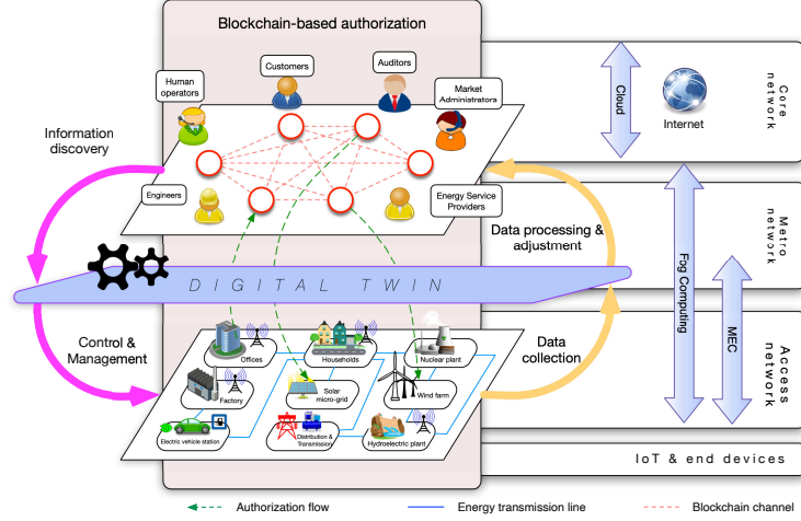
Figure 2: B5G-enabled Smart Grid architecture for accommodating DTs in the long term
