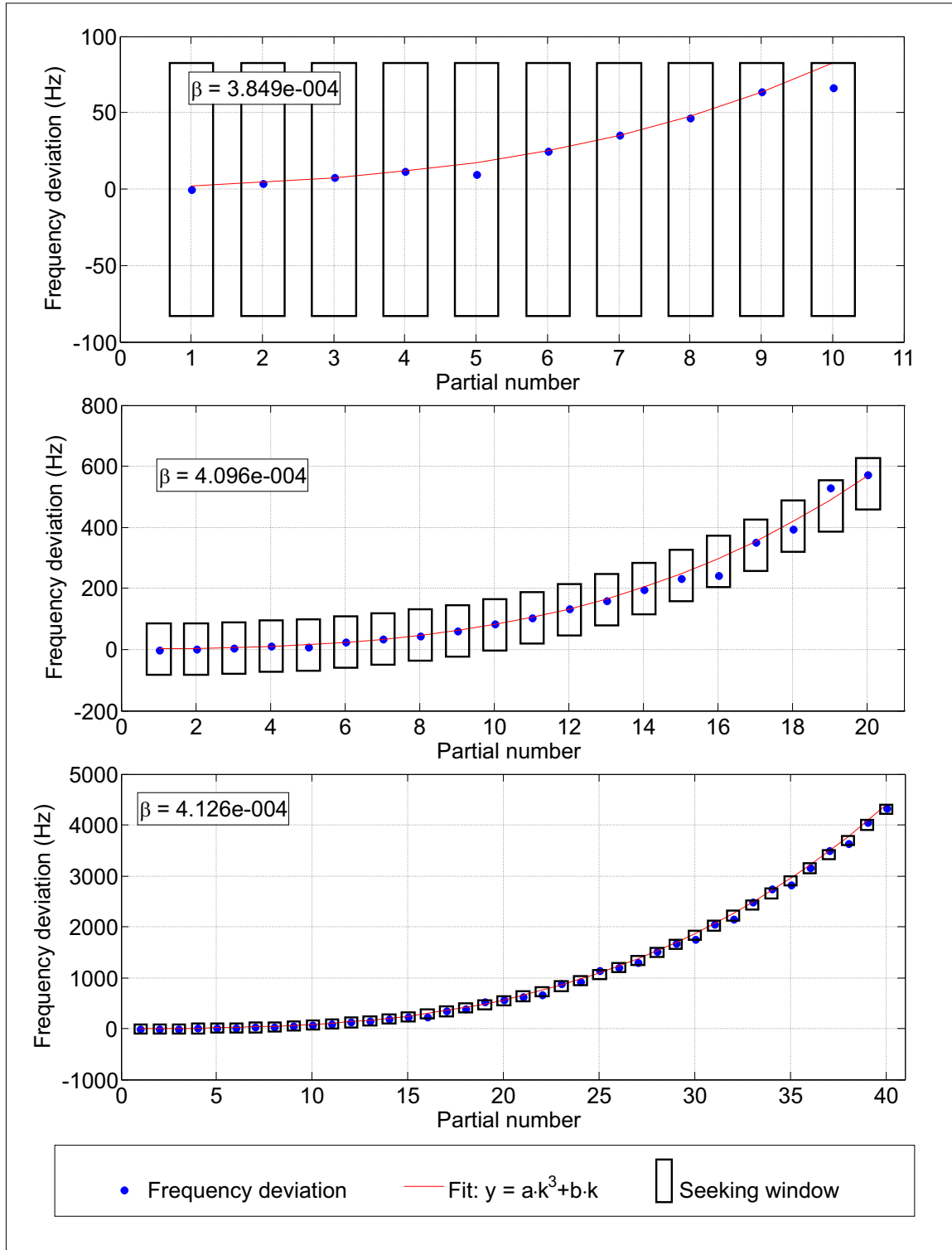
Fig. 6. Illustration of the refinement of the calculus of the inharmonicity coefficient for note E4, played on the 9-th fret of the 3-th string. Iterations 1, 2 and 3 are shown from top to bottom, respectively. The search windows are shown as boxes. The measured deviations for each partial are marked with dots. The fitted polynomial at each iteration is also drawn.
