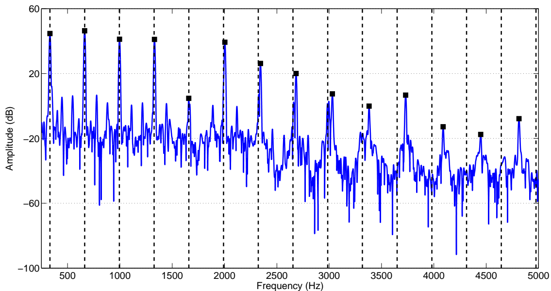
Fig. 4. Spectrum of the note E4, with f_0(3, 9) = 329.63\text{ Hz} . Detected partials are marked with filled squares. Multiples of the fundamental frequency are marked using dashed vertical lines.
