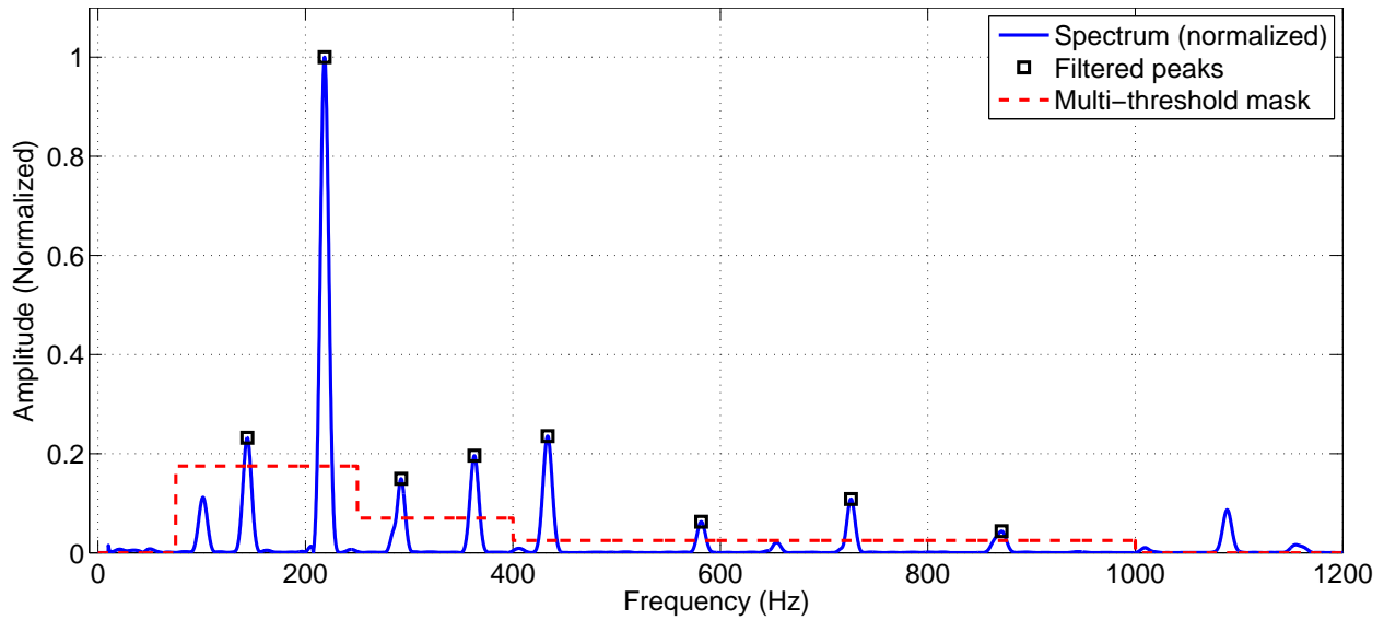
(a) The masked spectrum (normalized amplitude).
