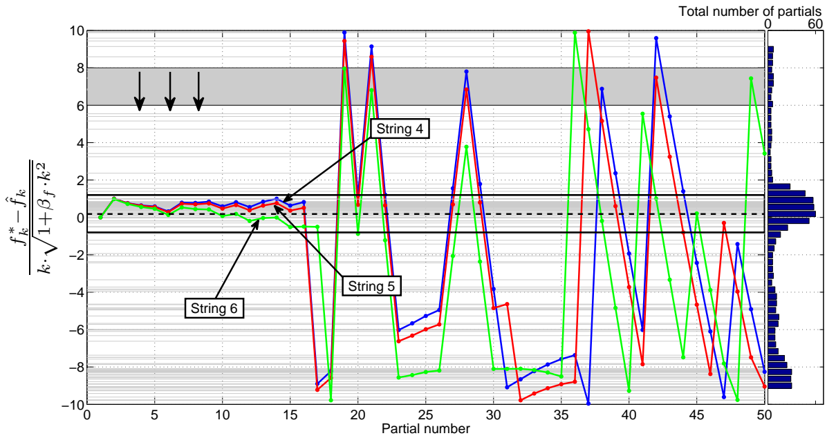
Fig. 7. Example of the voting procedure for the estimation of the error \epsilon_f for the note E3 using v_k(s, n) as defined in eq. (24), with R = 10\text{Hz} . Sample containers are shown in gray with dashed edges. The most populated container is displayed in gray with its center marker with a dashed thick line.
