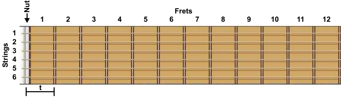
Fig. 3. A schematic representation of the guitar fingerboard.
