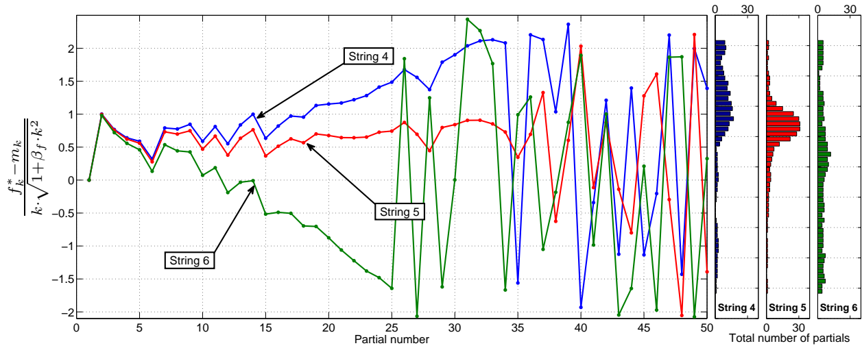
Fig. 8. Example of the second stage of the voting procedure for the detection of the note/string/fret corresponding to a note E3 played, using v'_k(s, n) as defined in eq. (25), with R = 2.3\text{Hz} .
