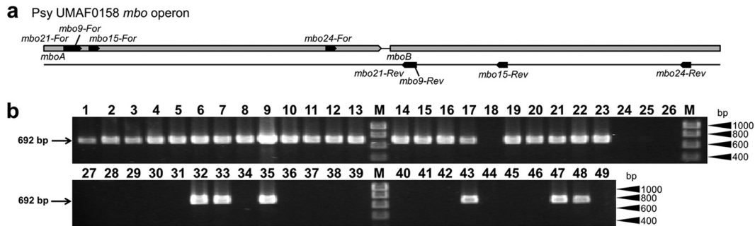
FIG 2 Detection by PCR of a specific mangotoxin biosynthesis operon sequence in different P. syringae genomospecies 1 strains. (a) Schematic representation of the four primer pairs designed for mbo operon detection in P. syringae strains. (b) Gel electrophoresis showing the specific 692-bp product generated with primers mbo24-For and mbo24-Rev from strains harboring the mbo operon. Lanes correspond to the following: 1, P. syringae pv. syringae 7C67; 2, P. syringae pv. syringae 7F29; 3, P. syringae pv. syringae 8F21; 4, P. syringae pv. syringae 1559-9; 5, P. syringae pv. syringae CECT127; 6, P. syringae pv. syringae CECT4429; 7, P. syringae pv. syringae CFBP3388; 8, P. syringae pv. syringae DAR77787; 9, P. syringae pv. syringae DAR77789; 10, P. syringae pv. syringae EPS17A; 11, P. syringae pv. syringae NCPPB1239; 12, P. syringae pv. syringae Ps-5; 13, P. syringae pv. syringae UMAF0081; 14, P. syringae pv. syringae UMAF0214; 15, P. syringae pv. syringae UMAF0225; 16, P. syringae pv. syringae UMAF1060; 17, P. syringae pv. syringae UMAF6024; 18, P. syringae pv. syringae UMAF6016; 19, P. syringae pv. pisi 1704B; 20, P. syringae pv. pisi HRI203; 21, P. syringae pv. pisi NCPPB1365; 22, P. syringae pv. avellanae ISPaVe011; 23, P. syringae pv. avellanae ISPaVe2056; 24, P. syringae pv. syringae 7D46; 25, 8B48; 26, P. syringae pv. syringae 8C43; 27, P. syringae pv. syringae ITACyL 488; 28, P. syringae pv. syringae ITACyL 521; 29, P. syringae pv. syringae ITACyL 523; 30, P. syringae pv. syringae ITACyL 526; 31, P. syringae pv. syringae ITACyL 529; 32, P. syringae pv. syringae 1444-5; 33, P. syringae pv. syringae FF5; 34, P. syringae pv. syringae EPSMV3; 35, P. syringae pv. syringae UMAF0167; 36, P. syringae pv. tomato DC3000; 37, P. syringae pv. tomato DCT6D1; 38, P. syringae pv. tomato UMAF4007; 39, P. syringae pv. tomato UMAF6018; 40, P. syringae pv. coronafaciens CECT4389; 41, P. syringae pv. phaseolicola 1448A; 42, P. syringae pv. phaseolicola CYL314; 43, P. syringae pv. aptata DSM50252; 44, P. syringae pv. syringae 1507-7; 45, P. syringae pv. syringae B728a; 46, P. syringae pv. syringae CECT4430; 47, P. syringae pv. syringae 0049; 48, P. syringae pv. syringae UMAF0158; 49, P. syringae pv. tabaci ATCC 11528; M, molecular size marker (HyperLadder I; Bioline).
