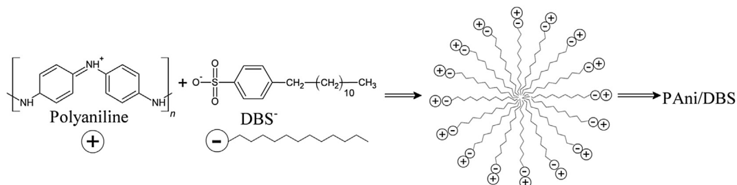
Fig. 5. Scheme of micelle formation prior to PANi/DBS polymerization.
