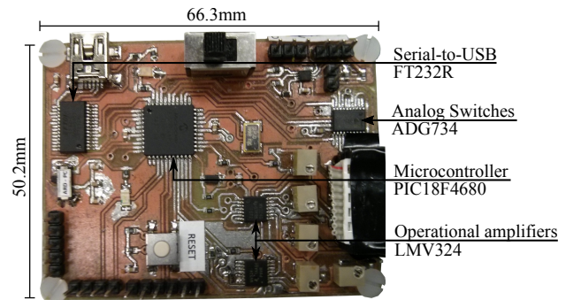
Figure 4. Conditioning electronics board.
