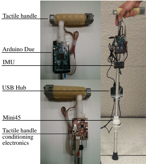
Figure 6. Experimental setup.
