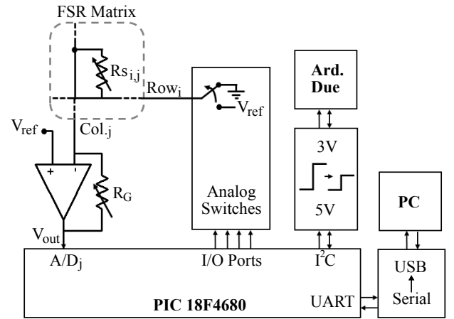
Figure 3. Conditioning electronics scheme.
