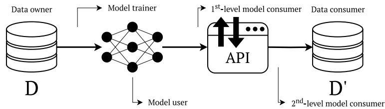
Fig. 1. Different levels of knowledge and access to the trained model.
