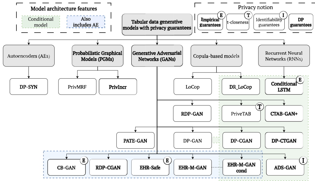
Fig. 7. Privacy-preserving tabular data generative models taxonomy.
