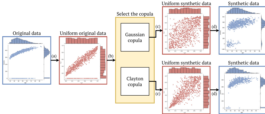
Fig. 6. Bivariate copula workflow. (a) Original data is transformed to uniform using the corresponding CDFs. (b) Select a copula that resembles the uniform transformation and fit its parameters. (c) Generate samples using the fitted copula on the uniform interval. (d) Use inverse CDFs to transform the uniform samples into the original distributions.
