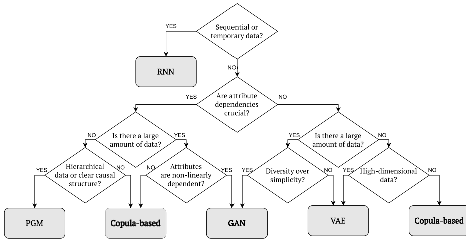
Fig. 10. Decision tree for model selection. The questions guide the identification of the model that, a priori, is most suitable for generating synthetic data that resembles the original data.
