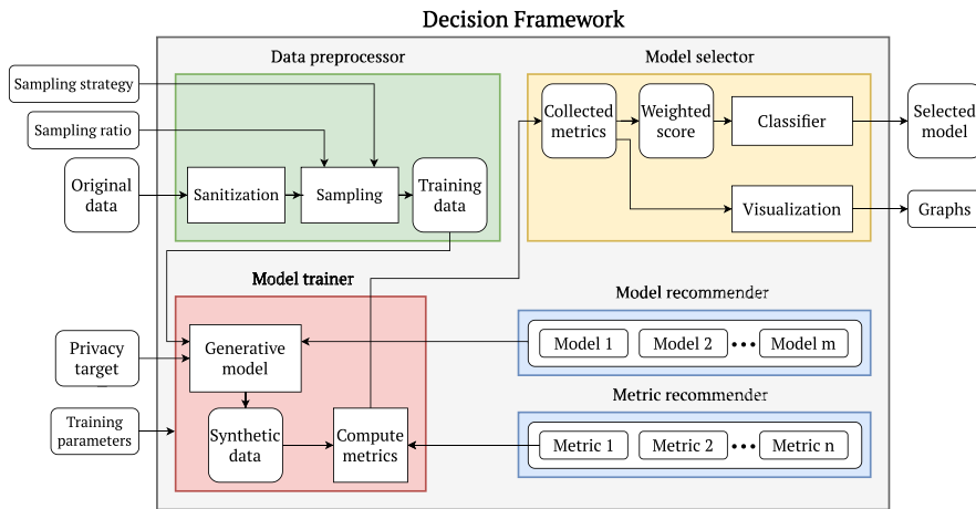
Fig. 9. Framework components diagram. The inputs are on the left and the outputs are on the right. The large colored boxes represent the different components. Rectangles with rounded corners represent variables or data, and rectangles with straight corners represent functions or processes.
