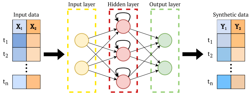
Fig. 4. RNN diagram consisting of three layers of neurons. The input data consists of n rows, each corresponding to a time point t_i of a sequence. The hidden layer receives input from both the input layer's outputs and its own previous state. This feedback mechanism enables the hidden layer to learn temporal and sequential dependencies within the data.
