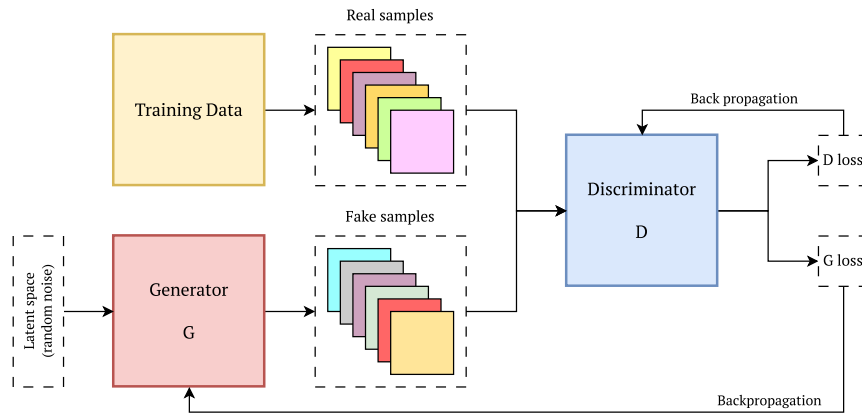
Fig. 2. Vanilla GAN block diagram. G generates samples from noise and uses them to feed D. D tries to distinguish between real and fake data. Losses are obtained from D to train G and D.
