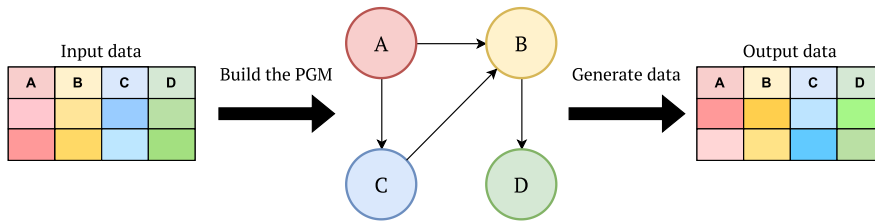
Fig. 5. PGM diagram: Each node A, B, C, and D represents an attribute of the input data, and their dependencies are represented by arrows.
