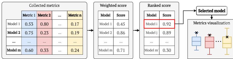
Fig. 11. Model selector diagram: The collected metrics are used to assign to each model an aggregated score based on user defined weights that can be used to select the best model. Additionally, the component provides visualizations to compare each model's metrics against the others.
