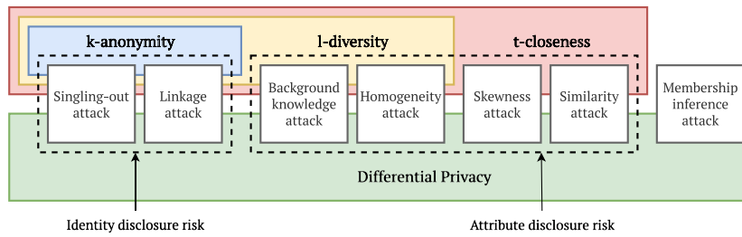
Fig. 8. Attacks on privacy and what privacy notions protect against them.
