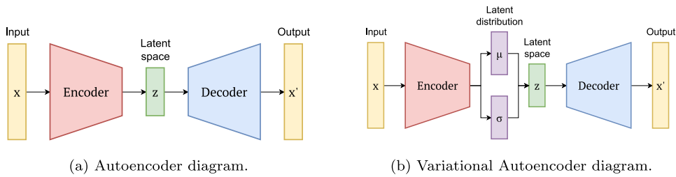
Fig. 3. Autoencoder structure. The encoder compresses the input into a latent space, and the decoder reconstructs the input from that latent representation.
