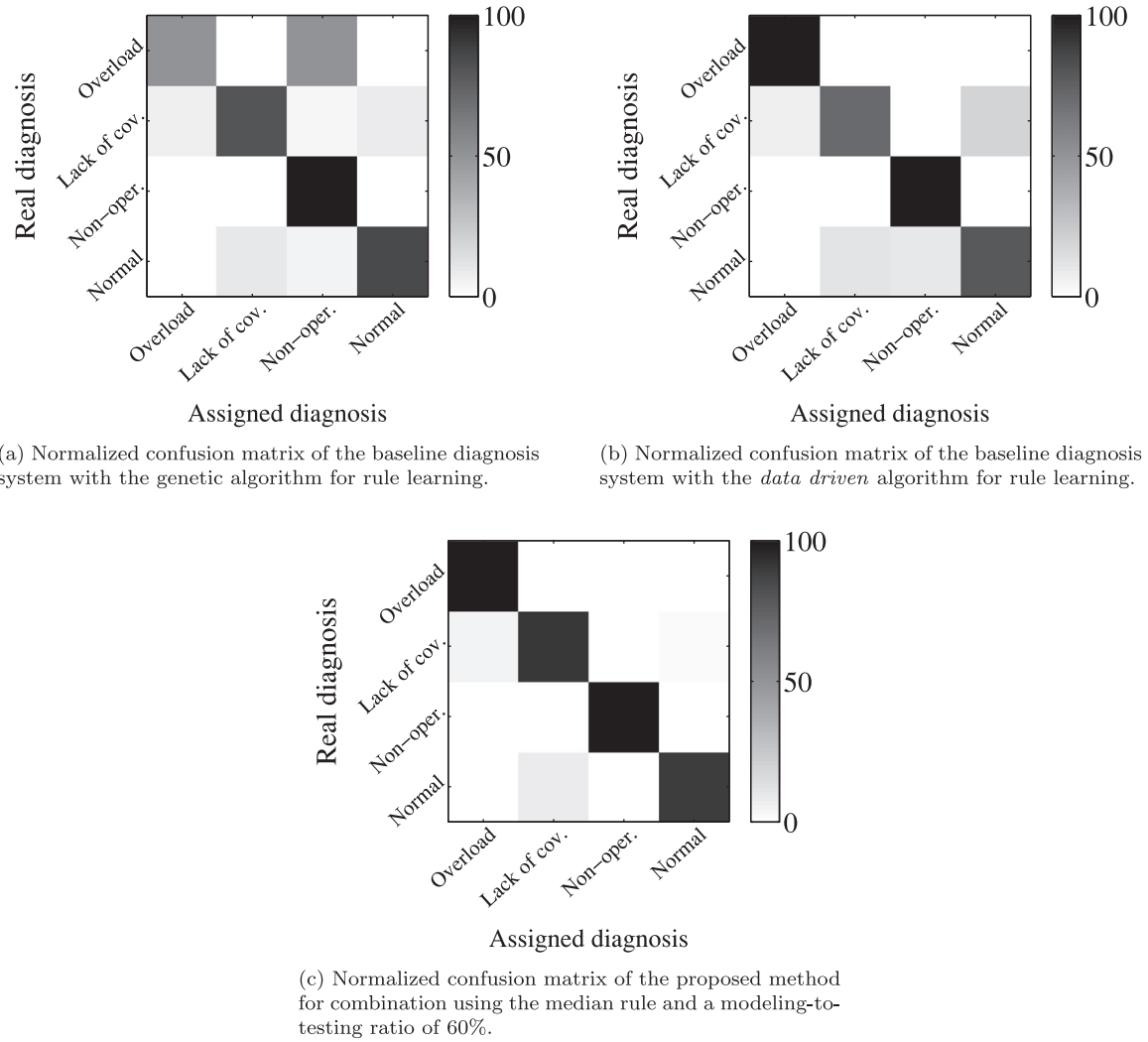
Fig. 6. Normalized confusion matrices for the second test.
