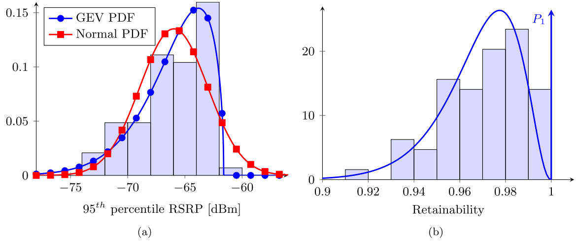
Fig. 4. (a) Normalized histogram for the KPI 95th percentile RSRP and two fitted PDFs: a generalized extreme value PDF in blue (round markers) and a normal PDF in red (square markers). (b) Normalized histogram for the KPI Retainability and a \beta' PDF estimation. (For interpretation of the references to colour in this figure legend, the reader is referred to the web version of this article.)
