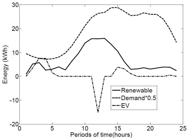
Fig. 8. Renewable energy output, total demand and EVs contribution
