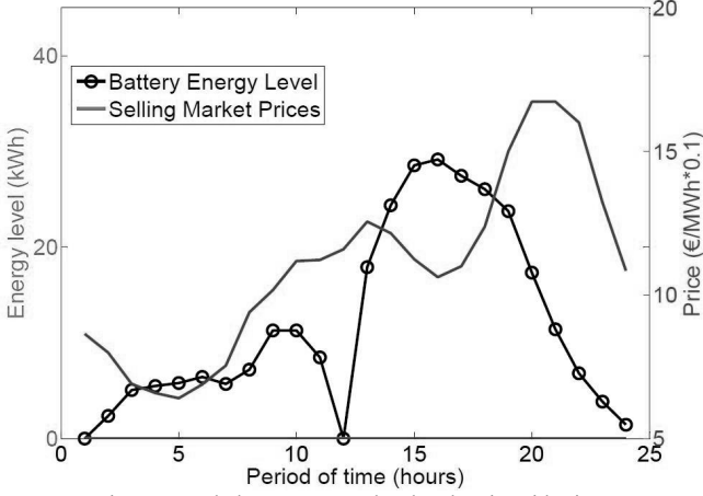
Fig. 5. Hourly battery energy level and main grid prices
