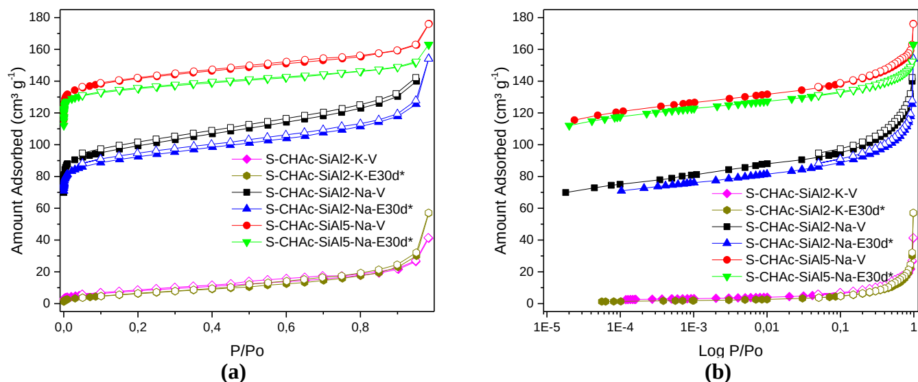
Figure 5.2.7. N_2 Isotherms at 77 K in linear (a) and logarithmic (b) scales for the Samples S – CHAc – SiAl(2, 5) – (Na, K) – (V, E30d*)
