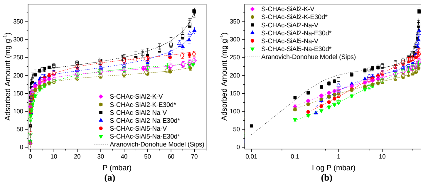
Figure 5.2.9. H 2 O Isotherms at 313 K in linear (a) and logarithmic (b) scales for the Samples S-CHAc-SiAl(2, 5)-(Na, K)- (V, E30d*)
