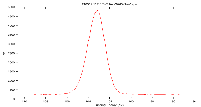
Figure 7.1.3. XPS Spectrograms for All Contributions in the Chabazite Samples S-CHAc-SiAl5-Na-V Spectrogram
