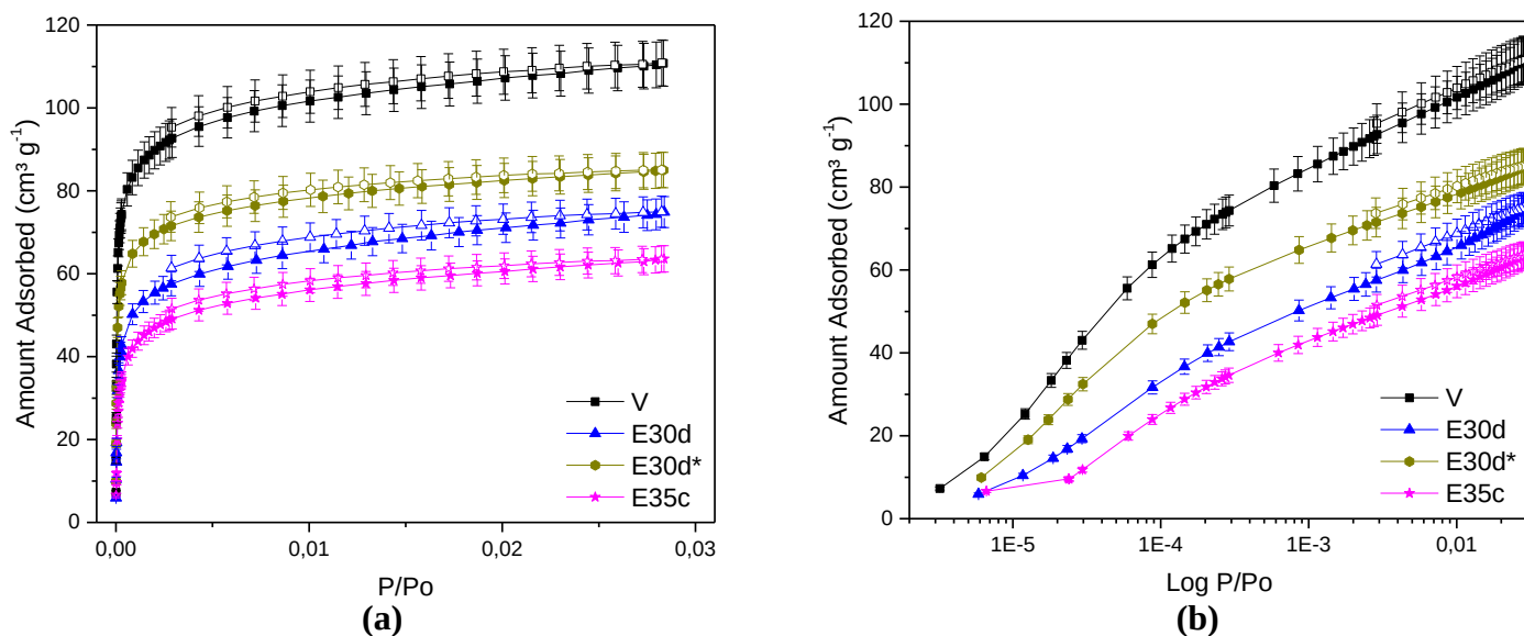
Figure 5.1.9. CO 2 Isotherms at 273 K in linear (a) and logarithmic (b) scales for sample (S-CHA C -SiAl 2 -Na): Pristine (V); Aged by PAP-1 (E35c) and by PAP-2 in a Single (E30d) and Dual (-E30d*) Sample Port
