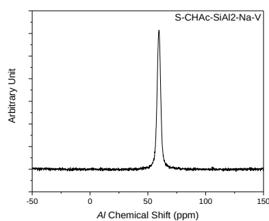
Figure 7.3.1. ^{27}\text{Al} and ^{29}\text{Si} NMR Spectrum for the Samples S-CHAc-SiAl 2 -Na S-CHAc-SiAl 2 -Na-V
