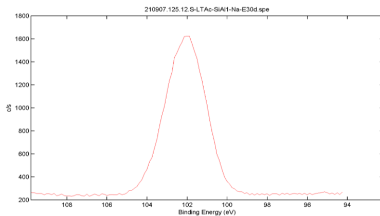
Figure 7.2.2. XPS Spectrograms for All Contributions in the Chabazite Samples S-LTA C -SiAl 1 -Na-E30d*
