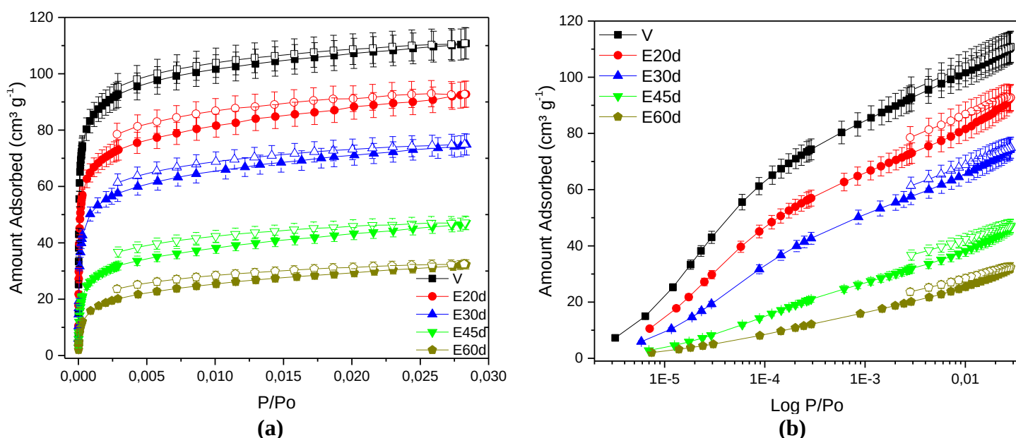
Figure 5.1.5. CO_2 Isotherms at 273 K for the S- CHA_C -SiAl 2 -Na Series Aged by PAP-2 in linear (a) and logarithmic (b) scales
