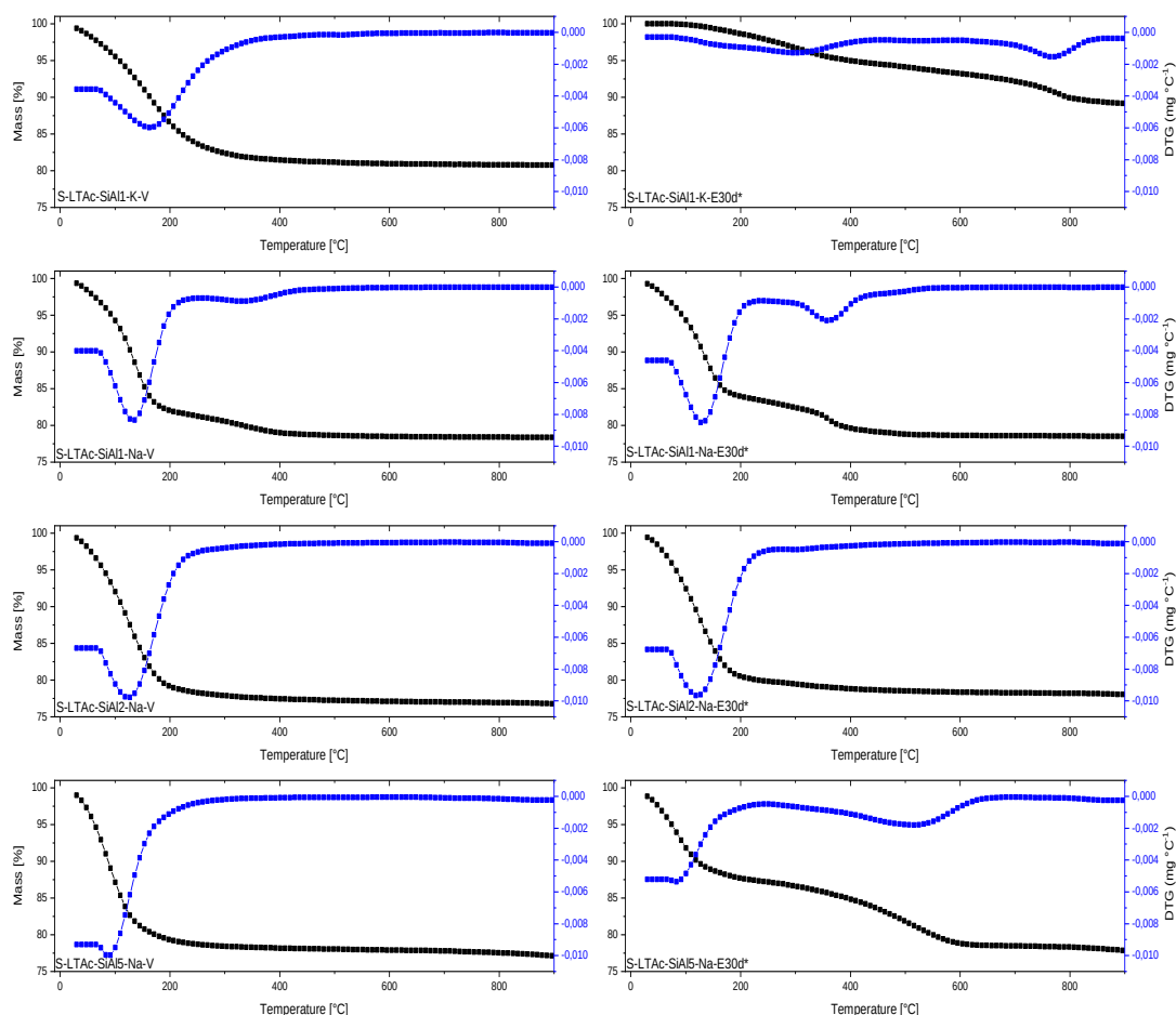
Figure 5.3.5. TG/DTG curves for the S-LTAc-SiAl(1, 2, 5)- (Na, K)- (V, E30d*) Samples
