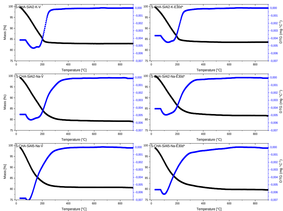
Figure 5.2.6. TG/DTG curves for the S-CHAc-SiAl(2, 5)- (Na, K)- (V, E30d*) Samples
