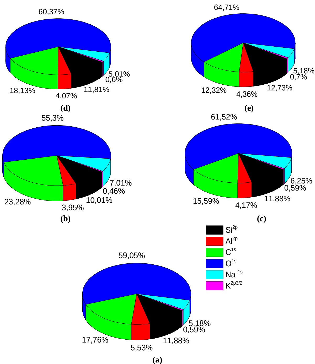
Figure 5.1.3. Chemical Surface Composition (% mass concentration) Determined by XPS Analysis for the S-CHAc-SiAl 2 -Na-V (a); S-CHAc-SiAl 2 -Na-E20d (b); S-CHAc-SiAl 2 -Na-V-E30d (c); S-CHAc-SiAl 2 -Na-E45d (d); S-CHAc-SiAl 2 -Na-E60d (e) Samples Aged by PAP-2
