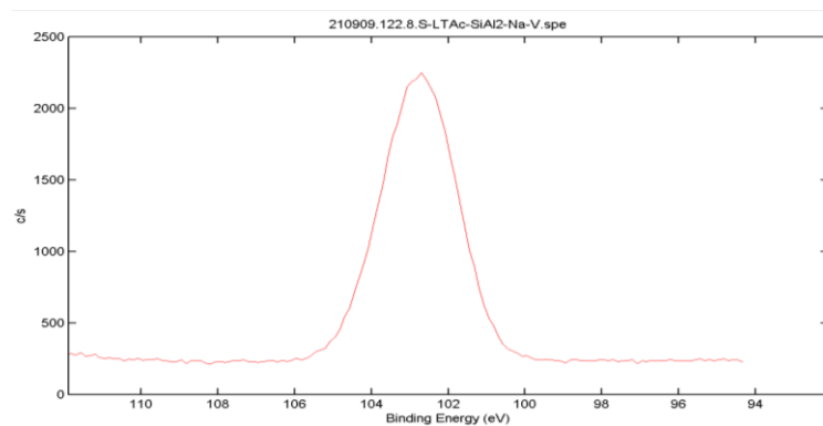
Figure 7.2.5. XPS Spectrograms for All Contributions in the Chabazite Samples S-LTAc-SiAl2-Na-V
