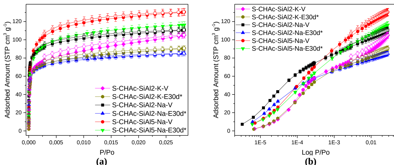
Figure 5.2.8. CO 2 Isotherms at 273 K in linear (a) and logarithmic (b) scales for the Samples S – CHAc – SiAl(2, 5) – (Na, K) – (V, E30d*)
