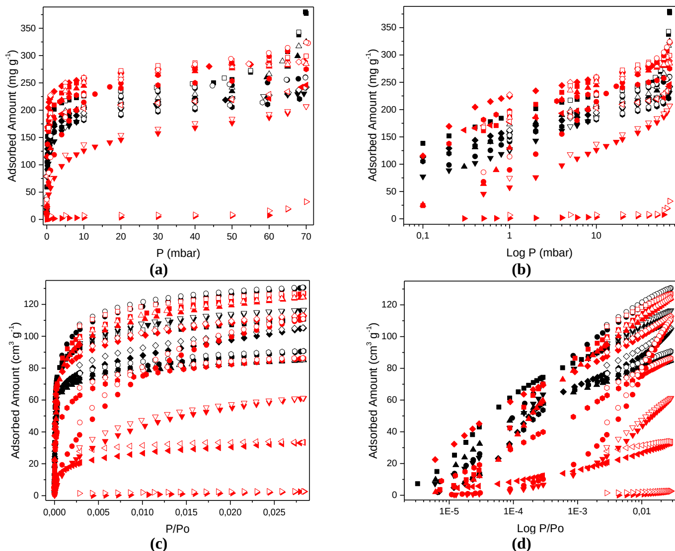
Figure 5.4.1. H 2 O Isotherms at 313 K in linear (a) and logarithmic (b) scales and CO 2 Isotherms at 273 K in linear (c) and logarithmic (d) scales for all studied samples
