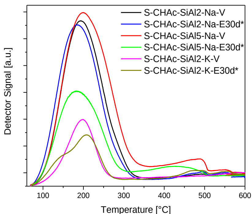
Figure 5.2.4. Detector signal in \text{NH}_3 temperature-programmed desorption for the S-CHAc-SiAl(2, 5)–( \text{Na} , \text{K} ) – (V, E30d*) Samples
