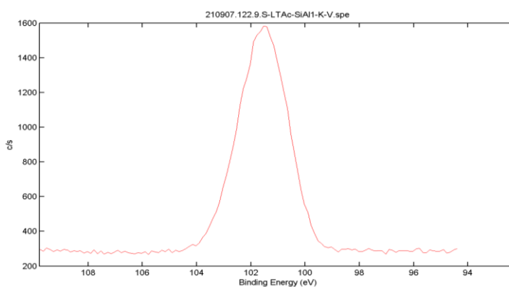
Figure 7.2.3. XPS Spectrograms for All Contributions in the Chabazite Samples S-LTA C -SiAl1-K-V
