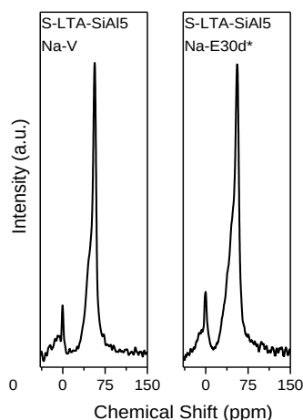
Figure 5.3.3. ^{27}\text{Al} NMR spectra for the sample S-LTAc-SiAl5-Na- (V, E30d*)
