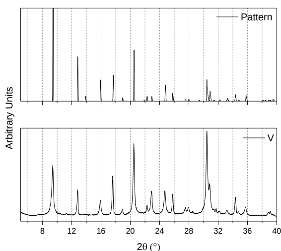
Figure 5.1.1. XRD Diffractograms for Pattern and Homemade Synthesized S-CHA C -SiAl 2 -Na-V Samples
