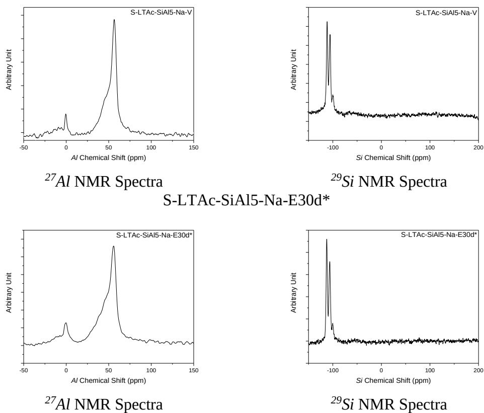
Figure 7.4.4. ^{27}\text{Al} and ^{29}\text{Si} NMR Spectrum for the Samples S-LTAc-SiAl 5 -Na S-LTAc-SiAl 5 -Na-V
