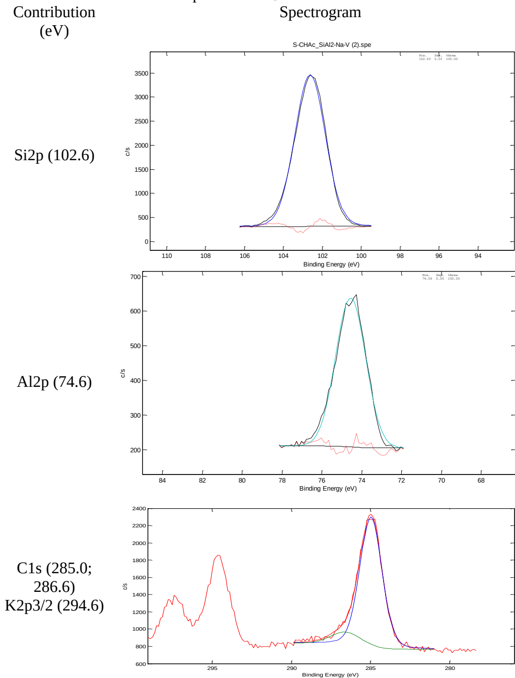
Figure 7.1.1. XPS Spectrograms for All Contributions in the Chabazite Samples S-CHAc-SiAl2-Na-V
