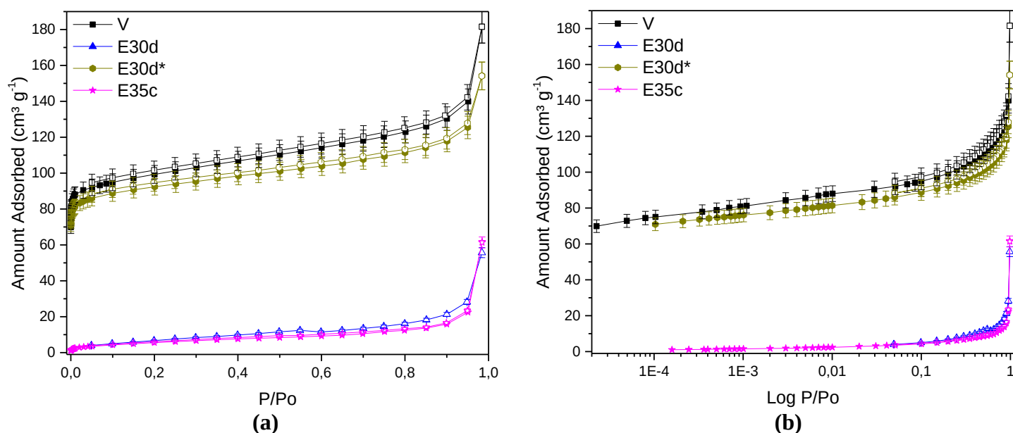
Figure 5.1.8. N 2 Isotherms at 77 K in linear (a) and logarithmic (b) scales for sample (S-CHAC-SiAl 2 -Na): Pristine (V); Aged by PAP-1 (E35c) and by PAP-2 in a Single (E30d) and Dual (E30d*) Sample Port
