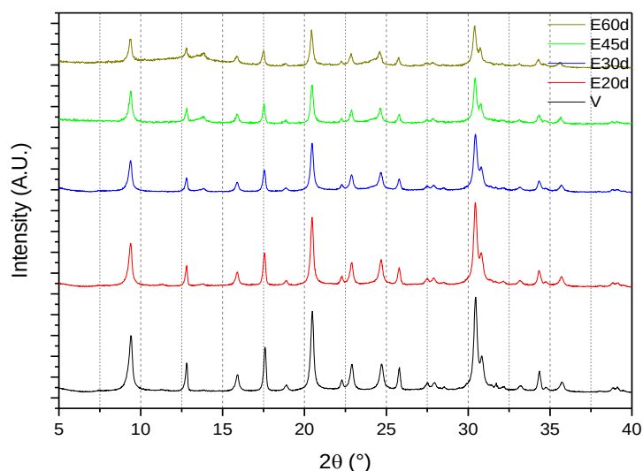
Figure 5.1.2. XRD Diffractograms for the S-CHAc-SiAl 2 -Na Series Aged by PAP-2
