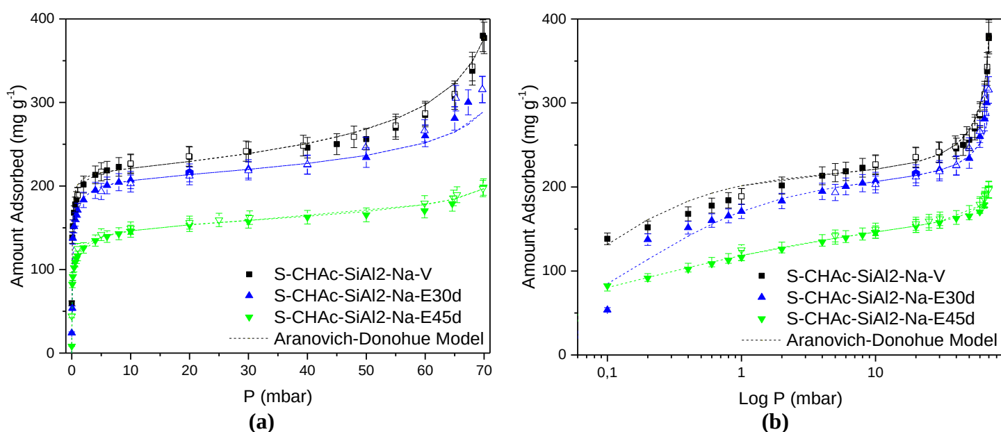
Figure 5.1.6. \text{H}_2\text{O} Isotherms at 313 K for the Samples S-CHAc-SiAl 2 -Na-(V, E30d, E45d) in linear (a) and logarithmic (b) scales
