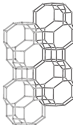
Figure 3.05. Chabazite (CHA)
