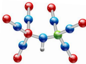
Figure 3.07. Brønsted Acid Sites in protonic zeolites [Blue spheres = O; Green sphere = Al; Red spheres = Si; White sphere = H].
