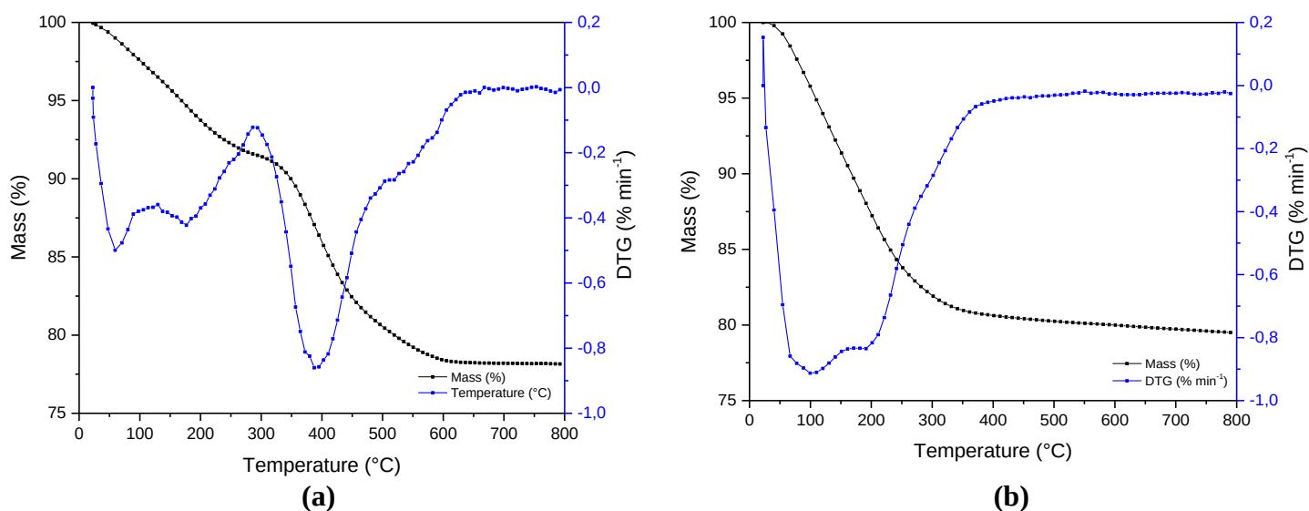
Figure 5.2.5. TG/DTG for the Pre-Calcinated S-CHAc-SiAl5-Na-V (a) and Calcined S-CHAc-SiAl5-Na-V (b) Samples
