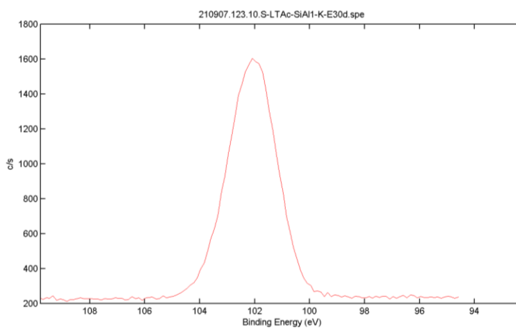
Figure 7.2.4. XPS Spectrograms for All Contributions in the Chabazite Samples S-LTAc-SiAl1-K-E30d*
