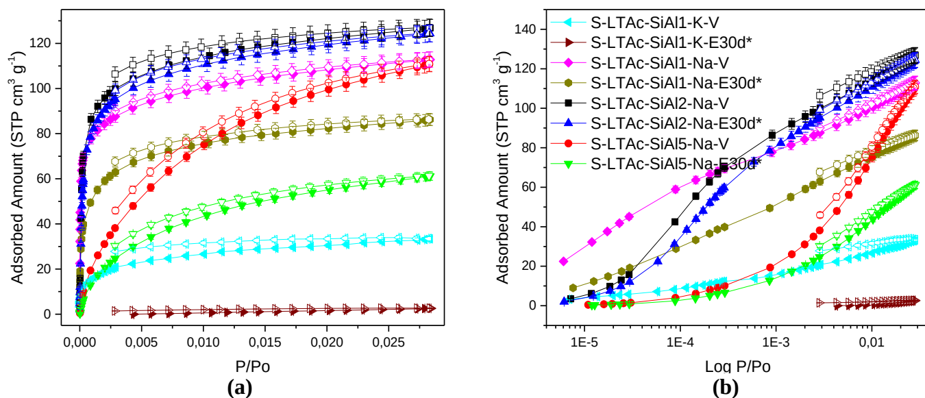
Figure 5.3.6. \text{CO}_2 Isotherms at 273 K in linear (a) and logarithmic (b) scales for the Samples S-LTAc-SiAl(1, 2, 5) - (Na, K) - (V, E30d*)
