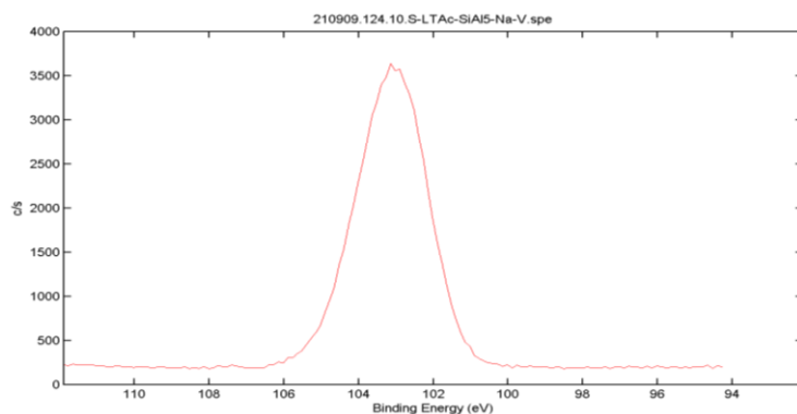
Figure 7.2.7. XPS Spectrograms for All Contributions in the Chabazite Samples S-LTA C -SiAl5-Na-V Spectrogram
