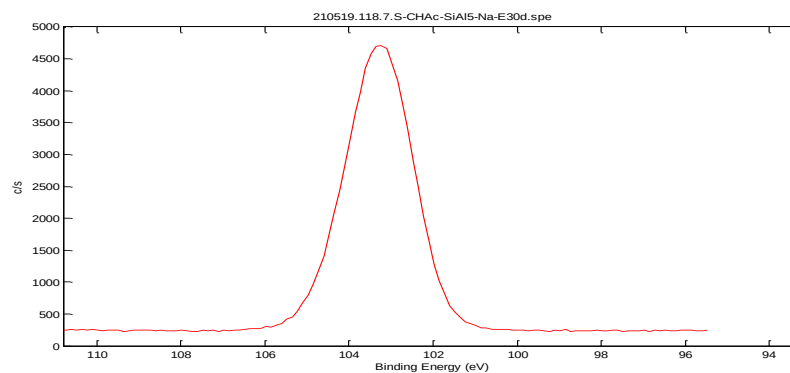
Figure 7.1.4. XPS Spectrograms for All Contributions in the Chabazite Samples S-CHAc-SiAl5-Na-E30d*
