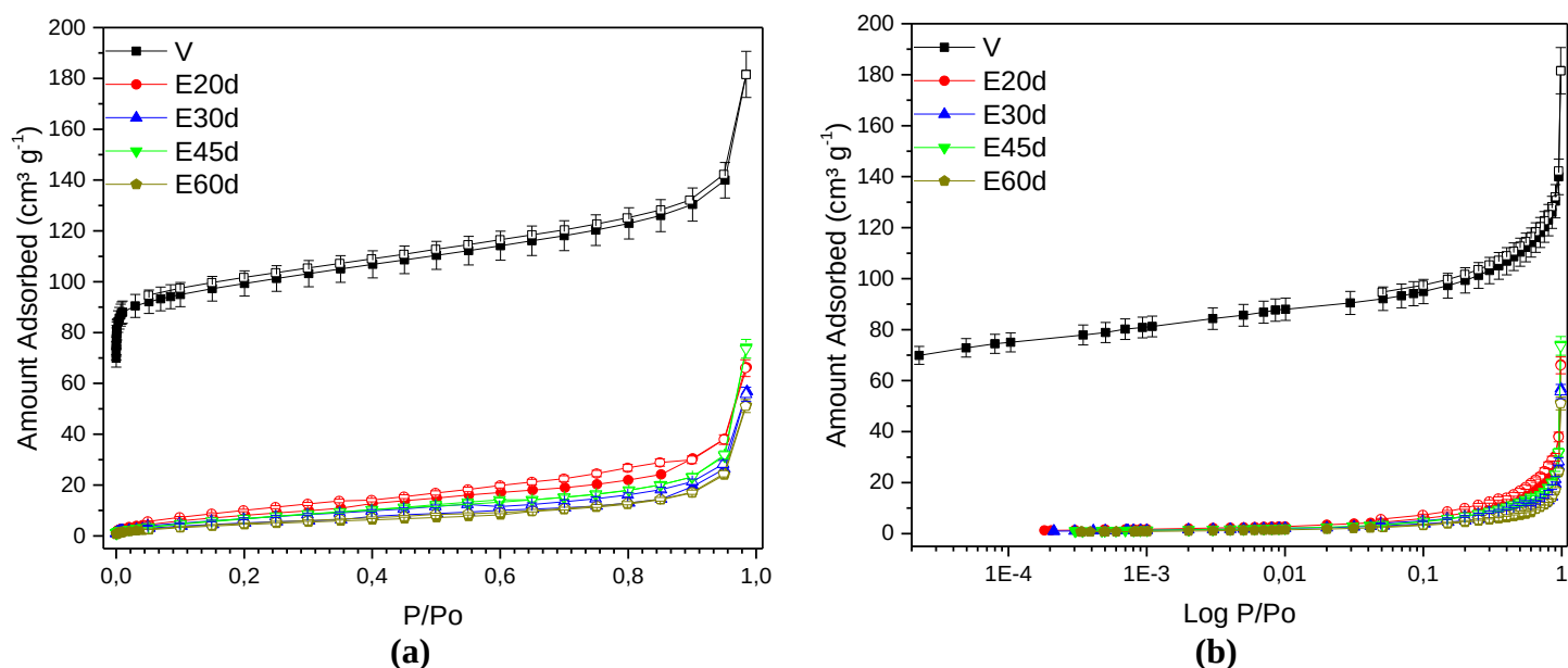
Figure 5.1.4. N 2 Isotherms at 77 K for the S-CHAC-SiAl 2 -Na Series Aged by PAP-2 in linear (a) and logarithmic (b) scales
