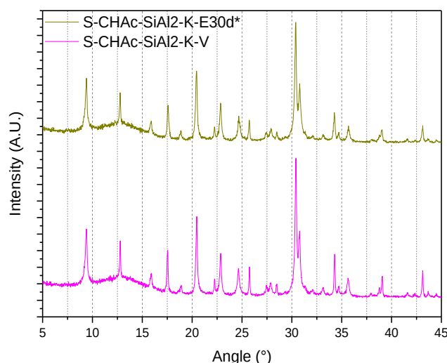
Figure 5.2.1. XRD Diffractograms for Samples S-CHAc-SiAl2-Na- (V, E30d*) (a), S-CHAc-SiAl5-Na- (V, E30d*) (b) and S-CHAc-SiAl2-K- (V, E30d*) (c)
