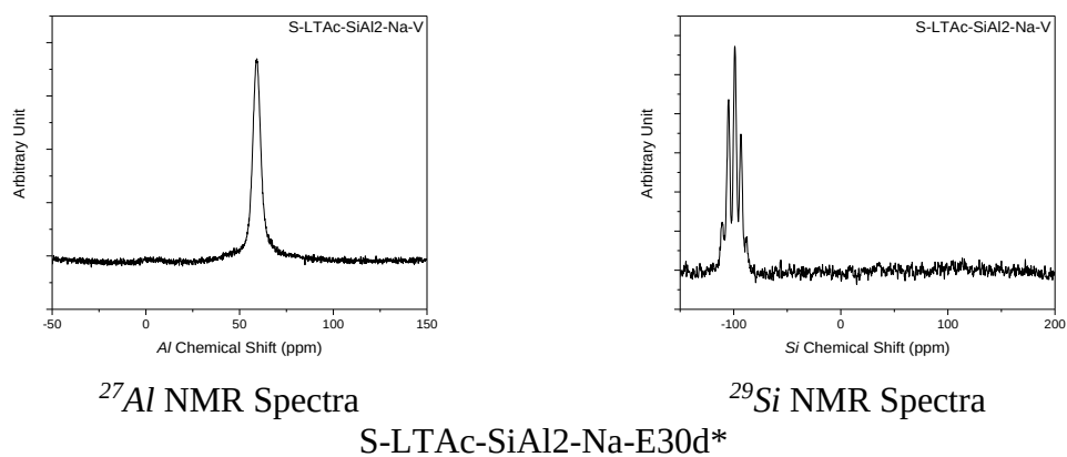
Figure 7.4.3. ^{27}\text{Al} and ^{29}\text{Si} NMR Spectrum for the Samples S-LTAc-SiAl 2 -Na S-LTAc-SiAl 2 -Na-V
