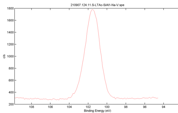
Figure 7.2.1. XPS Spectrograms for All Contributions in the Chabazite Samples S-LTA C -SiAl1-Na-V
