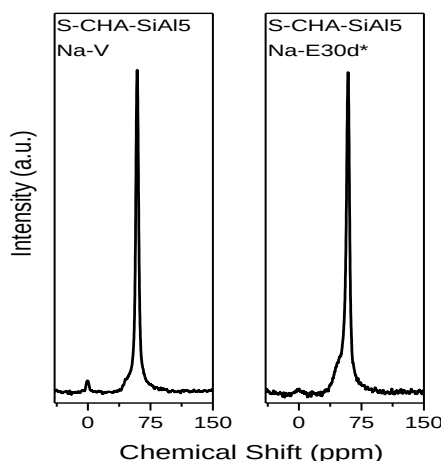
Figure 5.2.2. ^{27}\text{Al} NMR spectra for the sample S-CHAc-SiAl5-Na- (V, E30d*)
