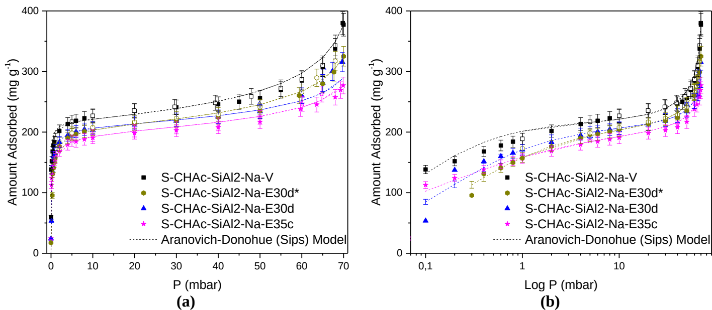
Figure 5.1.10. H 2 O Isotherms at 313 K in linear (a) and logarithmic (b) scales for sample (S-CHAc-SiAl 2 -Na): Pristine (V); Aged by PAP-1 (E35c) and by PAP-2 in a Single (E30d) and Dual (E30d*) Sample Port. The dashed curves stand for the Aranovich-Donohue model fits
