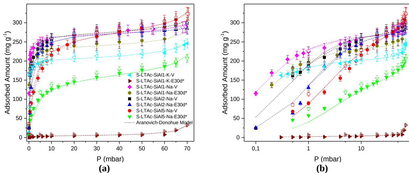
Figure 5.3.7. H 2 O Isotherms at 313 K in linear (a) and logarithmic (b) scales for the Samples S-LTAc-SiAl(1, 2, 5)- (Na, K) - (V, E30d*)
