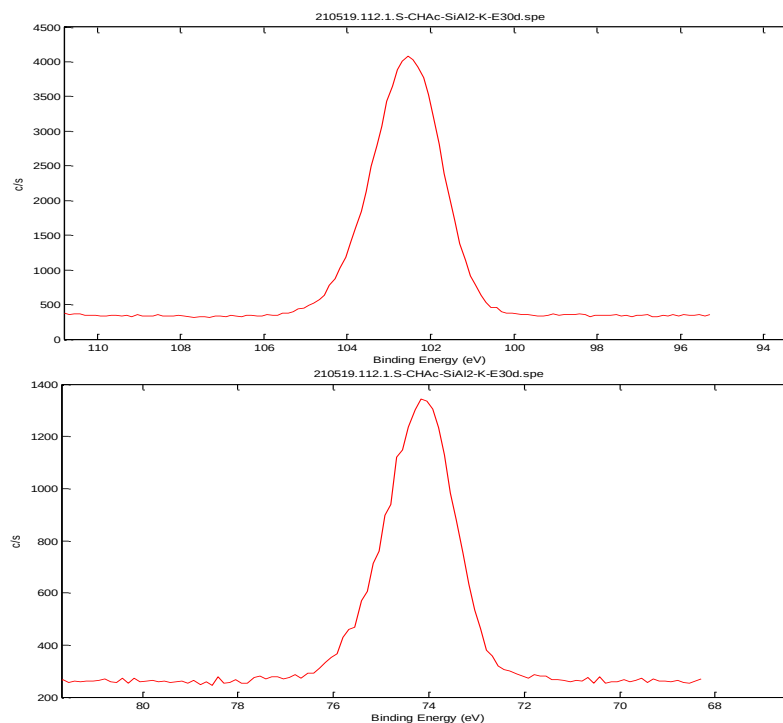
Figure 7.1.6. XPS Spectrograms for All Contributions in the Chabazite Samples S-CHAc-SiAl 2 -K-E30d*
