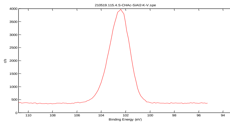
Figure 7.1.5. XPS Spectrograms for All Contributions in the Chabazite Samples S-CHAc-SiAl2-K-V
