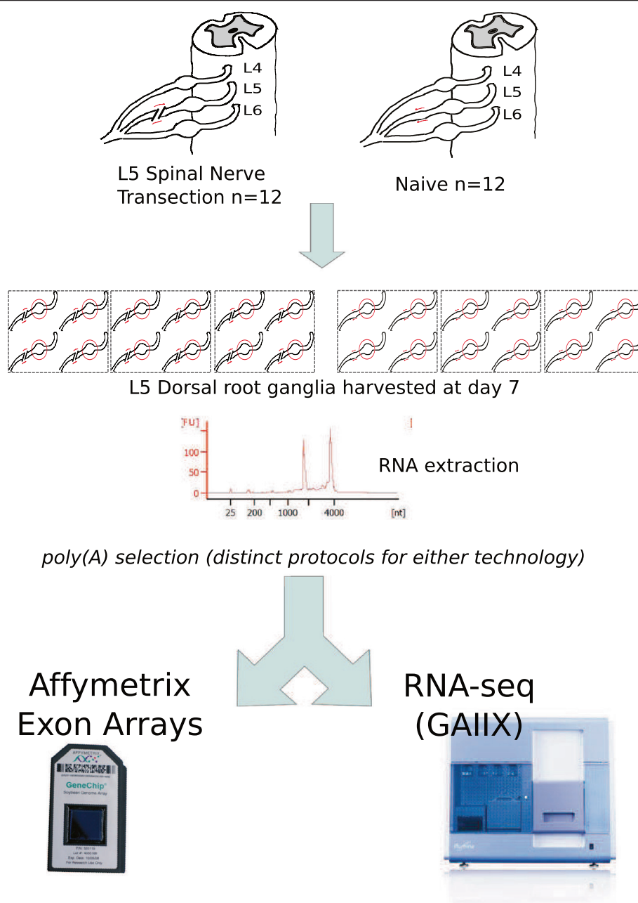
Figure 1 Experimental outline. L5-spinal nerve transection (SNT) was performed on twelve male Wistar rats. L5 DRG tissue was harvested 7 days after surgery and tissue from 4 animals was pooled for RNA extraction; naive tissue was used as control. Total RNA samples (n = 3 SNT, n = 3 naive) were divided into technical replicates used in parallel for microarray analysis (Affymetrix Rat Exon 1.0 ST arrays) and RNA-seq in the Illumina GALLX platform, in both cases following poly(A) enrichment.
