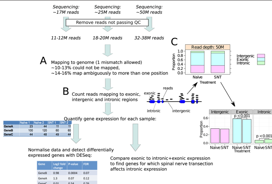
Figure 2 RNA-seq procedure and RNA-seq analysis pipeline. cDNA libraries were produced for each sample from poly(A) enriched RNA. These were sequenced to three distinct read depths (~17, ~25 and ~50 M reads/sample). Reads not passing the Illumina quality filter were discarded. A) Filtered reads were mapped to the genome, allowing a maximum of one mismatch between the sequence and the reference genome (Rn5); reads that could not be mapped to the reference genome or that could be mapped to more than one genomic location (ambiguous reads) were discarded. B) The remaining reads were mapped onto the genome and classified as exonic, intronic or intergenic as described in the Methods section. C) Stacked bar charts, showing the proportions of exonic, intronic and intergenic reads, at a 50 M read depth (the same pattern was obtained at 17 M and 25 M read depths). The unstacked barcharts show there is a significantly higher proportion of reads that align to intronic regions in SNT samples than in naive samples, and that the proportion of reads mapping to exonic regions is significantly higher in naive samples than in SNT samples. P-values were calculated using the overdispersed logistic regression test described in the Methods section. Evidence of a difference between SNT and naive was found for intergenic reads, however this did not retain significance following the Bonferroni correction for multiple testing. Following alignment, gene expression was quantified by counting the number of reads mapping to each gene. Read counts were normalised by, and differential gene expression analysis was performed using DESeq. The effect of reads mapping to intronic regions on differential gene expression was assessed by comparing exonic expression to exonic and intronic expression.
