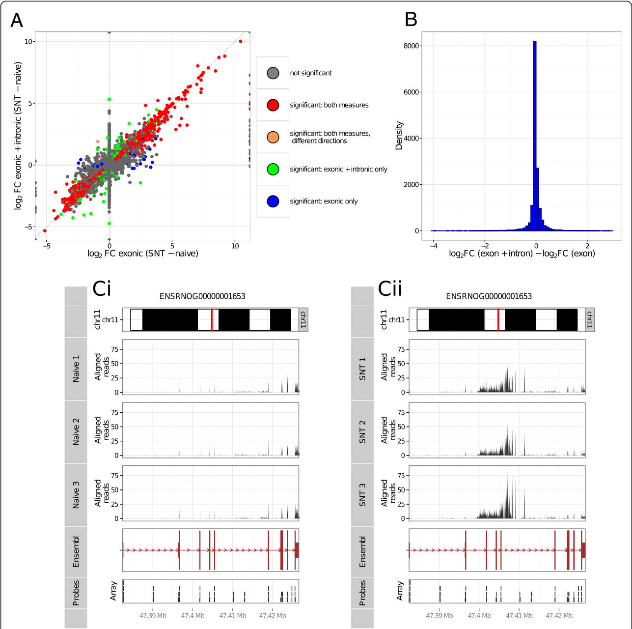
Figure 7 The effect of intronic expression on fold change calculation. A) Estimation of \log_2 FC considering exon reads only (x-axis) compared to FC calculating counting exon and intronic reads (y-axis). Red points represent genes called DE when using both counting schemes with the same direction of fold change, peach points represent the two genes that are called as DE with both schemes, but with opposite directions of fold change. Green points show genes called DE when considering exon reads only, but not when considering exon and intronic reads. Blue points show genes DE when considering exon and intronic reads but not when considering exon reads only. B) Distribution of the ratio of fold changes estimated by both methods. Calculated by subtracting the \log_2 FC values calculated using full gene expression from \log_2 FC calculated exon expression only. Ci, Cii) Genome graphs for gene St3gal6, showing intronic expression that is not proportional to exon expression, i.e. that is increased following SNT. The figure comprises a series of "tracks" for each gene, and its expression levels for SNT samples (Ci) and naive samples (Cii). The top tracks show the genomic coordinates of the gene on chromosome 11 (precise position marked in red). The middle histogram-like tracks show the positions of RNA-seq reads mapping to the genomic location of the gene. Below these tracks is a track showing the gene structure (exons are represented by boxes, introns are represented by arrowed lines, the direction of these arrows shows the direction of transcription). Bottom track shows the position of the microarray probes that map to the genomic location of the gene.
