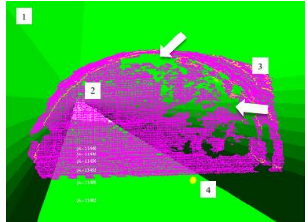
Figure 11: Snapshot of the TCS user interface. (1) Planned tunnel. (2) Mesh created from the scanned points. (3) Intersection of the planned tunnel and the mesh. The arrows point at areas where the scanned points were either lost or very noisy. (4) Position of the TCS system during the operation.
