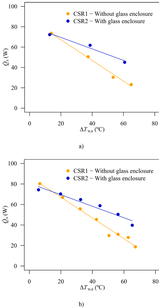
Fig. 8. Plots of standardised power of cookers CSR1 and CSR2 for the experiment 109B with clustering time interval of a) 10 min and b) 5 min.
