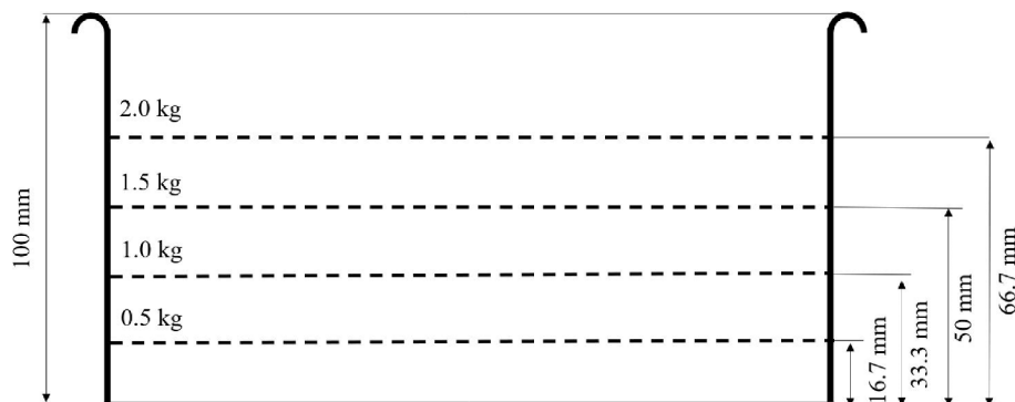
Fig. 6. Water line height h_w for different load levels.
