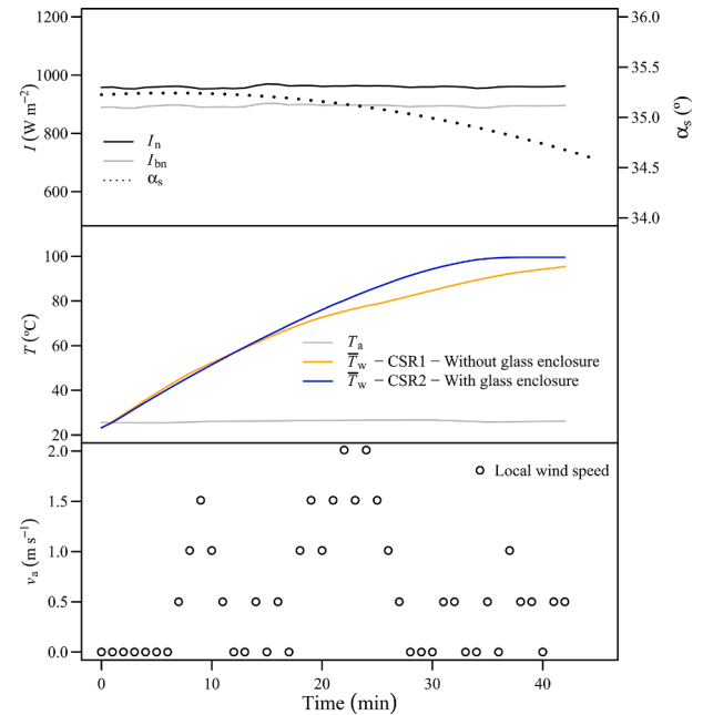
Fig. 7. Time series of several variables during test of cookers CSR1 and CSR2 in experiment 109B by using 0.5 kg of water.
