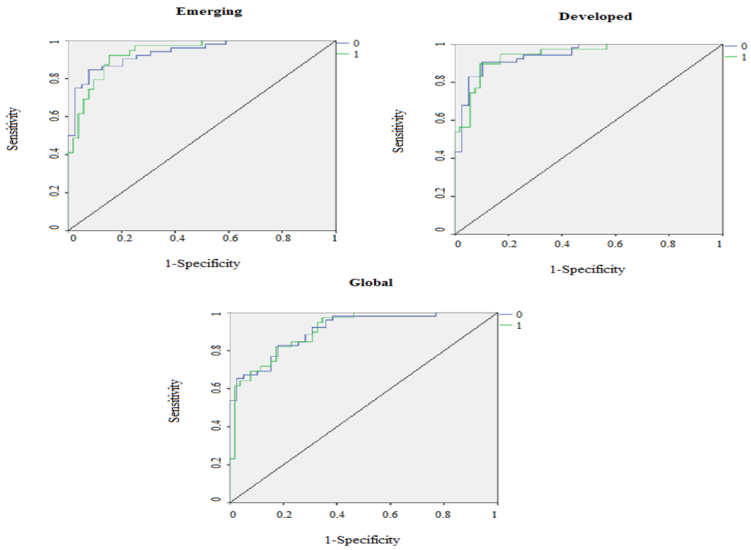
Figure 3. ROC curves of estimated models
