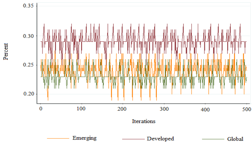
Figure 5. RMSE score in testing data for 500 iterations
