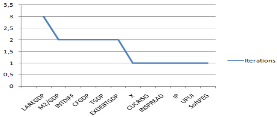
Figure 4. Number of repetitions of the significant variables
