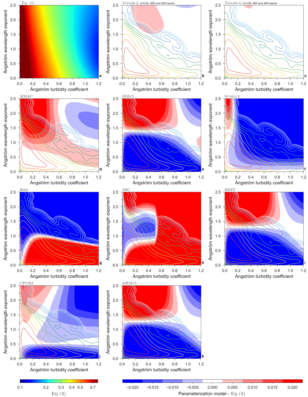
Figure S2: As Fig. 8 in the main paper but includes all models evaluated. The calculations with MRMV5 assume sea-level pressure.
