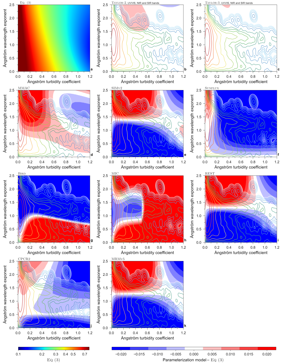
Figure S3: As Fig. 9 in the main paper but includes all models evaluated. The calculations with MRMV5 assume sea-level pressure.
