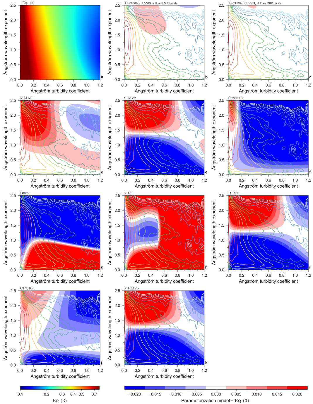
Figure S1: As Fig. 7 in the main paper but includes all models evaluated. The calculations with MRMV5 assume sea-level pressure.
