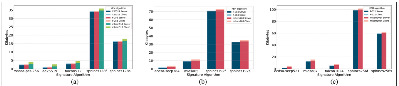
FIGURE 3. Data Transmission in Kilobytes During TLS handshake.
