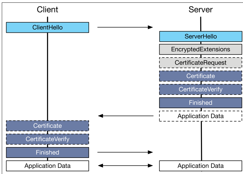
FIGURE 1. TLS 1.3 Message Flow (based on RFC 8446).
