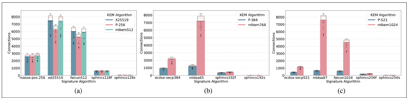
FIGURE 2. TLS Handshake connections during 10 seconds.
