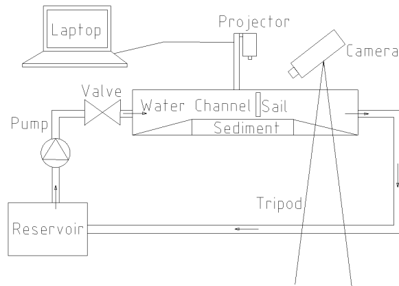
Figure 4.1: Sketch of the water channel.
