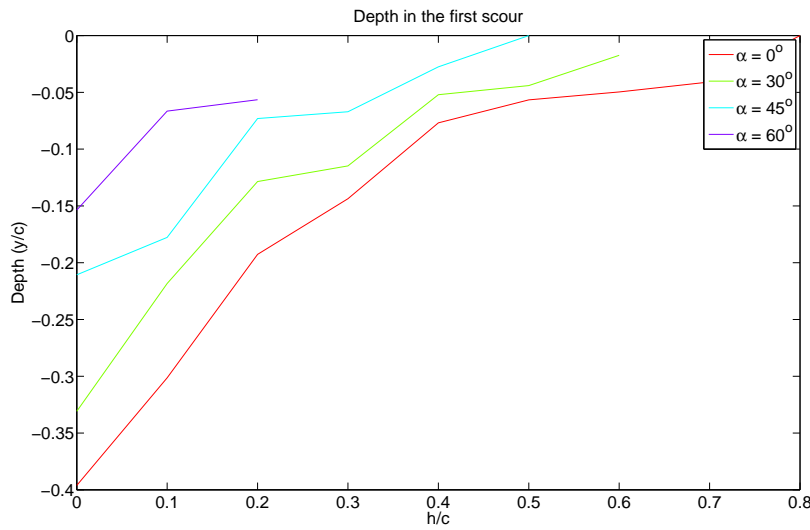
Figure 4.12: First scour depth for \alpha = 0^\circ, 30^\circ, 45^\circ and 60^\circ as a function of h .
