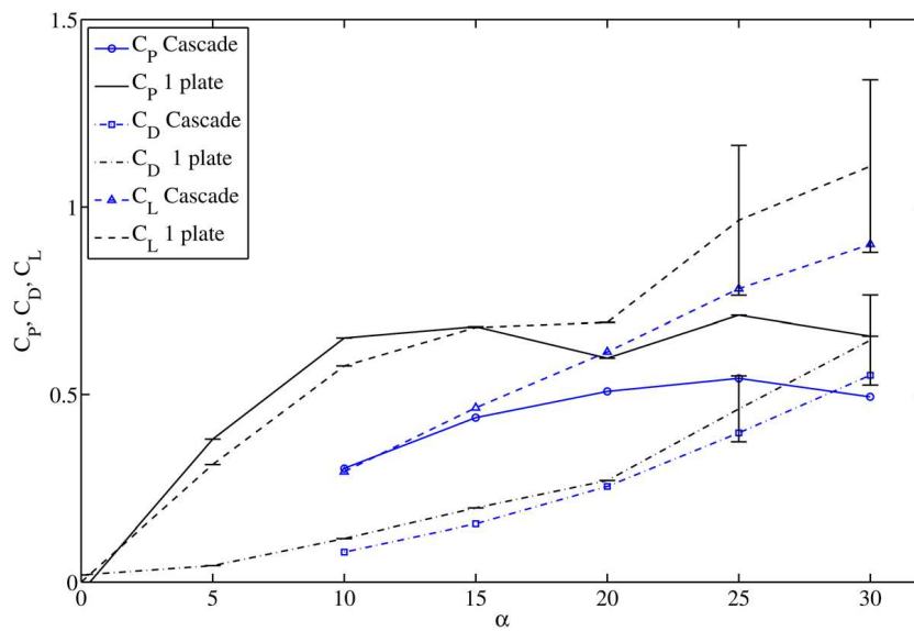
Figure 2.13: Comparison between C_P , C_L , and C_D vs. \alpha for an isolated plate and for a cascade with \sigma = 1 and \xi = 2.5
