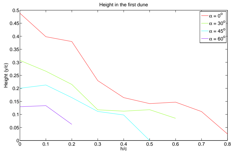
Figure 4.13: Height in the first scour for \alpha = 0^\circ , 30^\circ , 45^\circ and 60^\circ as a function of h .
