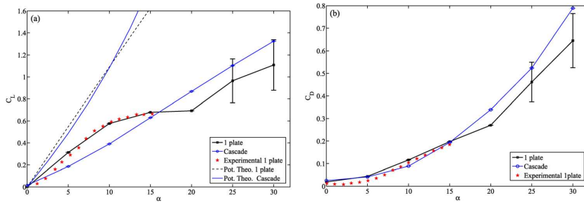
Figure 2.9: Comparison between C_L (a) and C_D (b) vs. \alpha for an isolated plate and for a cascade with \sigma = 1 and \xi = 1 ( sAR=3 , Re_W = 810^4 ). The error bars indicate the amplitude of the temporal oscillations around their mean values due to the oscillatory wake behind an isolated flat plate. The experimental results for a single plate by Pelletier & Mueller (2000) are included. Also included in (a) for reference sake is the 2D potential flow result C_L = 2\pi \sin \alpha \sin a for a single plate and the corresponding potential result for a cascade of flat plates Weing (1964)
