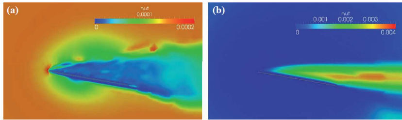
Figure 2.3: Contours of the computed eddy viscosity \nu_t on a portion of the middle plane z = 1.5c for the 3D flow around a flat plate with sAR = 3 , Re_W = 8 \times 10^4 and \alpha = 10^\circ when the RNG -k - \epsilon and the SST -k - \omega turbulence models are used. In particular, (a) corresponds to case 2 in Table I and (b) to case 6.
