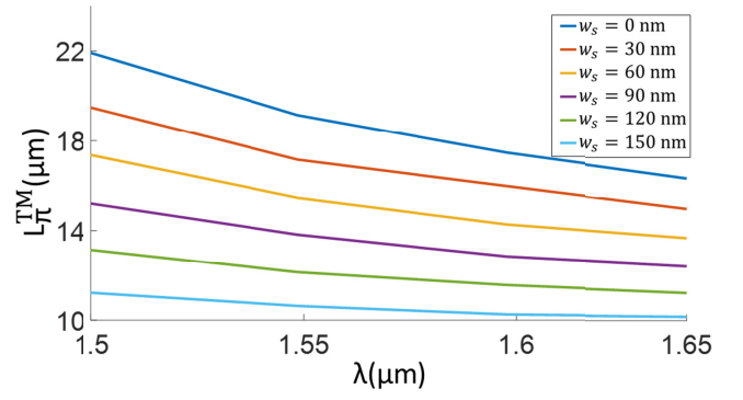
Fig. 4. Coupling length for TM polarization for the tilted SWG directional couplers with different silicon strip widths.
