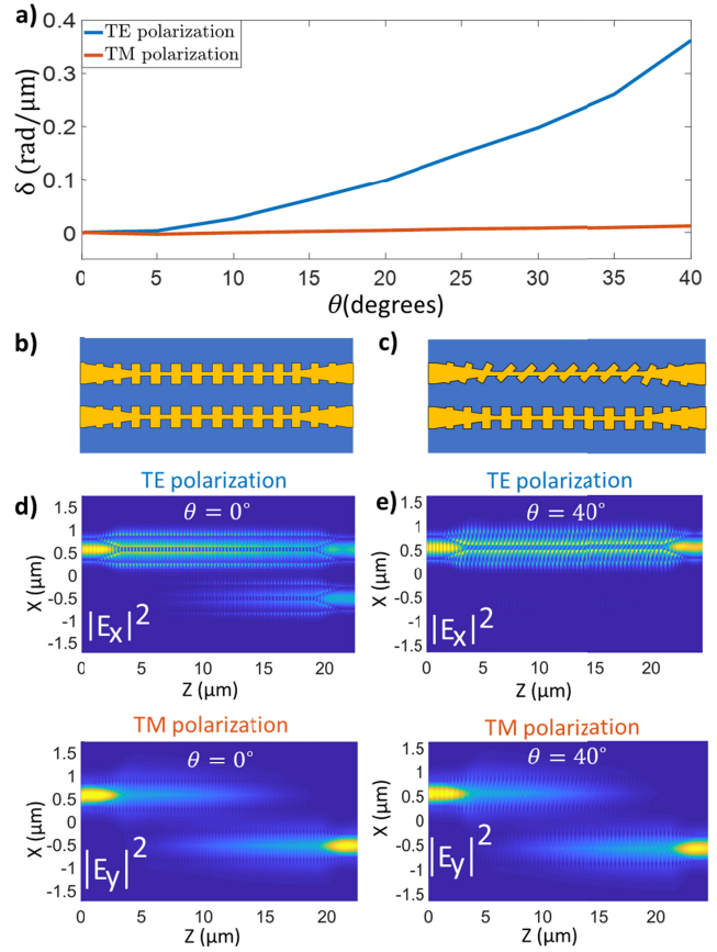
Fig. 2. (a) Detuning TE and TM phase matching conditions between the upper and lower waveguides with respect to the tilt angle. (b), (c) Schematic representation of the proposed directional coupler for a tilt angle of (b) \theta = 0^\circ and (c) \theta = 40^\circ . (d), (e) 3D-FDTD simulations of the squared magnitude of the main component of the propagating electric field for TE and TM polarization for a tilt angle of (d) \theta = 0^\circ and (e) \theta = 40^\circ .
