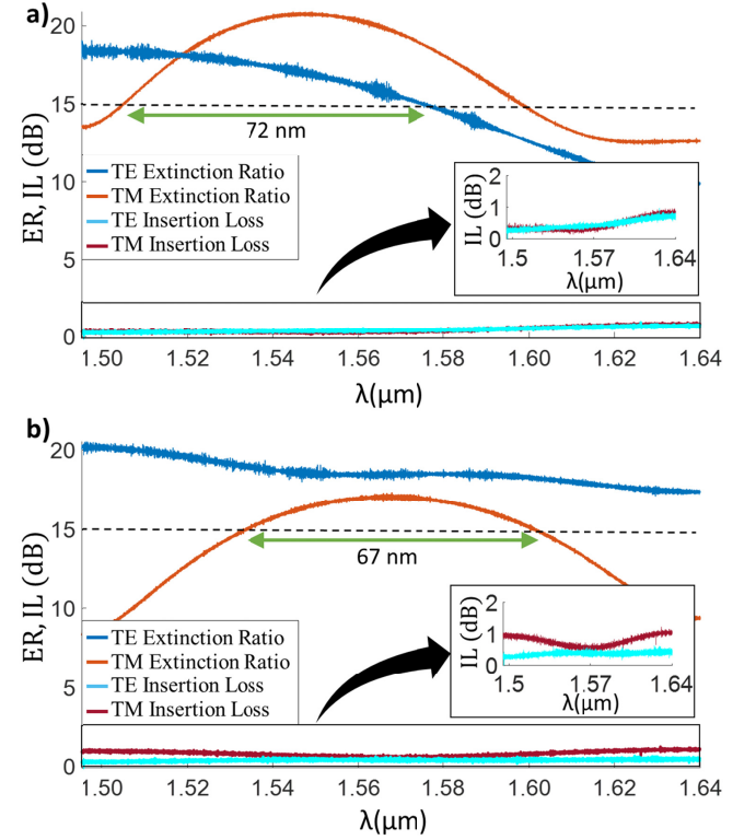
Fig. 5. (a) Measured extinction ratio and insertion loss of the nominal device. The IL is below 1 dB and the ER is better than 15 dB in bandwidth of 72 nm. (b) Measured extinction ratio and insertion loss for a device with a duty cycle increased 10%. The IL are <1 dB and the extinction ratio is >15 dB in a bandwidth of 67 nm.
