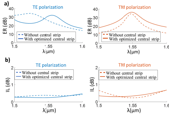
Fig. 3. (a) Extinction ratio, for both polarizations, of the tilted SWG directional coupler with and without the central silicon strip. (b) Insertion loss, for both polarizations, of the tilted SWG directional coupler with and without the central silicon strip.
