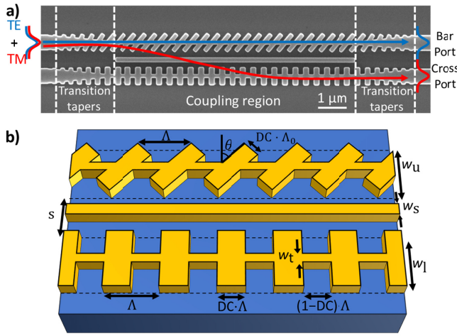
Fig. 1. (a) Scanning electron image (SEM) of the directional coupler based polarization beam splitter (before SiO 2 cladding deposition). The tilted SWG segments in the top waveguide break the structural symmetry for the TE polarized mode, which remains in this waveguide. The TM polarized mode is unaffected by the tilt and couples to the cross port. (b) Schematic of the coupling region of the polarization beam splitter (the cladding is not shown for the sake of clarity).
