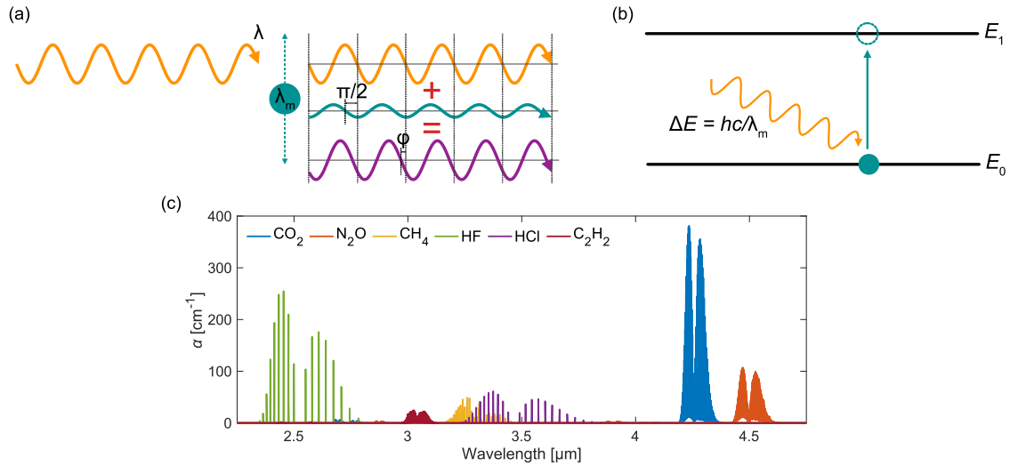
Figure 1.3: (a) Schematic representation of the fundamental origin of refraction. (b) Schematic representation of the absorption of a photon with energy \Delta E . (c) Light absorption spectra of different gases, represented in terms of the absorption coefficient ( \alpha ). All data are extracted from [46].
