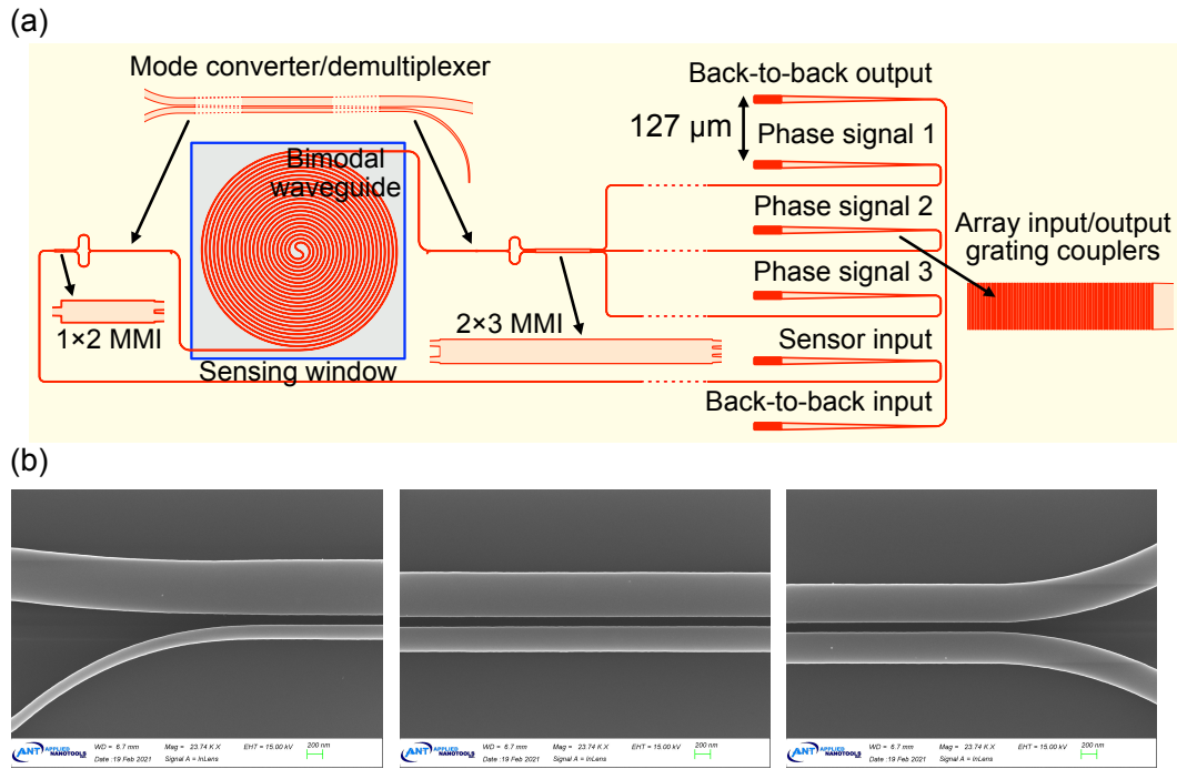
Figure 5.5: (a) Mask layout for the first-generation sensor, designed for ANT's SOI platform. (b) SEM images of the mode converter, based on a counter-tapered coupler.
