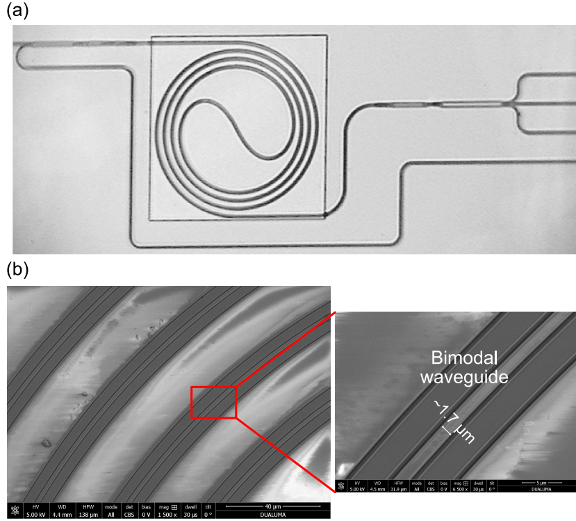
Figure 5.13: (a) Optical microscope picture of the bimodal sensor. (b) SEM images of the bimodal sensing waveguides. A waveguide width around 1.7 \mu\text{m} was measured.
