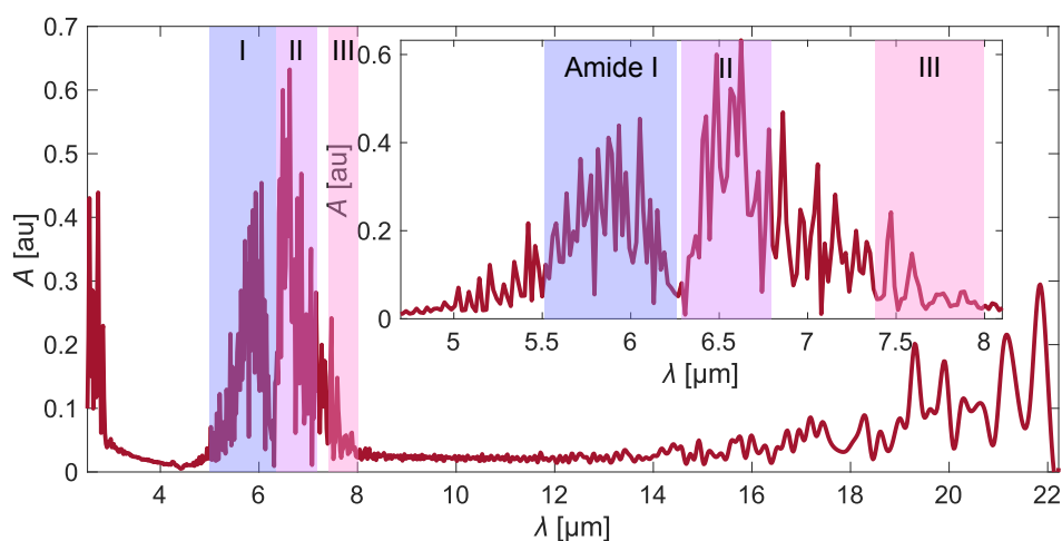
Figure 6.1: Water absorbance spectrum in the mid-infrared. The inset shows the high-absorption region between 5 and 8 \mu\text{m} . Data extracted from [139].
