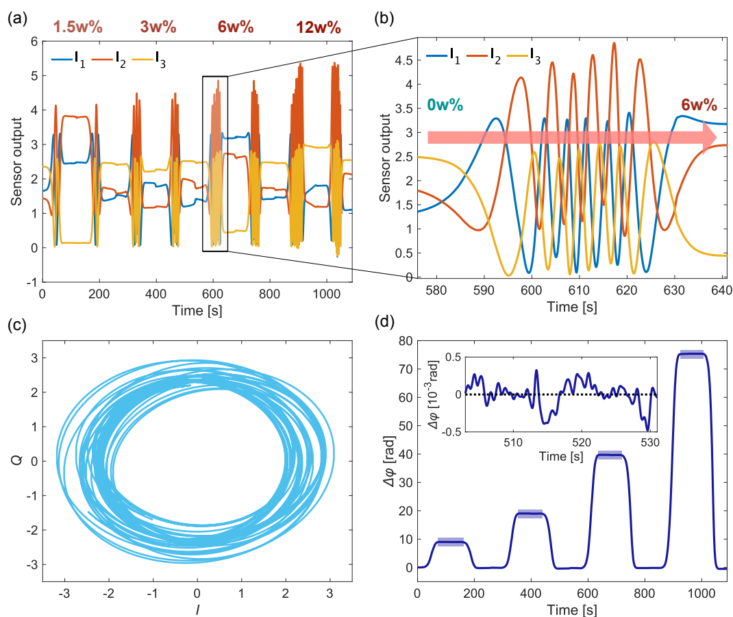
Figure 5.15: (a) Sensor output during a bulk sensing experiment with different NaCl solutions. (b) Close-up of the interferometric signals during the transition from the buffer to a 6w% NaCl sample. (c) Generated complex signal, from which (d) the phase shift is extracted. The areas employed in the calculation of saturation values are highlighted. A representative noise fragment is shown in the inset.
