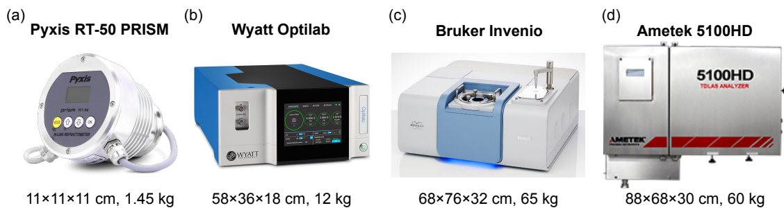
Figure 1.5: Commercial optical refractive index and absorption benchtop sensors. (a) Pyxis RT-50 PRISM prism-based refractometer [51]. (b) Wyatt Optilab interferometric refractometer [52]. (c) Bruker Invenio FTIR absorption spectrometer [53]. (d) Ametek 5100HD TDLAS absorption spectrometer [54].
