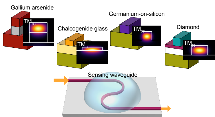
Figure 1.7: Overview of the main contributions of this thesis, including 3D illustrations (not to scale), simulated mode profiles, SEM and optical microscope images and results. The results shown for Chapters 4 and 5 include experimental demonstrations, while those from Chapter 6 are theoretical.
