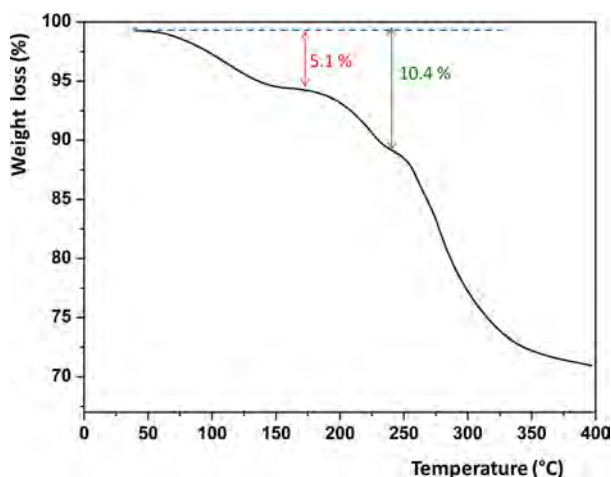
Figure 3. TGA data for \text{Mg-BPMGLY}\cdot 2\text{W} . Two weight-loss steps due to water release are highlighted.
