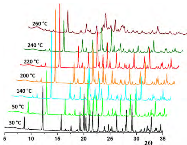
Figure 4. Thermodiffractometric study for \text{Mg-BPMGLY}\cdot 2\text{W} .
