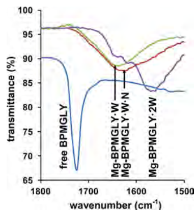
Figure 2. FT-IR spectra of the free ligand \text{BPMGLY} , \text{Mg-BPMGLY}\cdot 2\text{W} , \text{Mg-BPMGLY}\cdot\text{W} , and \text{Mg-BPMGLY}\cdot\text{W}\cdot\text{N} in the carboxylate asymmetric stretch region.
