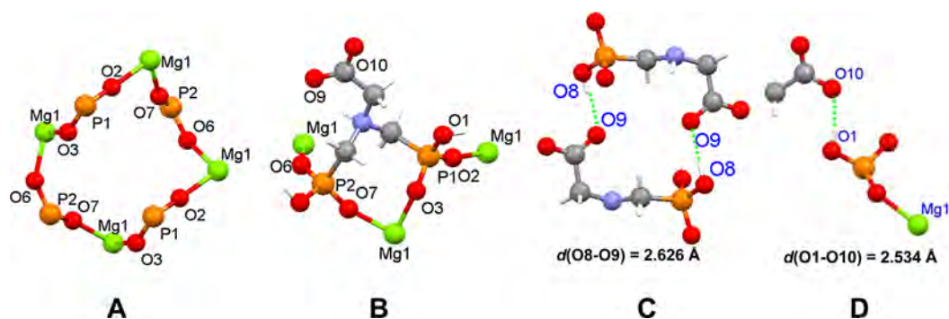
Figure 5. Mg–O(phosphonate) bonds forming 16-membered rings (A), coordination mode of the ligand BPMGLY in Mg–BPMGLY·2W (B), dyad of C–O 9 ⋯H–O 8 –P hydrogen bonds holding the layers together (C), and single C–O 10 ⋯H–O 1 –P hydrogen bond (D).
