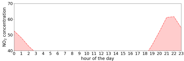
Fig. 6: The shaded area represents the \text{NO}_2 concentration over the EU threshold during weekends.
