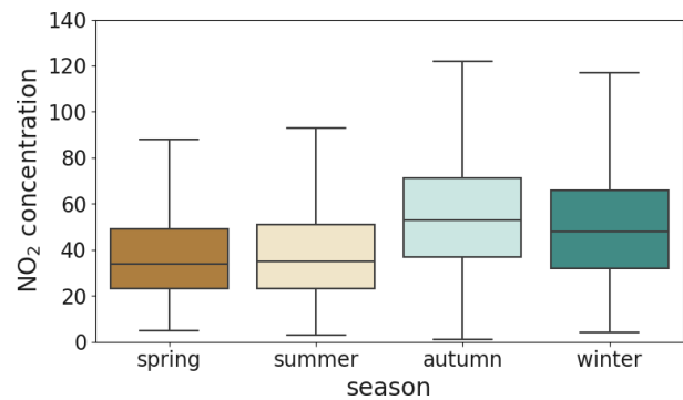
Fig. 3: \text{NO}_2 concentration per hour for each season.
