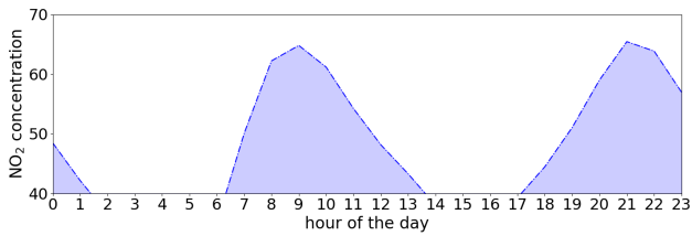
Fig. 5: The shaded area represents the \text{NO}_2 concentration over the EU threshold during working days.
