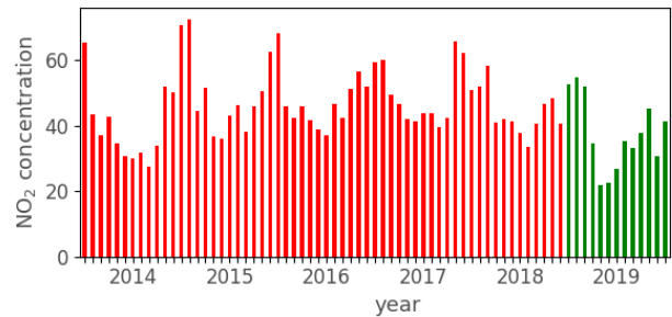
Fig. 2: Mean \text{NO}_2 concentration per month.
