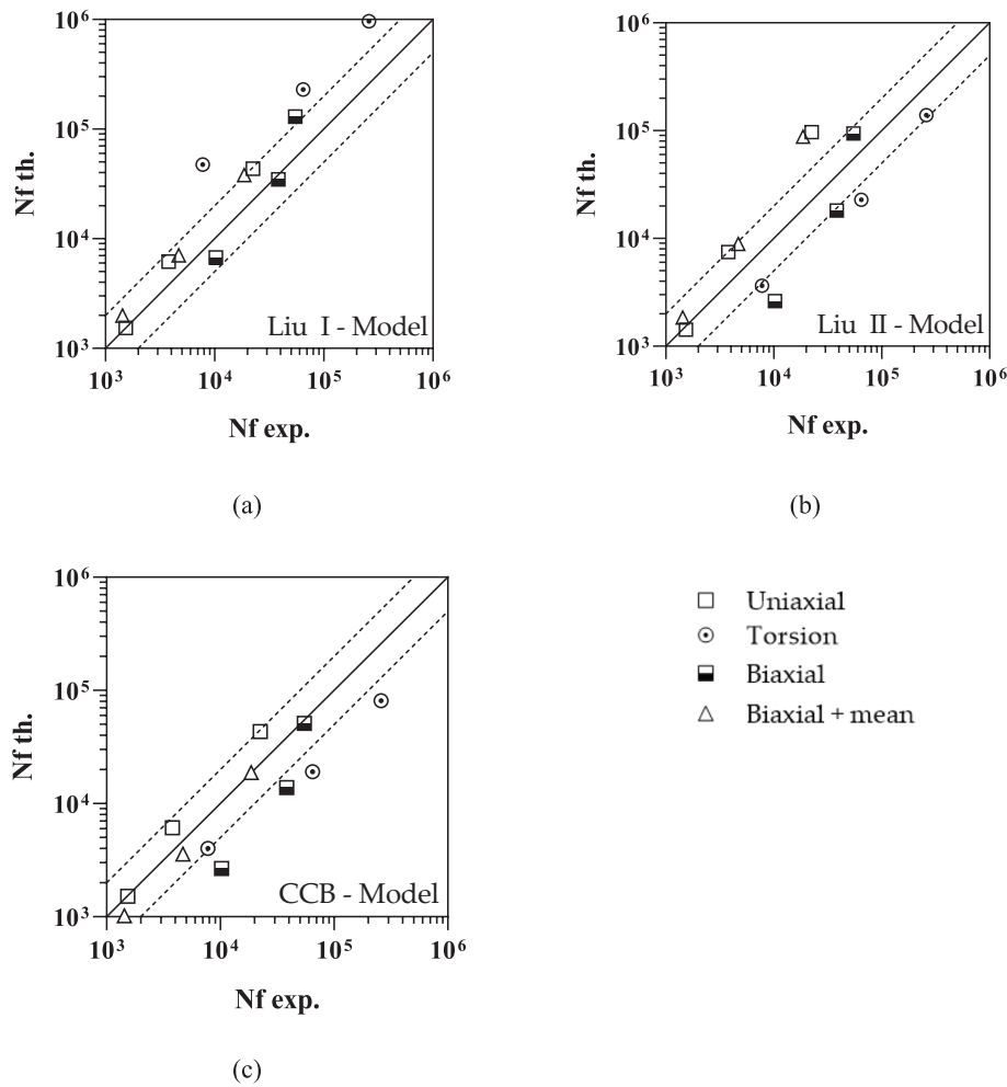
Fig. 7. Fatigue life estimation on AM 18Ni300 steel based of Liu I, Liu II and CCB methods against the experimental life.
