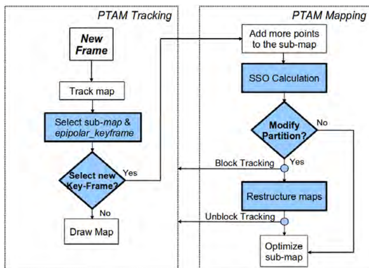
Figure 4.3: Tracking and mapping threads of PTAM. Blue boxes correspond to the embedded stages to perform the map partitioning.
