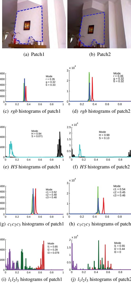
Figure 3.4: Two patches of the same plane extracted from different views with their histograms in the colour spaces rgb , HS , c_1c_2c_3 and l_1l_2l_3 below. We can appreciate that the histograms in rgb and c_1c_2c_3 exhibit more clearly unimodal, and more stable distributions.
