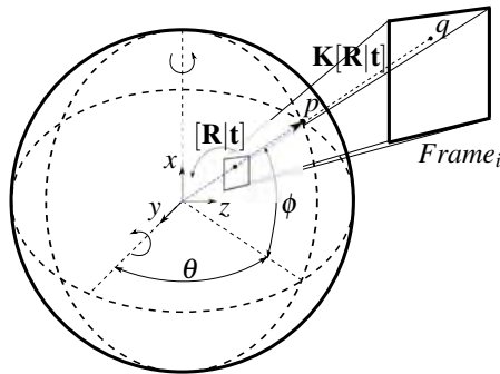
Figure 5.3: Spherical image construction
