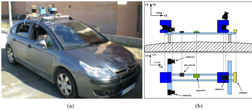
Figure 2.14: A semi-autonomous car which incorporates several laser rangefinders at different orientations. b) Scheme of the sensors.
