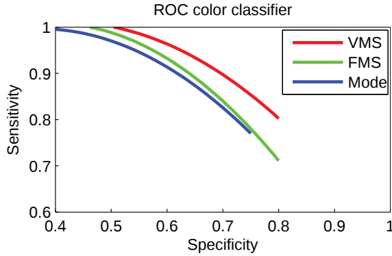
Figure 3.6: ROC curves (sensitivity vs. specificity) of the colour constraints as binary classifier.
