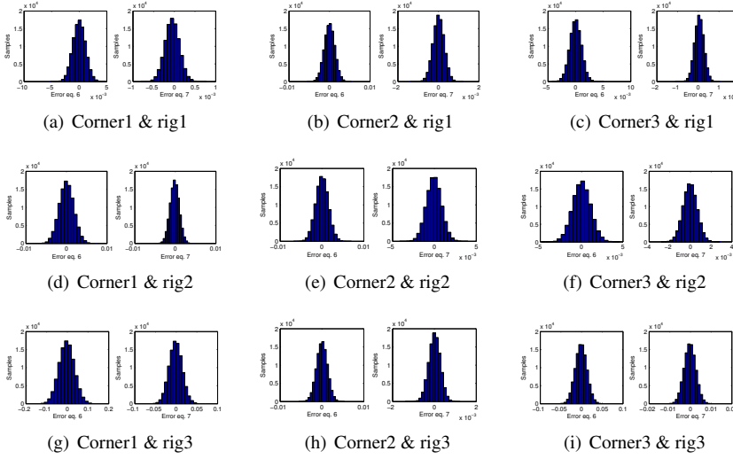
Figure 2.6: Monte Carlo simulation of a corner observation at three different orientations (a different corner is shown in each column) with three different rigs of two LRFs (a different rig is shown in each row). The planarity and perpendicularity errors are shown at the left and right of each graph, respectively.
