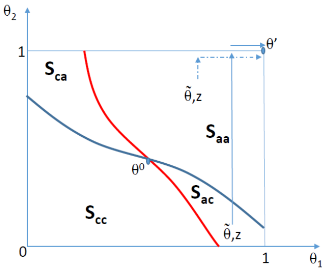
Picture 3.a. Case 3: \tilde{\theta} \in S_{ac} \cup S_{aa} \cup S^0
