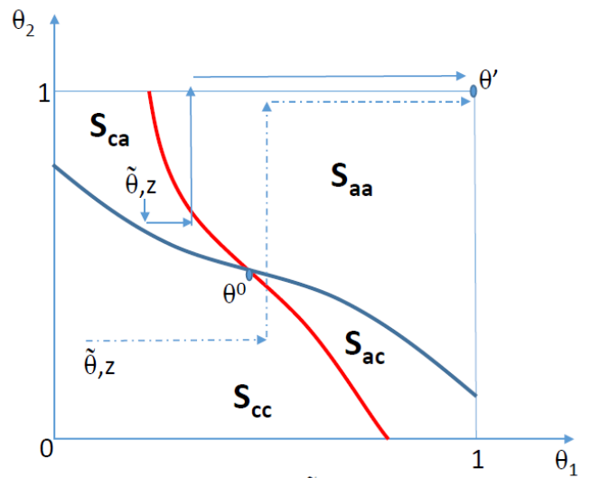
Picture 3.b. Case 4: \tilde{\theta} \in S_{ca} \cup S_{cc}
