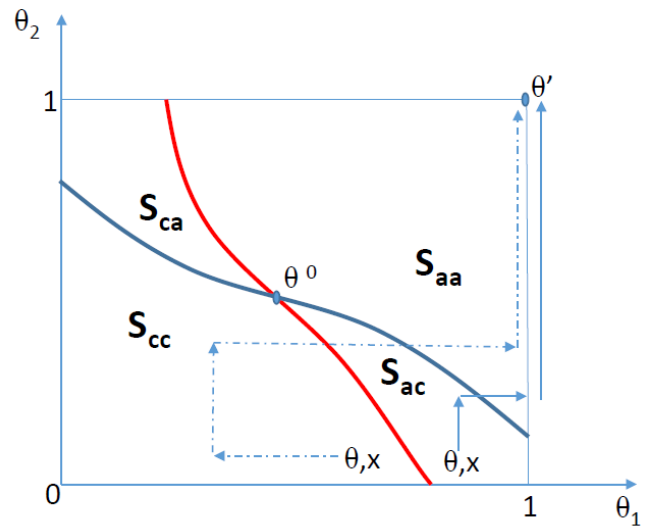
Picture 2.b. Case 2: \theta \in S_{ac} \cup S_{cc}
