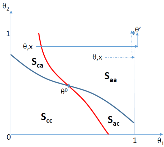
Picture 2.a. Case 1: \theta \in S_{ca} \cup S_{aa} \cup S^0
