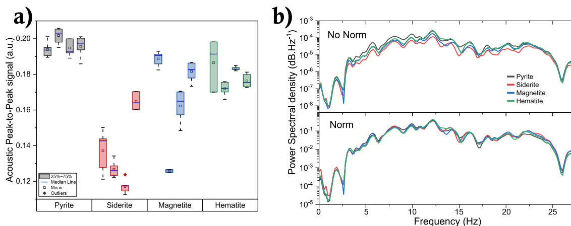
Fig. 3. a) Boxplot representing the average amplitude of the laser-induced acoustic signal for each homologue of the four different mineral phases. b) Non-normalized frequency domain power spectra for the mineral phases under study.
