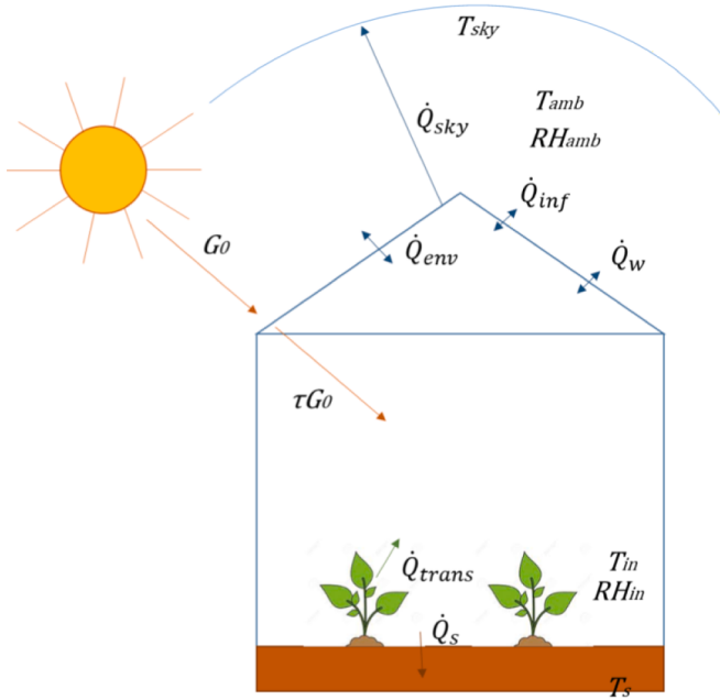
Fig. 2. Main thermal loads involved in the greenhouse energy balance.
