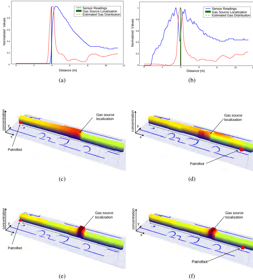
Figure 3.25: Snapshots of the maps generated in the 1D gas distribution mapping experiment at the middle and end of the robot path (left/right column, respectively), for a robot speed of 0.4\text{m/s} . Top row sub-figures illustrate a comparison between the normalized sensor readings and the gas distribution estimated here. The middle and bottom row sub-figures show a 3D reconstruction of the maps generated with the raw MOX readings (middle row), or the estimation provided by the proposed model (bottom row).
