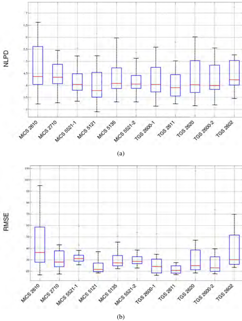
Figure 4.8: NLPD and RMSE box-plot for the case of one-sensor GP calibration with logarithmic transformation. For both indicators, as lower the value the better the calibration. On each box, the central red mark is the median, the edges of the box are the 25th and 75th percentiles, the whiskers extend to the most extreme data points not considering outliers, and outliers are plotted individually as red crosses.
