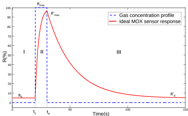
Figure 3.18: Ideal response of an MOX sensor (solid red line) when excited with a step gas concentration (dashed blue line). The curve shows the three phases of a measurement: (I) baseline, (II) gas measurement, and (III) recovery phase.
