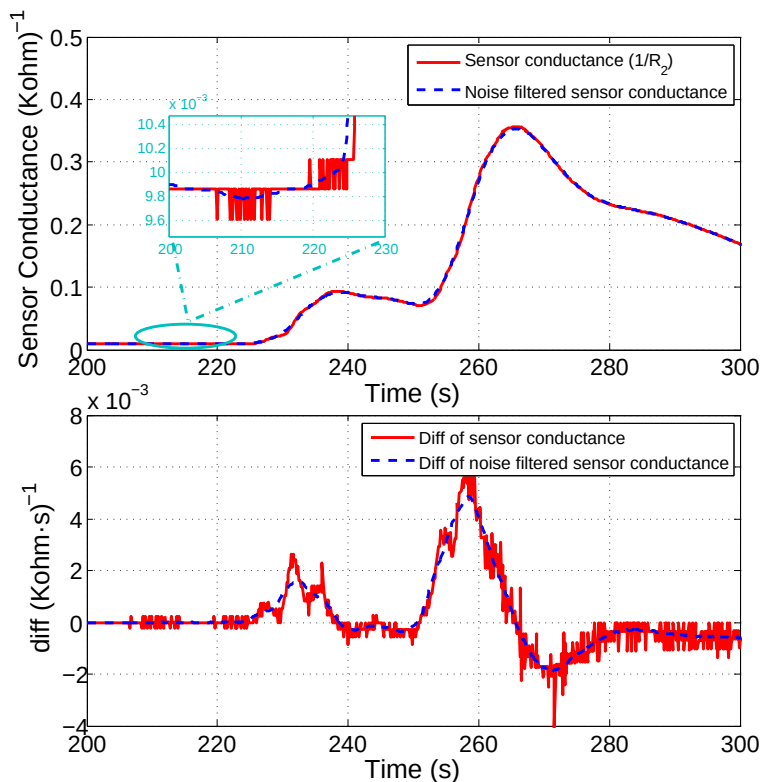
Figure 3.20: Noisy sensor conductance readings and its derivative (solid red line), and the corresponding filtered versions (dashed blue line).
